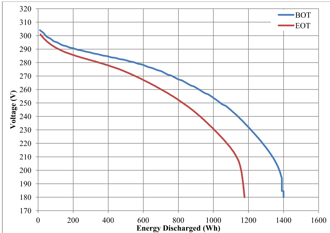
Figure 1. Voltage versus energy discharged during the static capacity test
