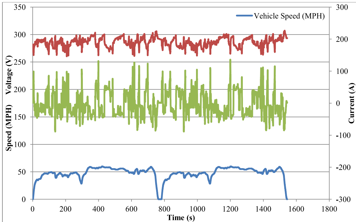
Figure 12. Battery pack current, voltage, and vehicle speed for a HWFET dynamometer drive-cycle
