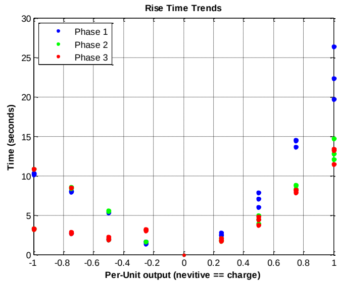
Figure 8 Rise Time
