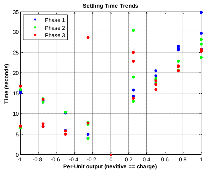
Figure 9 Settling Time
