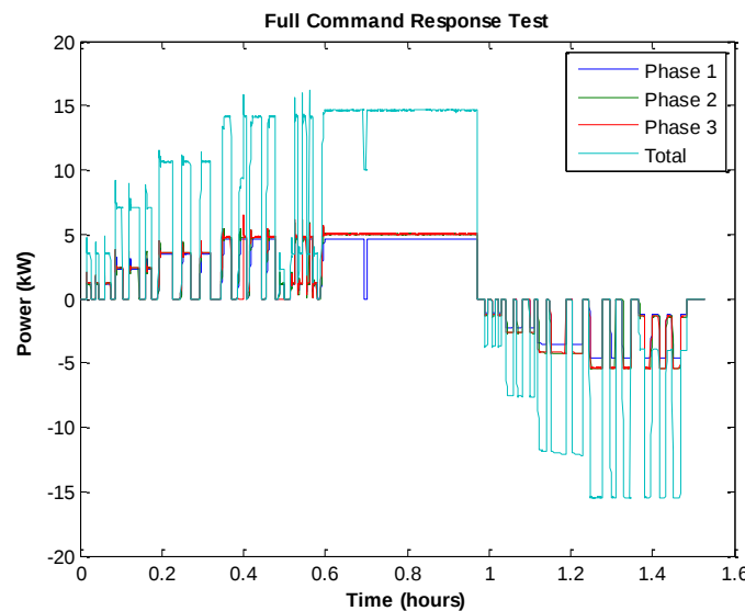
Figure 3 Command Response Test Results
