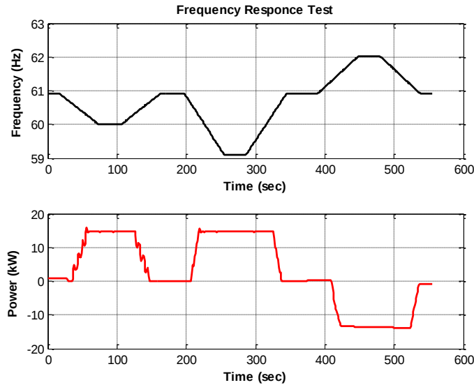
Figure 5 Frequency Response Test Results
