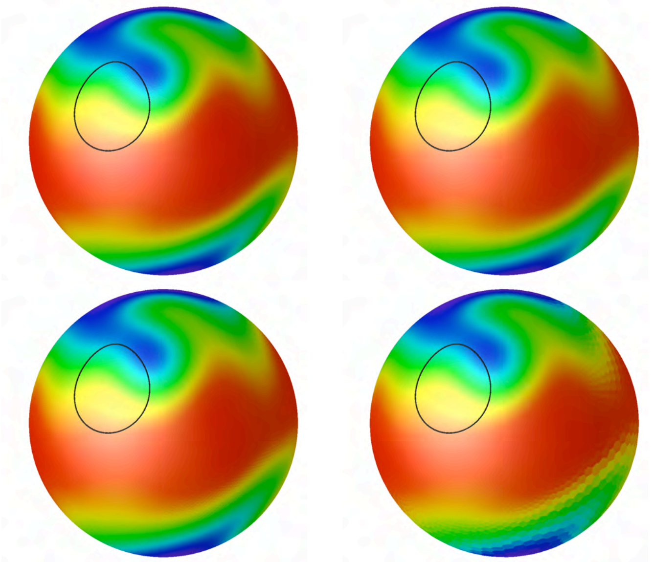
FIG. 4. The fluid height, h_i + b_i , at day 15 for SWTC5. Starting at the upper left and moving clockwise shows results from the X1, X2, X16 and X4 meshes using 40962 cells. The black oval denotes the location of the orography. The figures are generated by filling each Voronoi cells with a single color, i.e. there is no interpolation due to rendering. This allows the far-field grid resolution to be seen in the X4 and X16 simulations.
