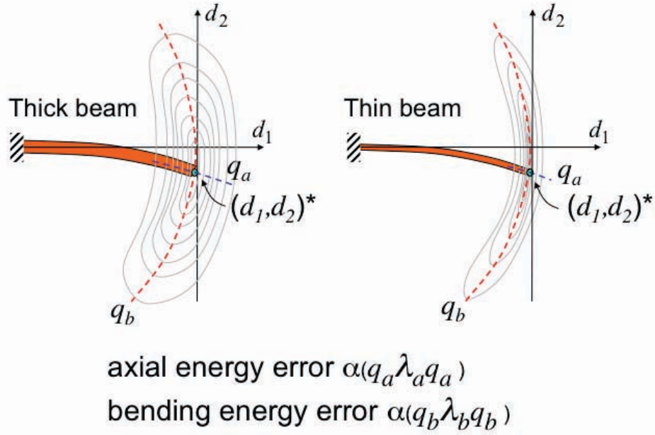
Figure 13.4: Energy error example: Energy error contours for two beams.
