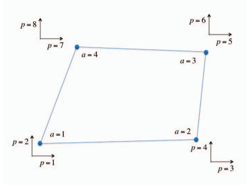
Figure 10.4: Element (local) degrees of freedom for a sample finite element.
