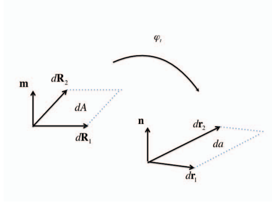
Figure 7.1: Notation for derivation of Nanson's formula
