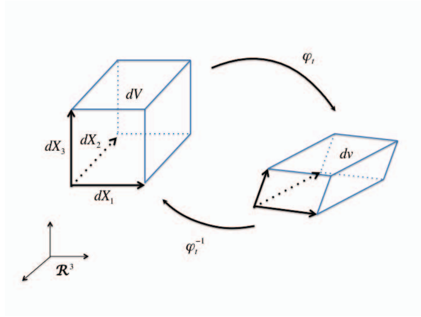
Figure 5.1: Deformation of a volume element as described by the configuration mapping \varphi_t .
