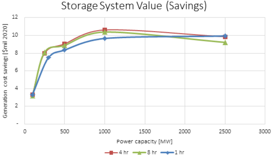
Figure 3: Additional Storage System Sensitivity Results
