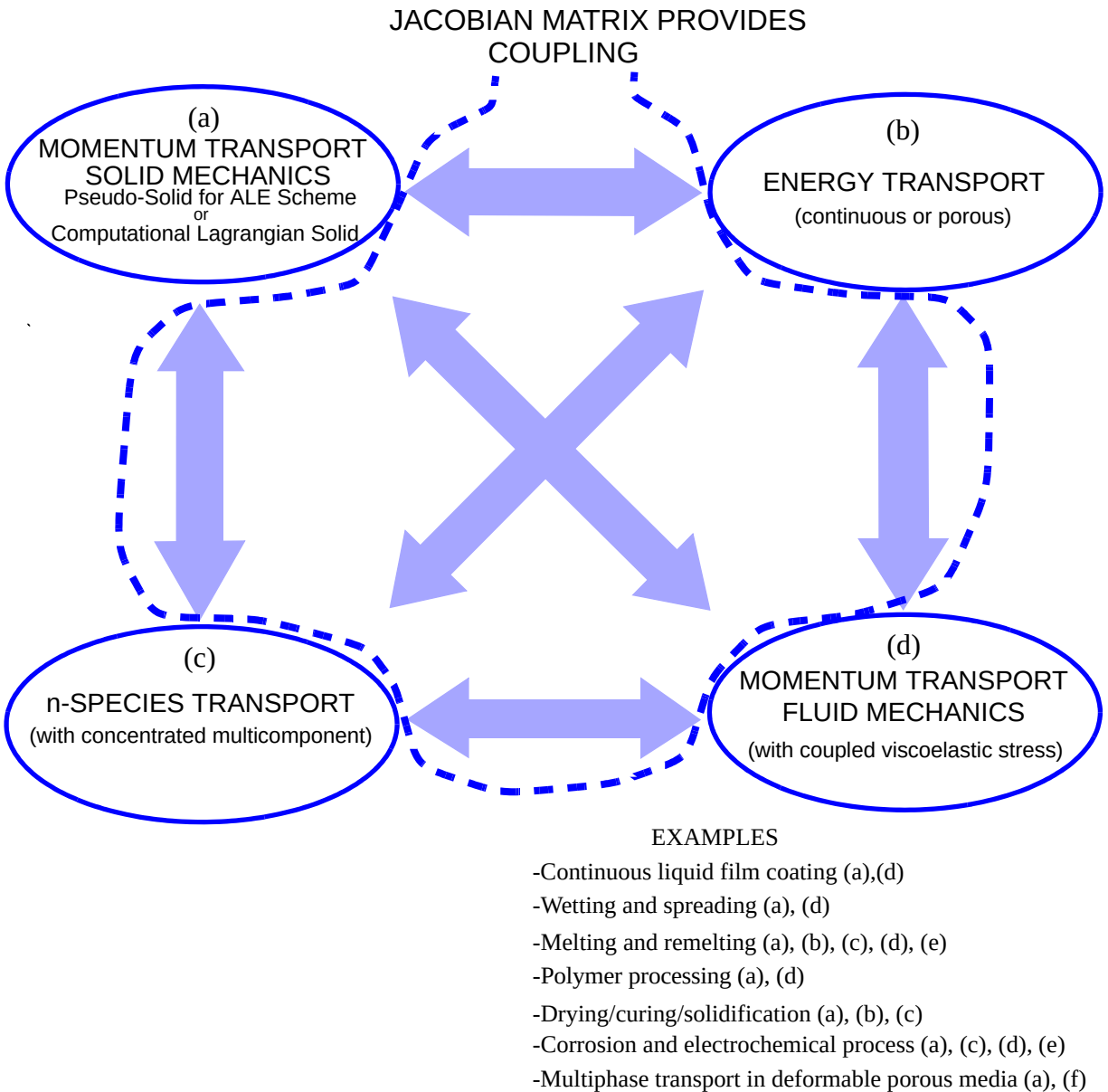
Figure 1. Main physics modules of Goma , their coupling and examples of potential applications.
