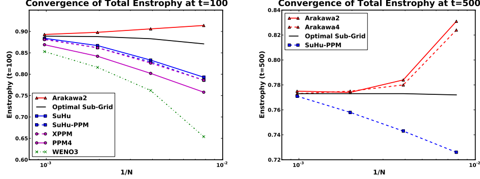
FIG. 4.6. Convergence of the total enstrophy at time t = 100 (left) and time t = 500 (right) vs. 1/N , for grid sizes N = 128, 256, 512, 1024 , for the high Reynolds number case. Also plotted are the solutions from an optimal sub-grid model.
