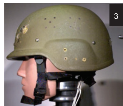
Figure 1) Proton radiograph of a jet penetration (penetration direction bottom to top). Figure 2) Optical photograph of an armor material cross section acquired after impact of a kinetic energy projectile (impact direction top to bottom). Figure 3) Optical photograph of a composite material helmet just prior to a kinetic energy projectile impact (projectile moving from right to left).
