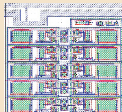
Ten-frame imager pixel layout; the 40-μm x 40-μm pixel shown above, in 180-nm CMOS process allows 10 signal storage capacitors per pixel.
