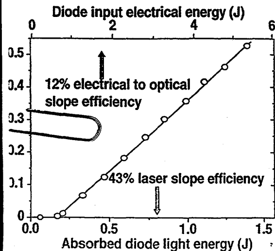
Fig.6: Laser performance of a laser diode array pumped Yb:S-FAP oscillator.
