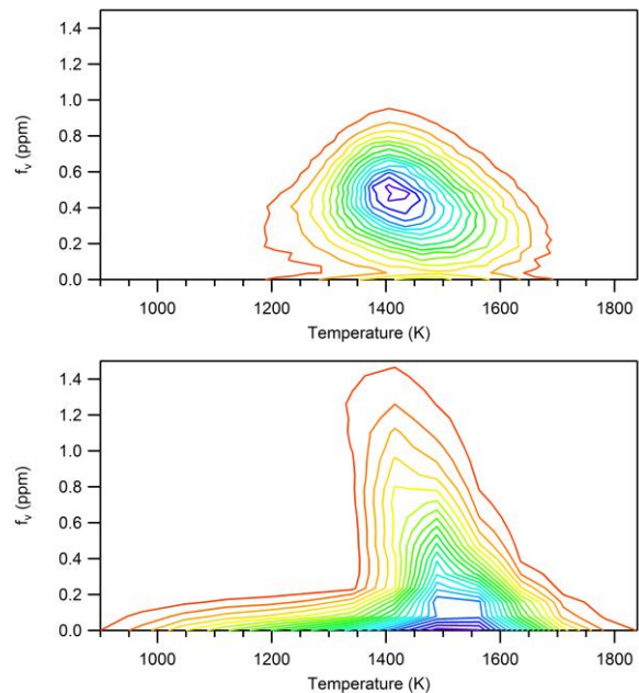
Fig. 7. Joint pdfs of soot volume fraction and soot temperature at a height of 44.8 cm ( z/d = 140 ) (top) and at a height of 64.0 cm ( z/d = 200 ) (bottom) along the centerline of the ethylene jet flame.
