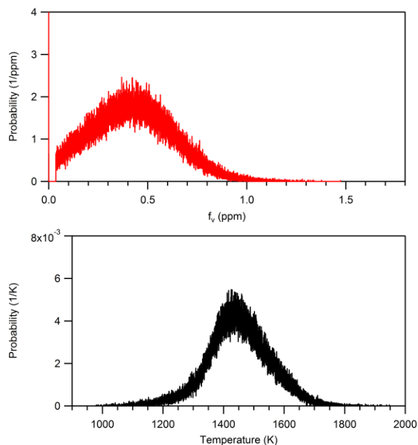
Fig. 5. Soot volume fraction pdf (top) and soot temperature pdf (bottom) at a height of 44.8 cm ( z/d = 140 ) along the centerline of the ethylene jet flame..
