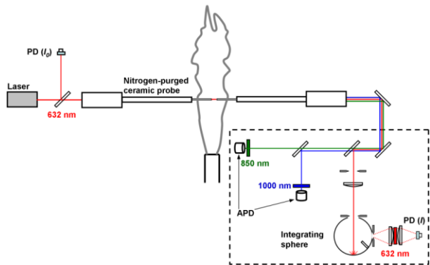
Fig. 1. Schematic of diagnostic configuration used to perform 3-line measurements of soot temperature/concentration statistics in the turbulent jet flames.
