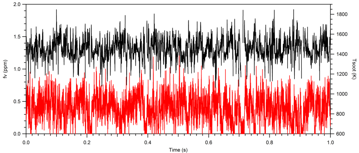
Fig. 4. Deduced soot volume fraction and soot temperature time records for the raw data record shown in Fig. 3. The volume fraction is shown in red, corresponding to the left axis, and the soot temperature is in black and corresponds to the right axis.
