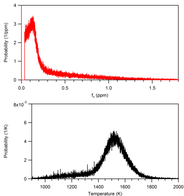
Fig. 6. Soot volume fraction pdf (top) and soot temperature pdf (bottom) at a height of 64.0 cm ( z/d = 200 ) along the centerline of the ethylene jet flame.
