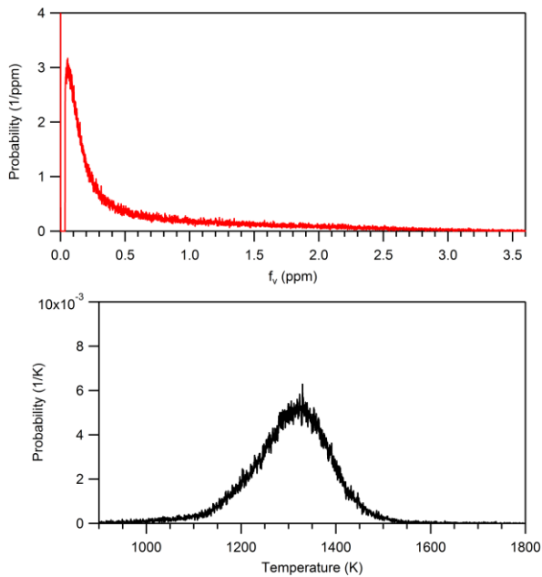
Fig. 9. Soot volume fraction pdf (top) and soot temperature pdf (bottom) at a height of 68.75 cm ( z/d = 275 ) along the centerline of the JP-8 surrogate jet flame.
