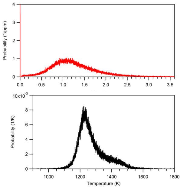
Fig. 8. Soot volume fraction pdf (top) and soot temperature pdf (bottom) at a height of 37.5 cm ( z/d = 150 ) along the centerline of the JP-8 surrogate jet flame.
