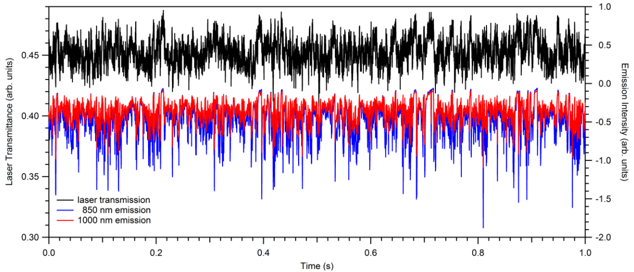
Fig. 3. Example time record of laser transmittance and soot emission for a height of 44.8 cm ( z/d = 140 ) along the centerline of the ethylene jet flame.
