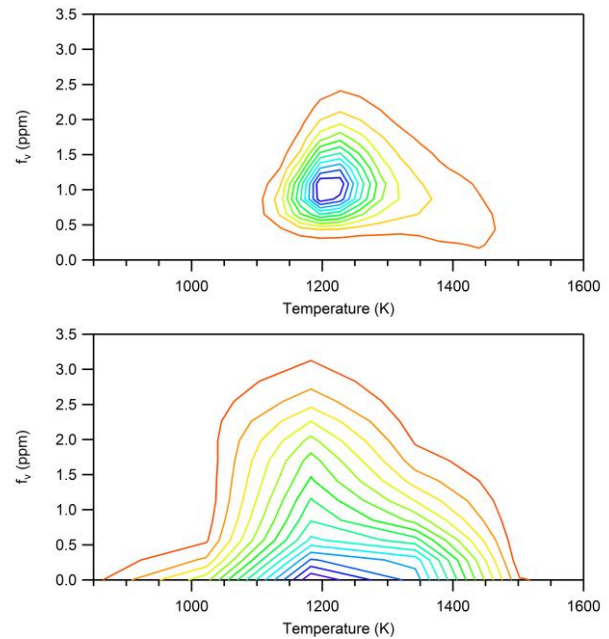
Fig. 10. Joint pdfs of soot volume fraction and soot temperature at a height of 37.5 cm ( z/d = 150 ) (top) and at a height of 68.75 cm ( z/d = 275 ) (bottom) along the centerline of the JP-8 surrogate jet flame.
