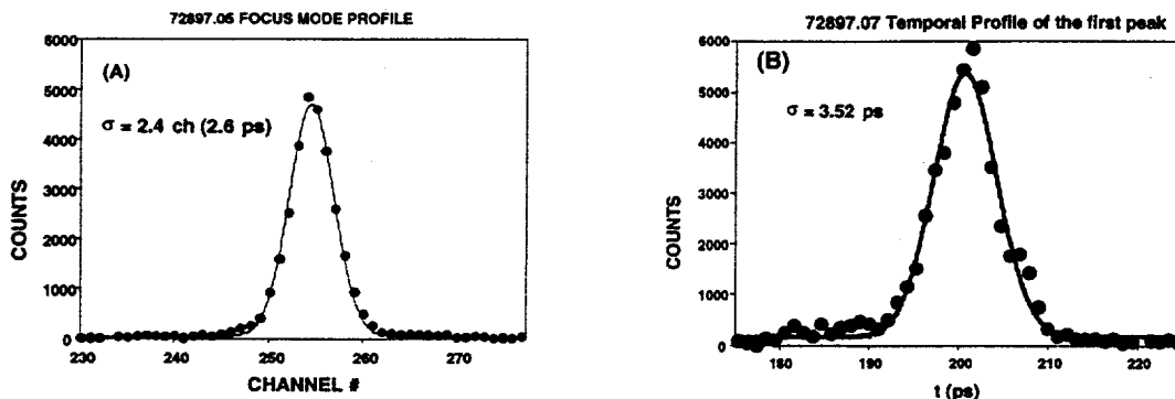
FIGURE 4. Streak camera images taken with a 550 x 40 nm bandpass filter for the focus mode (a) and the R2 streak range (b). The total observed bunch length is about 3.6 ps ( \sigma ) from the conventional gun and buncher system.
