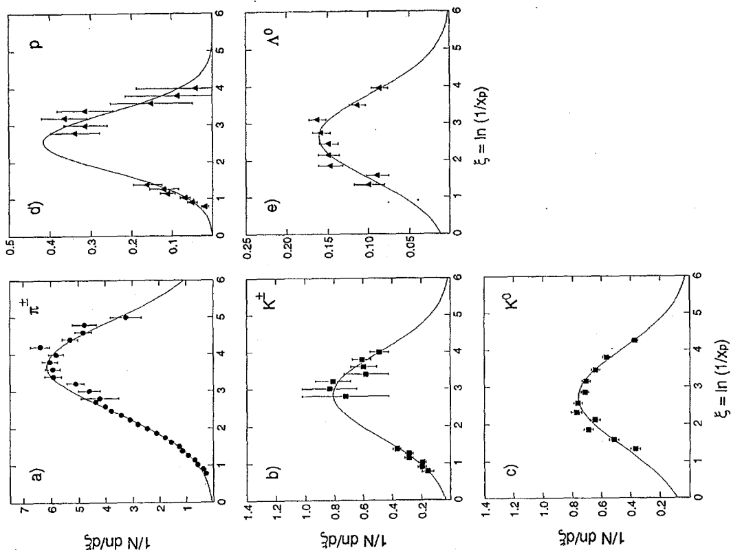
Figure 3: The production spectra for \pi^\pm , K^\pm , K^0 , p , and \Lambda^0 in hadronic Z^0 decays.
