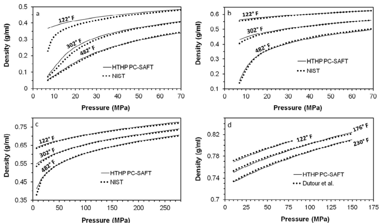
Figure 33: Density predictions for (a) ethane, (b) n-butane, (c) 2-methylpentane, and (d) n-nonadecane obtained using the PC-SAFT equation with HTHP parameters calculated with predictive correlations.
