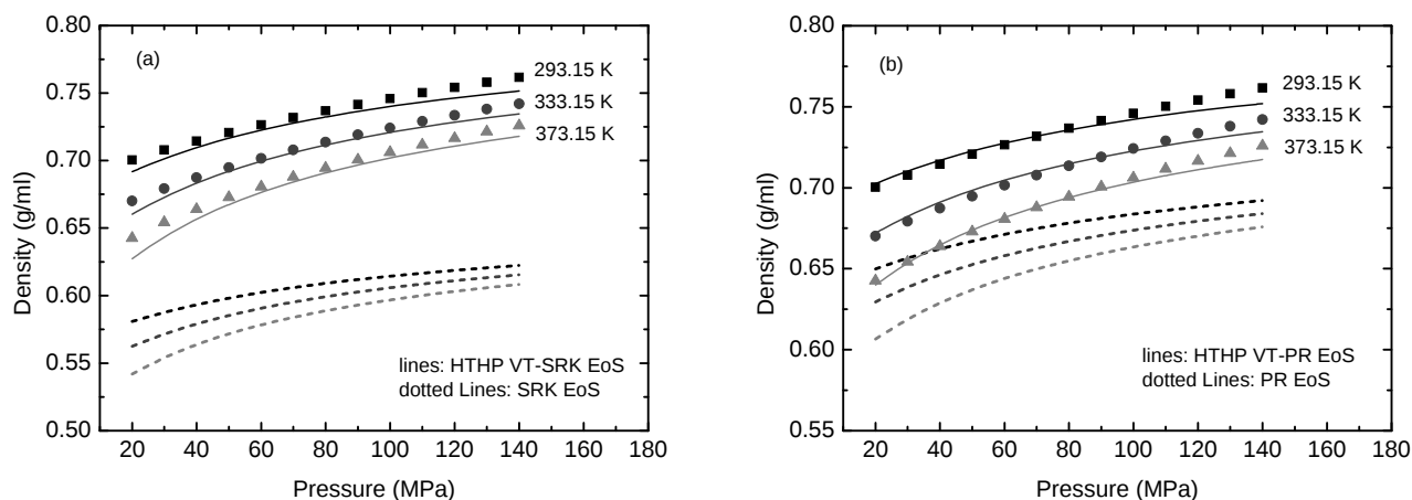
Figure 28: Comparison of density experimental data [64](symbols) of the binary mixture methane/n-decane (x methane = 0.3124) at 293.15, 333.15, and 373.15 K (20, 60, and 100°C) with (a) predicted densities using SRK EoS (dotted lines) and HTHP VT-SRK EoS (lines) with k_{ij} = 0.062 . (b) predicted densities using PR EoS (dotted lines) and HTHP VT-PR EoS (lines) with k_{ij} = 0.065 .
