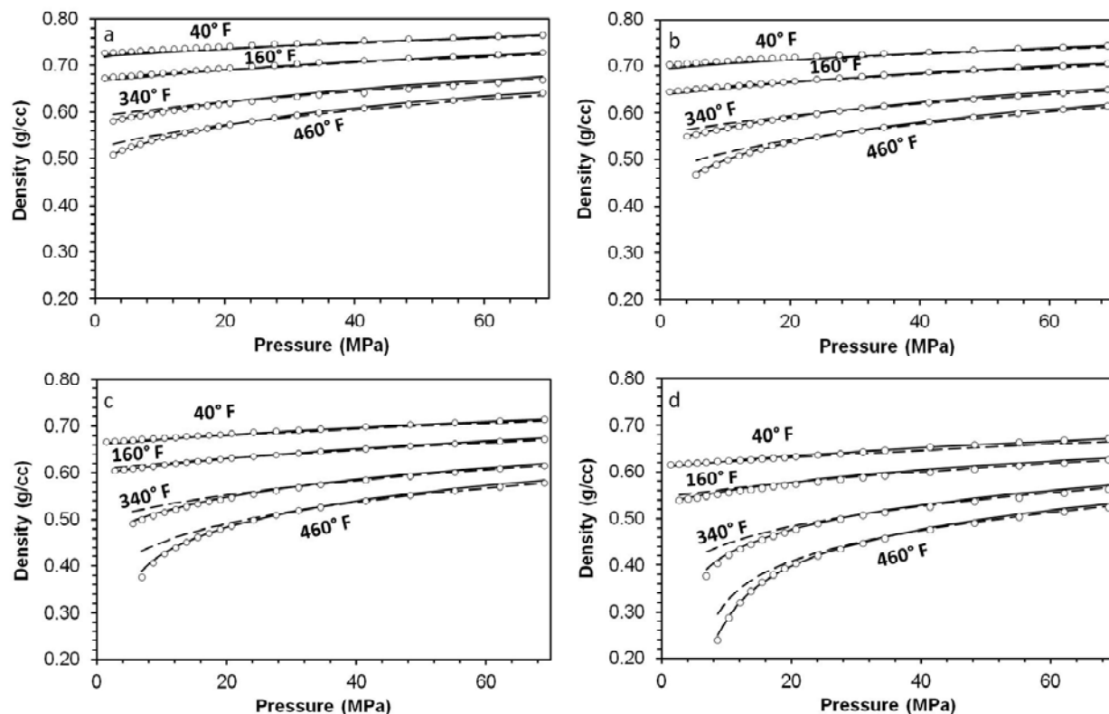
Figure 36: Hybrid PC-SAFT predictions are superior to HTHP PC-SAFT predictions for propane-n-decane mixtures of composition (a) 0.2:0.8, (b) 0.4:0.6, (c) 0.6:0.4, and (d) 0.8:0.2. k_{12} = 0 . ( — ) Hybrid PC-SAFT ( - - - ) HTHP PC-SAFT (o) Reamer and Sage [78].
