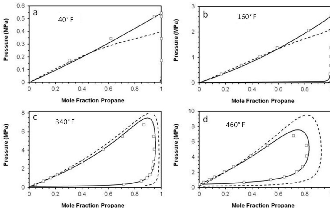
Figure 39: The hybrid PC-SAFT phase compositions for C_3/C_{10} binary predictions are almost identical to those predicted by the G-S PC-SAFT method at (a) 277.6 K, (b) 344.3 K, (c) 444.3 K, and (d) 510.9 K. k_{12} = 0 . (—) Hybrid PC-SAFT (---) HTHP PC-SAFT (o) Reamer and Sage [78].
