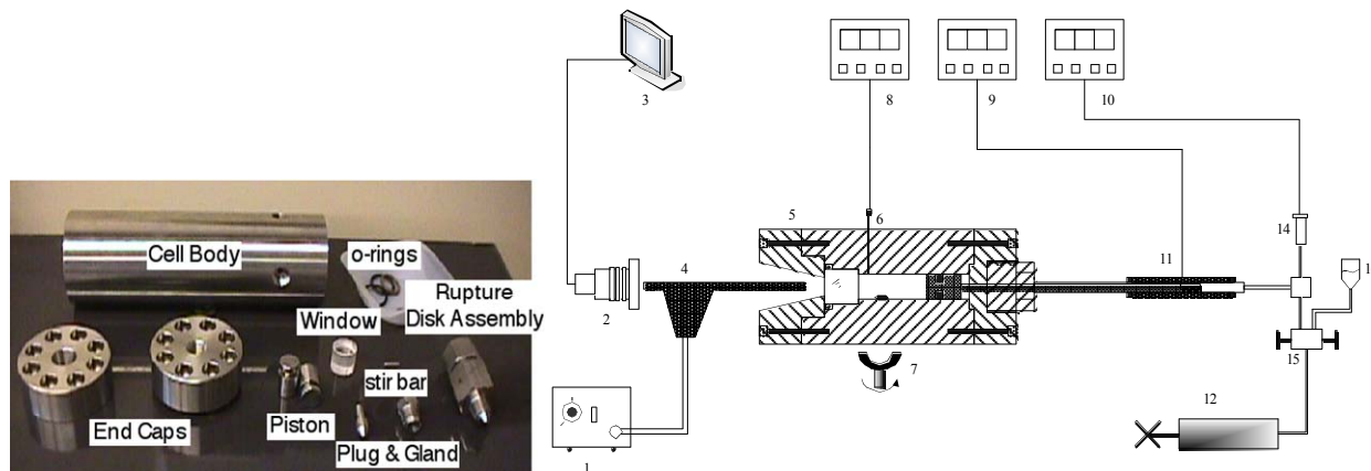
Figure 6: View cell apparatus (not to scale) and picture of the view cell parts. 1. light source 2. camera 3. monitor 4. boroscope 5. high-pressure view cell 6. thermocouple 7. magnetic stirring 8. temperature readout 9. linear variable differential transformer (LVDT) readout 10. pressure readout 11. LVDT 12. pressure generator 14. pressure transducer 15. double-stem valve 16. water reservoir.
