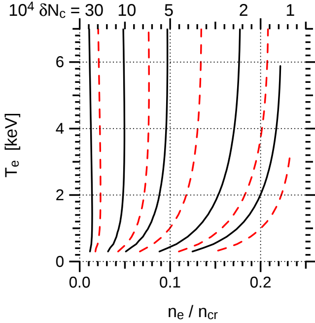
FIG. 10. (Color online.) Threshold Langmuir wave amplitude for collisions, \delta N_c . LW \omega_2 and k_2 are for phase-matched SRBS with a natural LW (black solid curves of Fig. 7), and pump wavelength \lambda_0 = 351 nm. Black solid: Z_{\text{eff}}=1 . Red dash: Z_{\text{eff}}=4 . From right to left, curves are for \delta N_c = [1, 2, 5, 10, 30] \times 10^{-4} .
