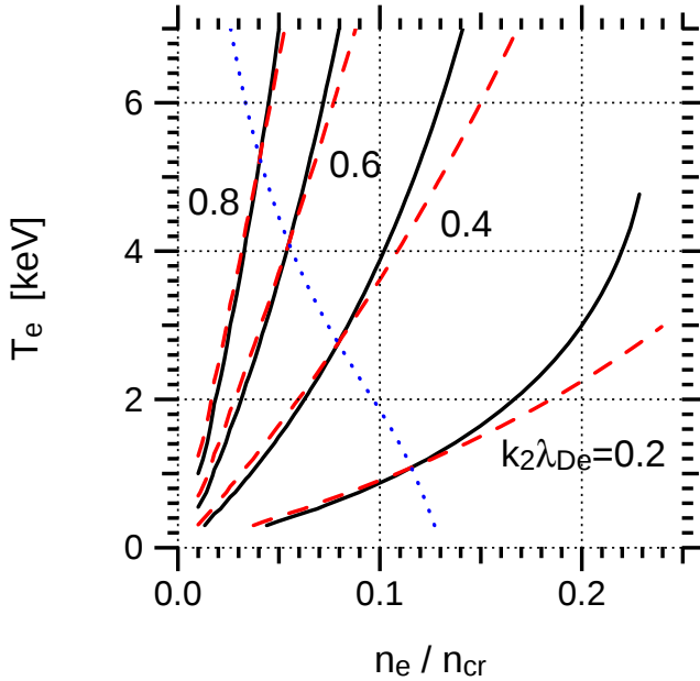
FIG. 8. (Color online.) Langmuir wave k_2 \lambda_{De} phase-matched for SRBS with different \lambda_1 choices, for a pump wavelength \lambda_0 = 351 nm. Black solid: \lambda_1 phase-matched with a natural Langmuir wave, as in black solid curves of Fig. 7. Red dash: \lambda_1 = 550 nm ( \omega 's fixed, k 's vary). Blue dot: \lambda_1 = 550 nm black-solid contour from Fig. 7.
