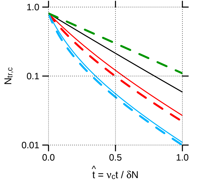
FIG. 5. (Color online.) Trapped fraction due to collisions N_{\text{tr},c} vs. unitless time \hat{t} defined in Eq. (27). Solid curves are exact results from Eq. (29). (u_p, Z_{\text{eff}}) = (2, 1) , (4, 1) , and (4, 4) for black, red, and blue, respectively. Dashed red and blue curves are approximate results for u_p \rightarrow \infty from Eq. (A19), which depend only on Z_{\text{eff}} and not u_p . Green dashed curve is 0.81 \exp[-2\hat{t}] , the approximate form neglecting the term proportional to \hat{t} in the denominator. N_{\text{tr},c}(t = 0) = 0.81 and not unity due to electrons not initially in the fundamental u_x mode.
