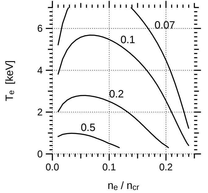
FIG. 11. Ratio \delta N_c/\delta N_{sl} from Figs. 9 and 10 for Z_{\text{eff}}=4 .
