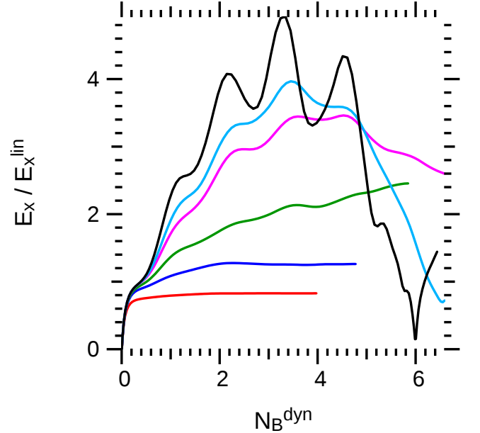
FIG. 3. (Color online.) Amplitude of k = k_0 mode of E_x(y = 0) for 2D LOKI runs with transverse driver profiles h(y) with various L_y . Run parameters and curve meanings are given in Table II. Black curve is 1D run 1D.35c.
