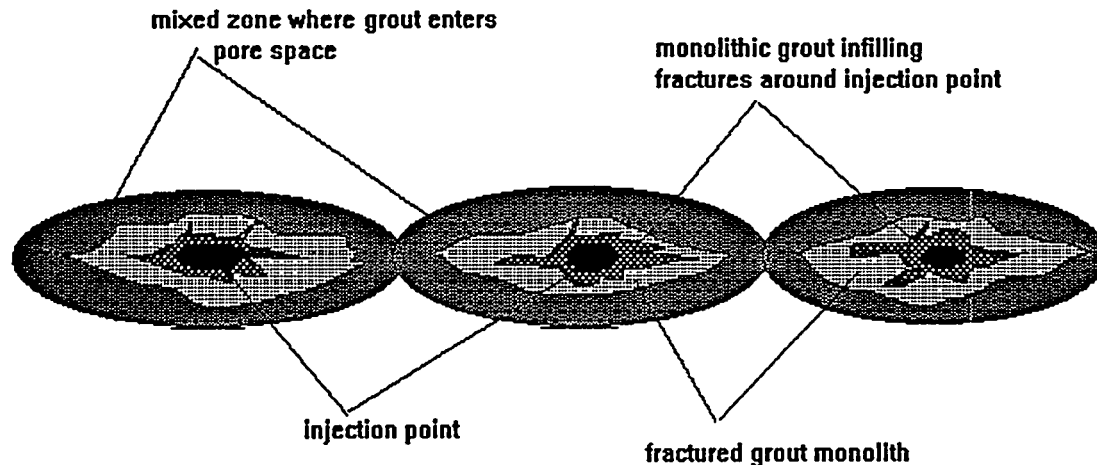
Figure 3: Conceptual Cross-Section of Subsurface Grout Barrier
