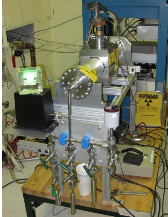
Figure 5-4: Refurbished horizontal source. Shown are the new \frac{1}{2} " diameter pipes and the two bottles of \text{UF}_6 (foreground, bottom). The bottle on the right is empty.
