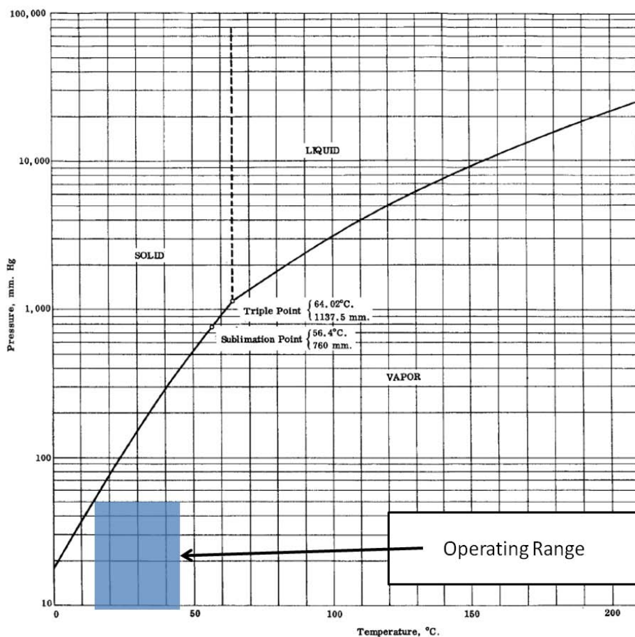
Figure 4-5: \text{UF}_6 phase diagram showing (in blue) the temperature and pressure operating range of our experiments. Tests were performed with \text{UF}_6 in the gas phase only. The only area that approached the freezing of the gas was at 15^\circ\text{C} at 50 Torr, so the source temperature was always kept at or above 15^\circ\text{C} .
