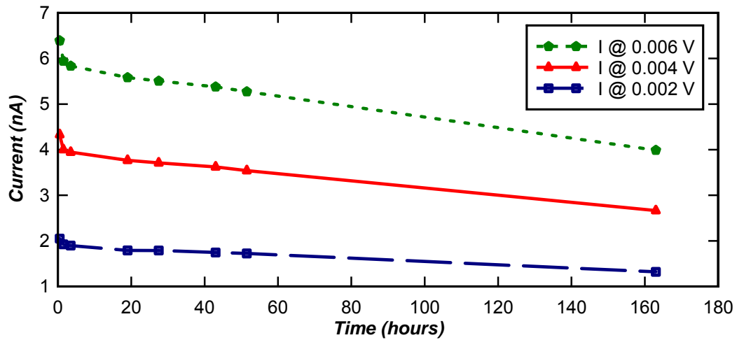
Figure 5-3: Observed recovery of the flux monitor diode after the long-term irradiation test for three voltages on the I-V curve shown in Fig. 5.2. Short- and long-term recovery of the diode from charge trapping is shown.
