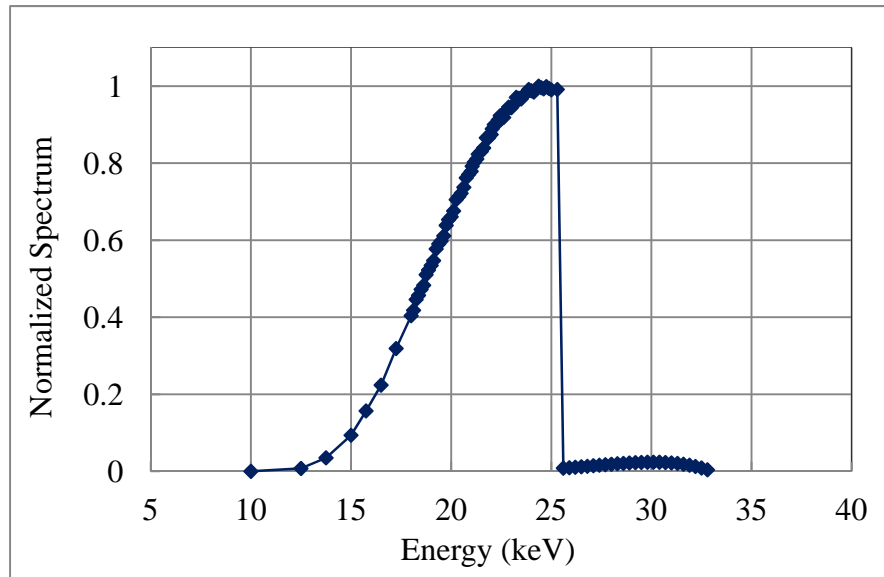
Figure 4-8: Calculated spectrum generated by an x-ray tube with a 0.1-mm-thick silver notch filter.
