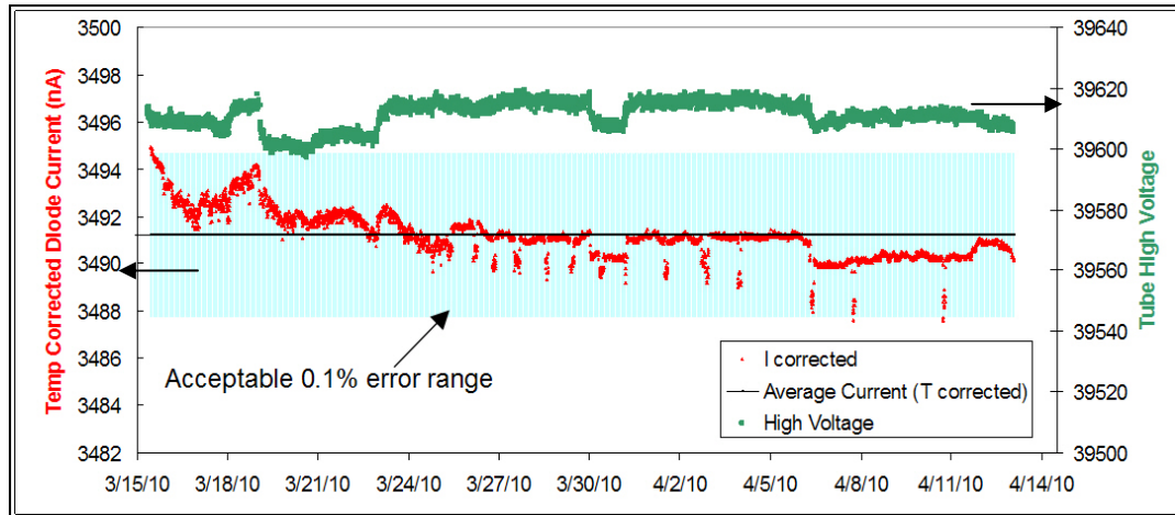
Figure 5-1: Long-term irradiation test of the flux monitor diode at 40 kV and 1 mA. Temperature-corrected diode data are shown, plus high voltage, to help explain the remaining fluctuations.
