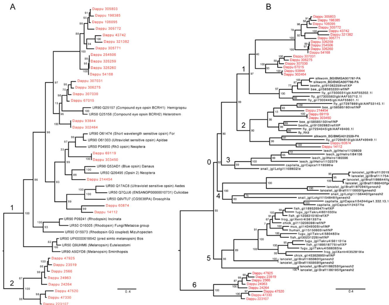
Figure S22. Maximum-likelihood phylogenies of Daphnia pulex opsin genes for comparison to evolution of other gene families involved in vision and eye development [S66]. Bootstrap support at the nodes is reported as concordance among 100 pseudo-replications. We included two clades of opsins in this analysis: rhabdomeric opsins (panel A, lineage 1), and the newly described arthropsin clade (panel A, lineage 2). Consistent with previous analyses [S97], this analysis recovers rhabdomeric opsins only from the bilaterian animals. A reconciled tree analysis (inferring the timing of gene duplication and loss events by comparing a gene tree to a species tree [S66, S160]) identifies 43 well-supported gene duplication events in the evolutionary history of rhabdomeric and arthropsin opsins across all taxa examined – far more than any other phototransduction locus considered by [S66]. Twenty-five of these duplications occurred within the D. pulex lineage alone. One duplication of rhabdomeric opsin predated the bilaterians (panel B, lineage 0); two duplications occurred at least prior to the origin of the Pancrustacea (panel B, lineages 1 and 2), and two duplications preceded the evolution of the vertebrates (Panel B, lineages 4 and 5). This analysis also recorded 13 loss events for rhabdomeric opsins. Because the node joining arthropsins (panel B, lineage 6) to the larger rhabdomeric opsin radiation was weakly supported in this analysis (alrt = 65) (panel B) and because we assigned loss and gain using nodes supported by alrt = 0.9 or greater, we did not record any loss events for this clade. However, the finding that the Daphnia -specific opsin clade arthropsin is basal to rhabdomeric opsins in rooted analyses (Figure S21) suggests that a more complicated history of loss for arthropsins is likely. Panel B lineages: 1 = Rh6/Rh2; 2 = Rh3/Rh4/Rh5/Rh7; 3 = Loph Rh; 4 = Bilateralian Rh; 5 = Melanopsin; 6 = Arthropsin.
