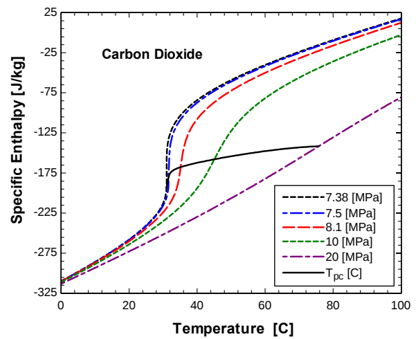
Figure 54: A plot of the temperature versus specific enthalpy of carbon dioxide with several isobars and the pseudo-critical line shown.
