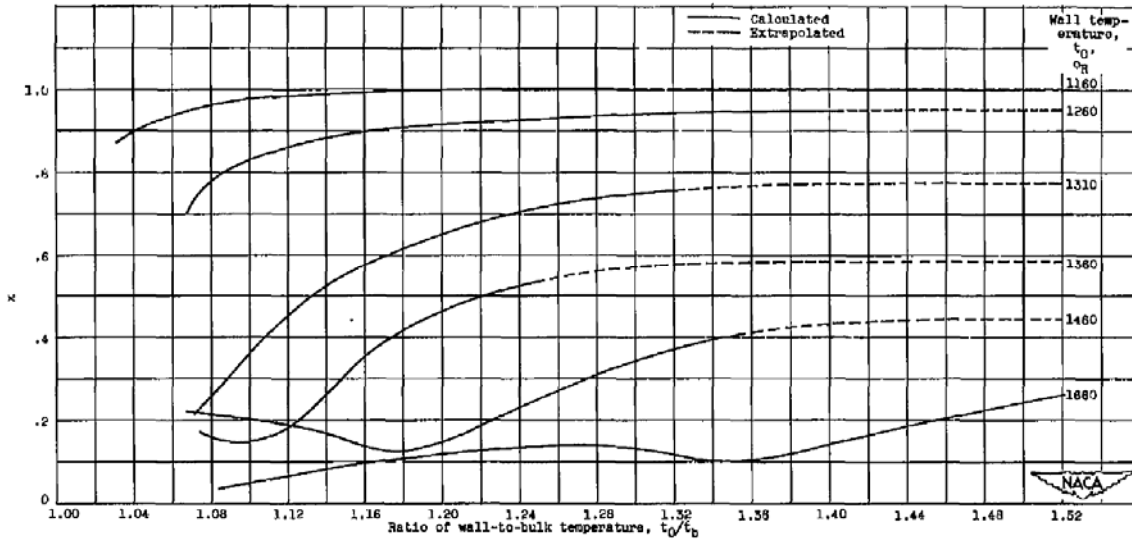
Figure 60: A plot of weighting factor x versus the ratio of wall and bulk temperature, where x is defined by T(x) = x(T_w - T_b) + T_b , for the Nusselt number of water at a pressure of 5000 psi from Deissler and Taylor [30].
