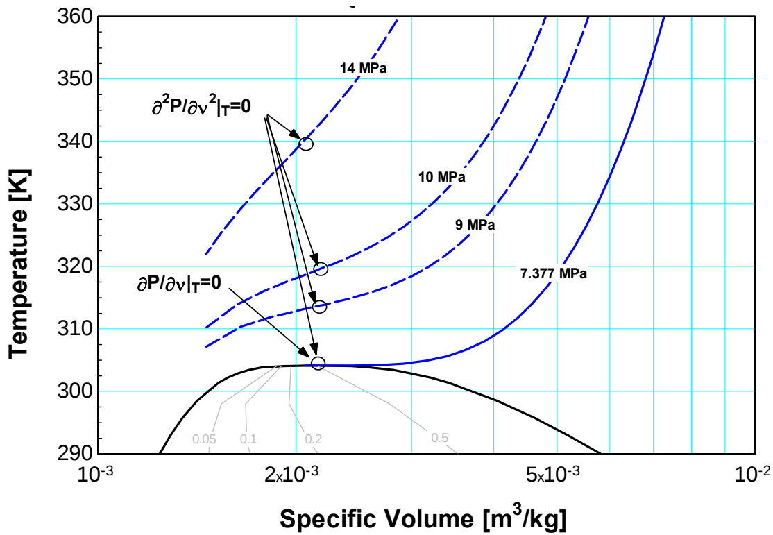
Figure 154 Temperature as a function of specific volume for carbon dioxide, the critical point and approximate location of points on the pseudocritical line are shown.
