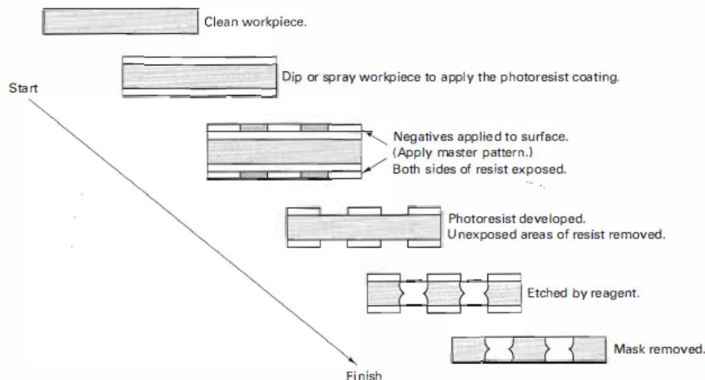
Figure 72: A diagram of the photochemical machining process from Black et al [36]. Note that PCHE plates are typically etched on only one side while chemically blanked plate heat exchangers (CBHE or Marbond™) are etched through from both sides (blanked) as shown.
