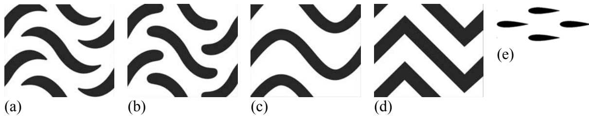
Figure 81: Two-dimensional patterns of various PCHE geometries including (a) sinusoidal fin, (b) rounded sinusoidal fin, (c) sinusoidal, (d) sharp zig-zag, and (e) airfoil fin channels.
