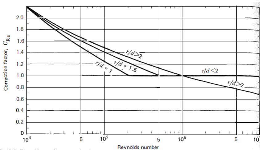
Figure 91: A diagram of the Reynolds number correction factor as a function of Reynolds number and the bend radius to diameter or bend radius to channel width ratio.
