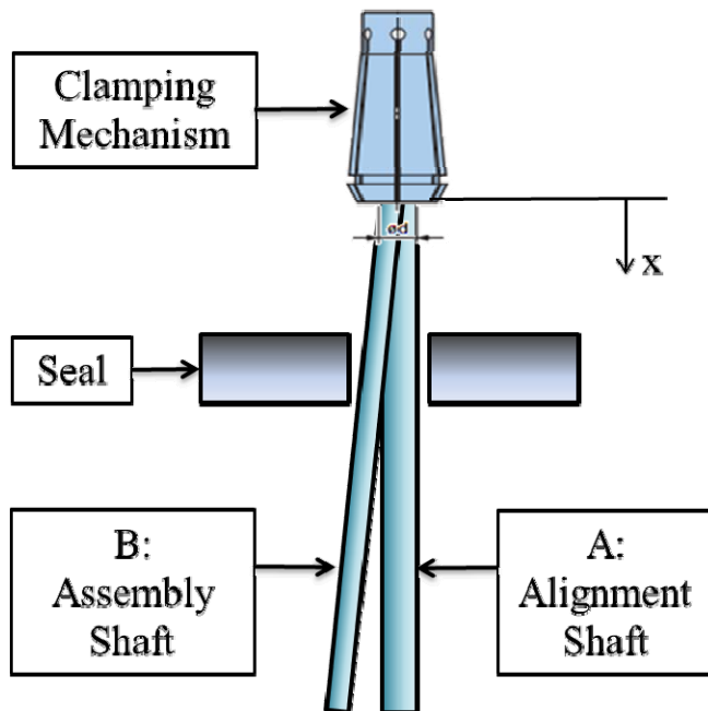
Figure 192 Alignment issues attributed to clamping mechanism error
