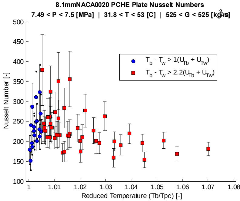
Figure 149: 8.1 mm NACA0020 airfoil fin channel Nusselt number vs. reduced temperature at 7.5 MPa and high mass flux for cooling-mode flow using the measured geometry with error bars indicating propagated uncertainty.
