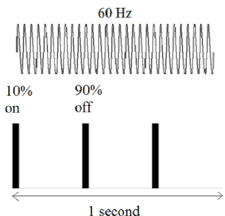
Figure 205 Relay controlled output signature of heaters
