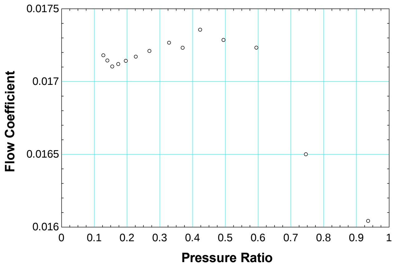
Figure 236 Discharge coefficient for measurements taken with an orifice at P_{\text{inlet}} = 2.07 \text{ MPa} and P_{\text{inlet}} = 7.67 \text{ MPa}
