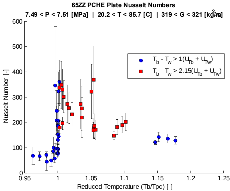
Figure 136: 65-degree zig-zag channel Nusselt number vs. reduced temperature at 7.5 MPa and low mass flux for cooling-mode flow using the measured geometry with error bars indicating propagated uncertainty.
