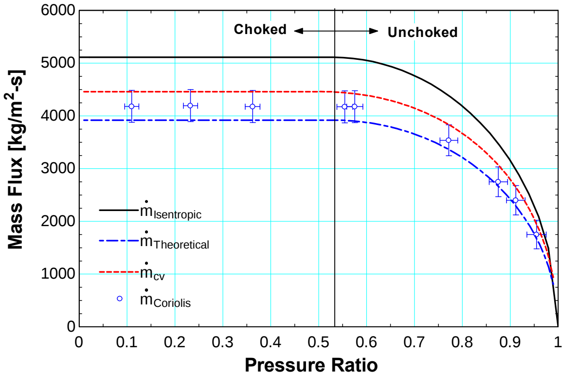
Figure 234 Measurements obtained with a knife-edge orifice at P_{\text{inlet}} = 2.068 \text{ MPa} and \rho_{\text{inlet}} = 24 \text{ kg/m}^3 . Discharge coefficient evaluated at C_d = 0.84 for the data shown.
