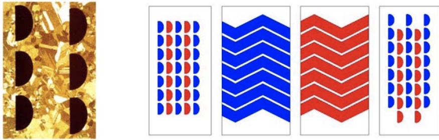
Figure 84: A micrograph of a PCHE cross-section perpendicular to the flow direction, along with a diagram showing cross-sections at two different locations of stacked zig-zag channels indicating that channels may not be equally aligned even in the same block.
