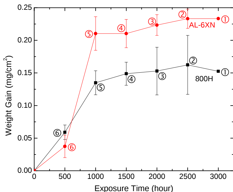
Figure 36: Weight gain (with standard deviation) of the austenitic steels 800H and AL-6XN exposed to the S-CO 2 at 650°C and 20.7 MPa. The circled numbers denote the corresponding number of samples for each data point
