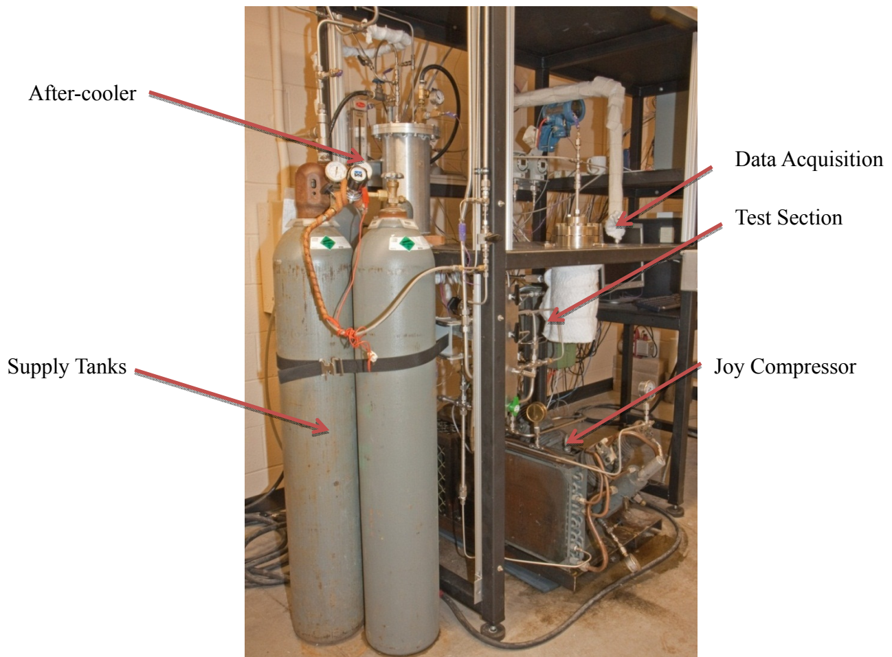
Figure 231 UW-Compression Loop facility (side view)
