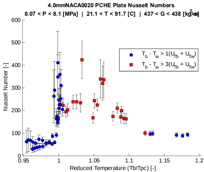
Figure 148: 4.0 mm NACA0020 airfoil fin channel Nusselt number vs. reduced temperature at 8.1 MPa and low mass flux for cooling-mode flow using the measured geometry with error bars indicating propagated uncertainty.
