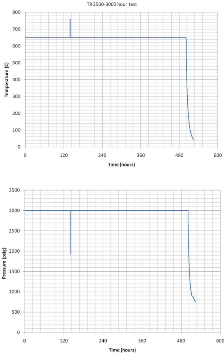
Figure 24 Temperature and pressure history for the 2500-3000 hour test duration
