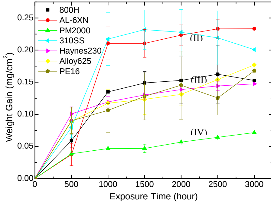
Figure 27: Weight gain of the samples exposed to the s-co2 at 650C
