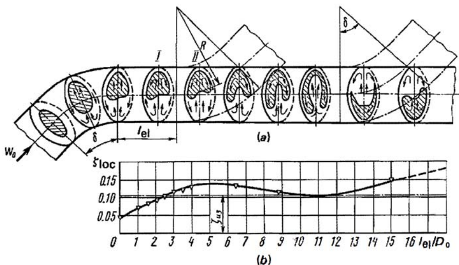
Figure 93: A diagram of a "gooseneck" configuration involving two identical bends with a variable separation length l_{el} . Approximate flow distributions within the channel are shown at various cross-sections (a), while the plot (b) shows measured loss coefficients for the combination of bends as a function of separation length scaled by the pipe diameter. The loss coefficient for an isolated bend is shown (approximately 0.10). From Idel'chik[16].
