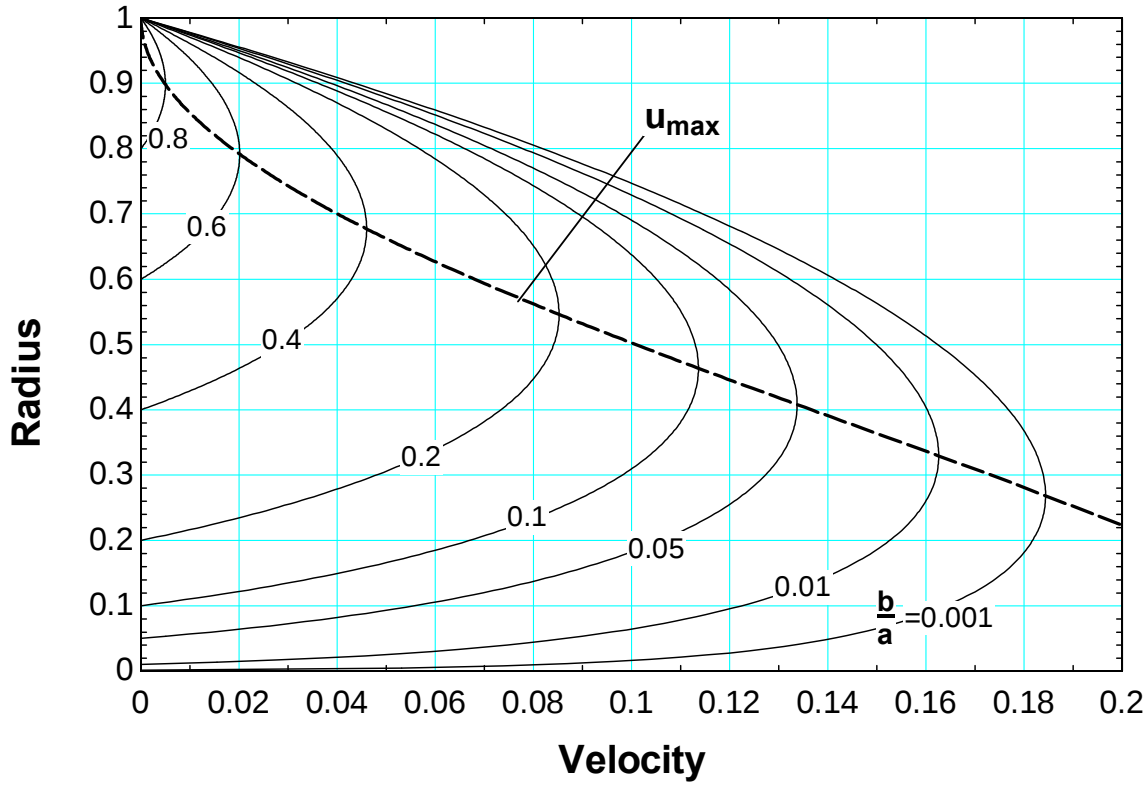
Figure 184 Velocity profiles through an annular region for a=1 , 0 < b/a < 1
