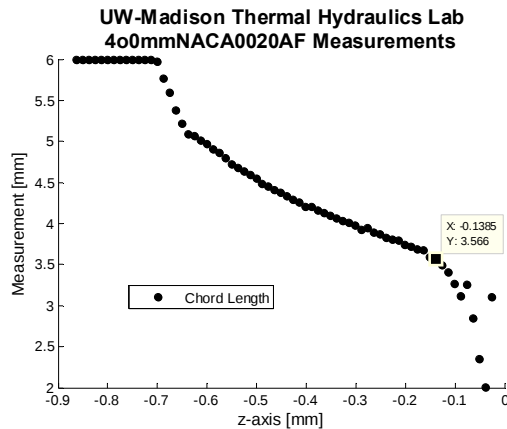
Figure 126: Measured chord length versus depth for the 4.0 mm NACA0020 surface.
