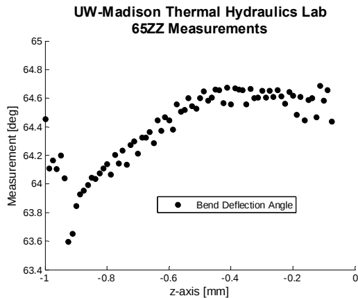
Figure 118: Bend deflection angle versus depth for the 65-degree zig-zag surface.
