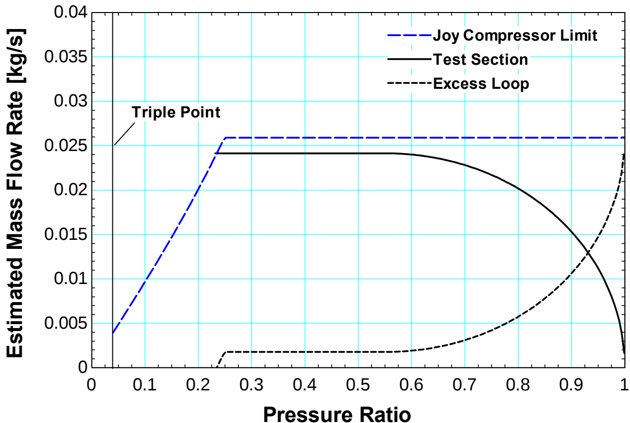
Figure 181 Expected flow rates in test facility from an initial inlet pressure of 13.8 MPa and an upstream temperature of 325 K
