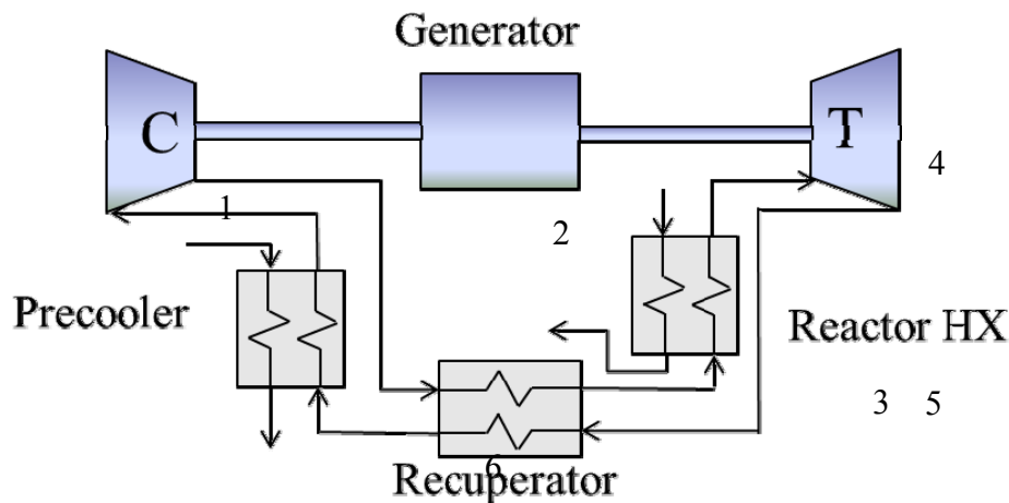
Figure 155 Schematic of S-CO 2 Brayton cycle
