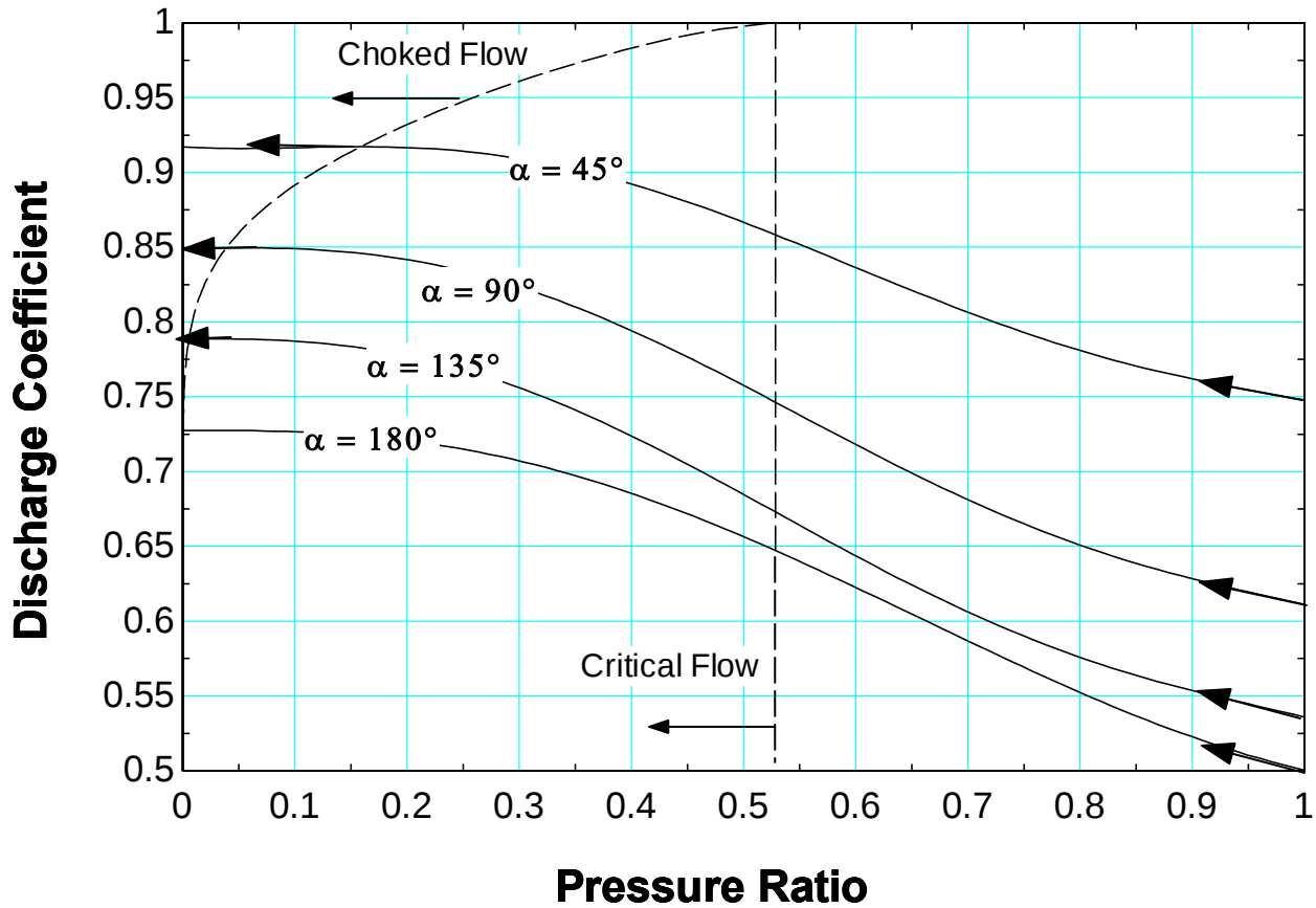
Figure 164 Standard Graph flow map methodology attributed to Linfield (2000). Graph depicts the discharge coefficient for an ideal gas with aspect ratio AR=0 , specific heat ratio k=1.4 , and wall angle \alpha
