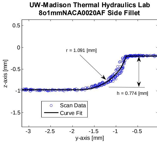
Figure 125: A plot of the averaged unit cell YZ slice at the widest section of the airfoil fit to the “StepFillet” function with the measured height and radius overlaid for the 8.1 mm NACA0020 surface.
