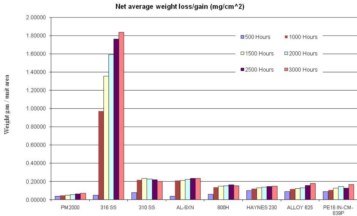
Figure 26: Bar graph of sample weights per unit exposed area
