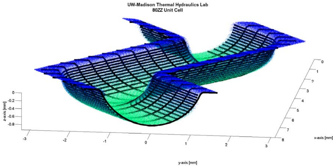
Figure 77: The measured average unit cell of the 80-degree zig-zag channel plate surface with interpolation lines overlaid in black and depth shown as a color gradient from dark blue to light green.
