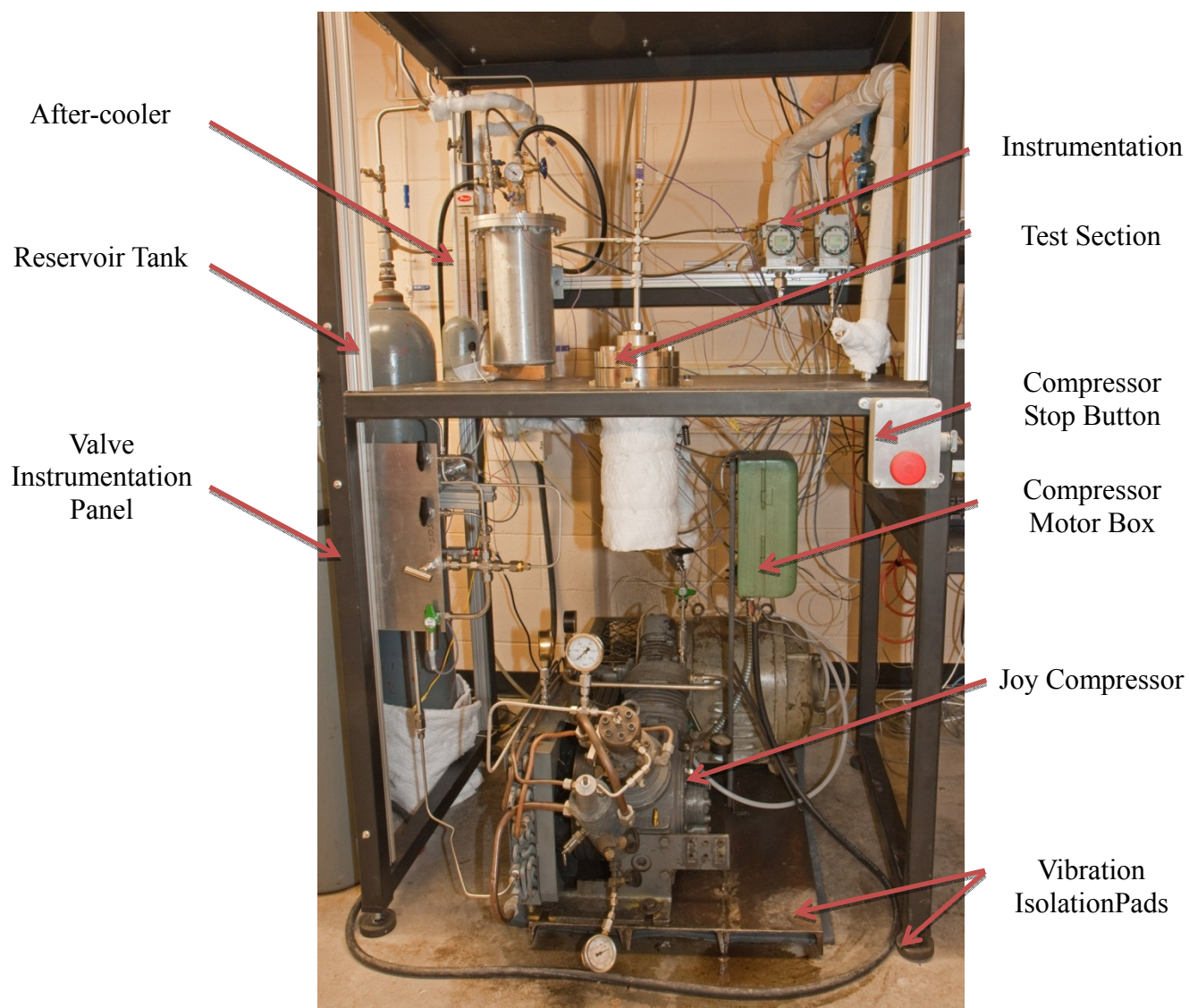
Figure 232 UW Compression-Loop facility (front view)
