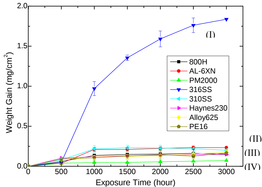
Figure 25: Weight gain of the samples exposed to the s-CO 2 at 650C
