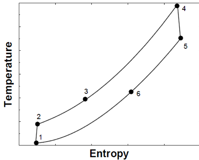
Figure 156 Simple diagram of Brayton cycle
