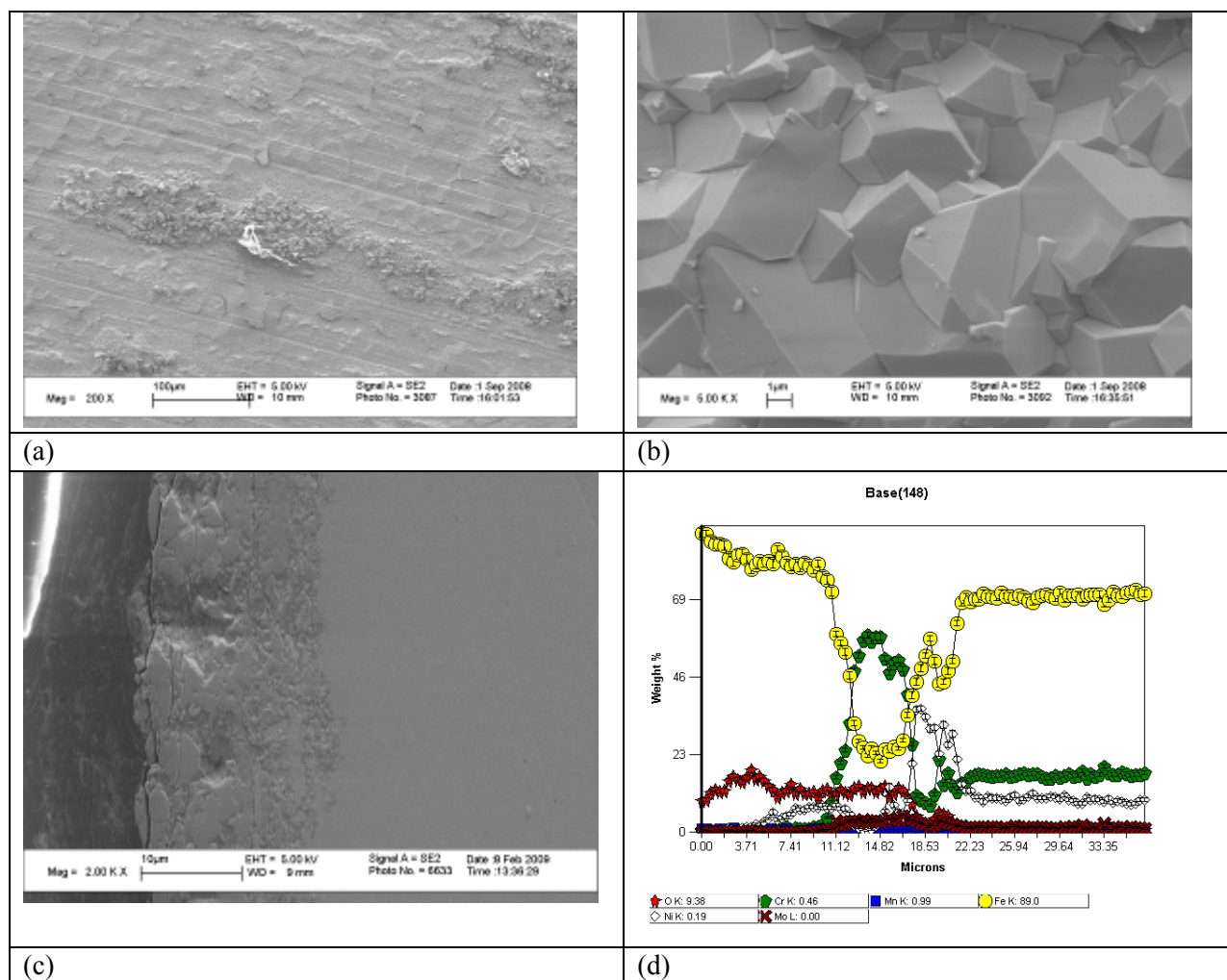
Figure 34: (a) SEM-EDS analysis of the oxide layer formed on 316 stainless steel after exposure to S-CO_2 at 650C, (a) plan view (1000 hours exposure), (b) plan view (1000 hours exposure), (c) cross-sectional view (1500 hours exposure), and (d) EDS line scan across the oxide layer (1500 hours exposure)
