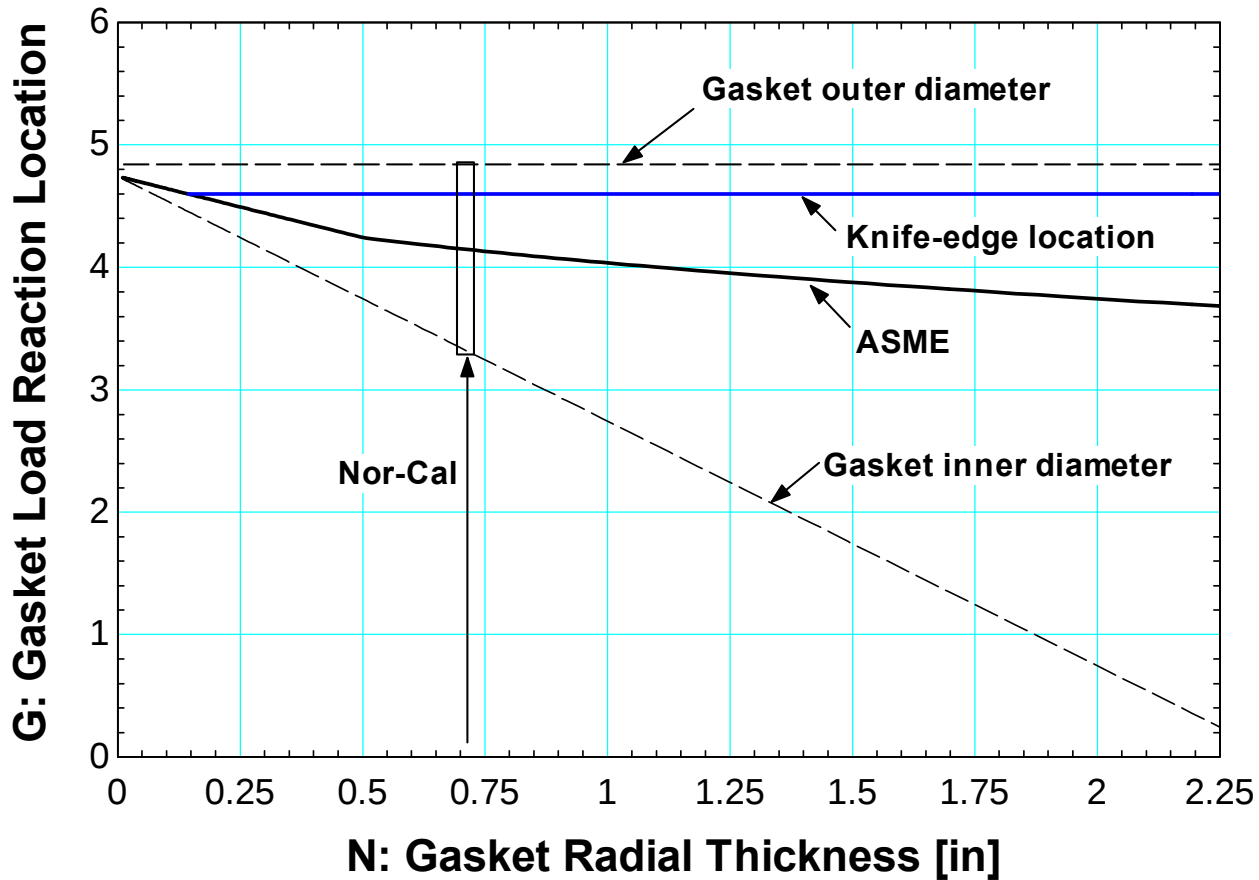
Figure 225 ASME equation-specified gasket load reaction location as a function of gasket thickness. Outer diameter of copper seal used in facility is specified with all other parameters varying according to the gasket thickness
