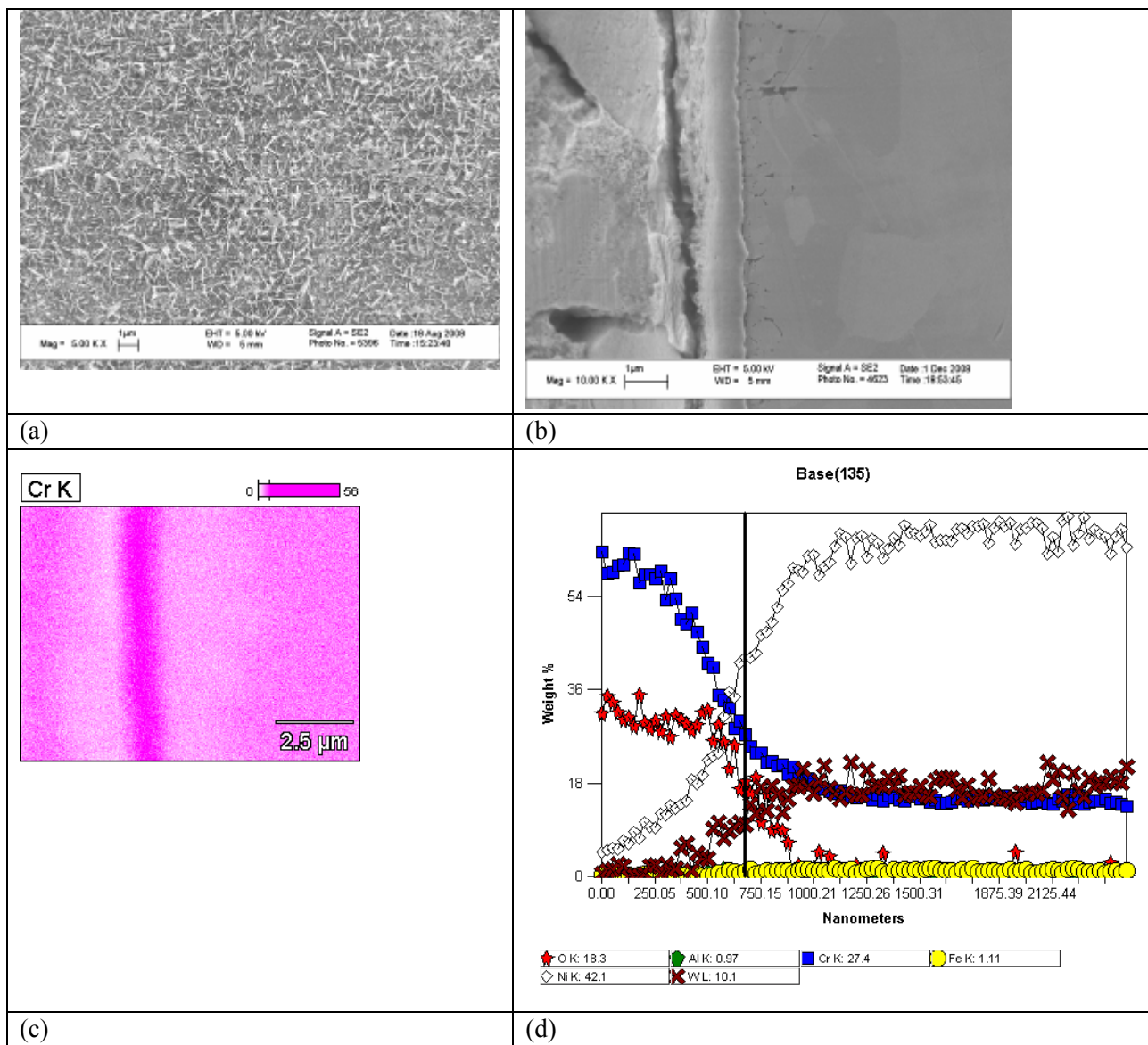
Figure 31: (a) SEM-EDS analysis of the oxide layer formed on Haynes 230 after exposure for 1500 hours, (a) plan view, (b) cross-sectional view, (c) x-ray mapping showing enrichment of Cr, and (d) EDS line scan showing a Cr-rich oxide layer.
