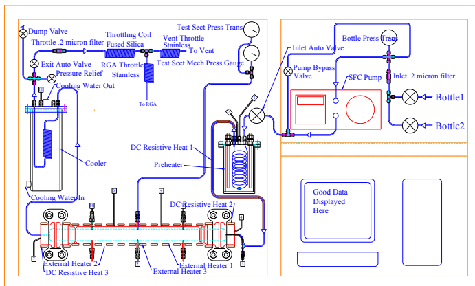
Figure 3 Labview control drawing for operation of the autoclave system showing key components
