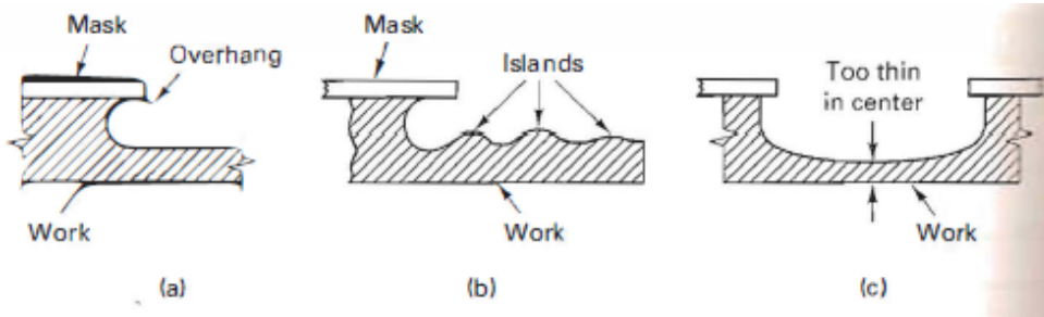
Figure 73: A diagram of photochemical machining defects including (a) overhang, (b) islanding, and (c) dishing, from Black et al [36].
