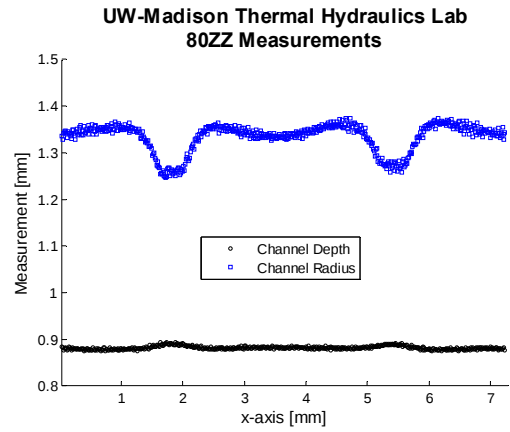
Figure 115: Channel depth and circular segment radius versus x-axis position for the 80-degree zig-zag surface.
