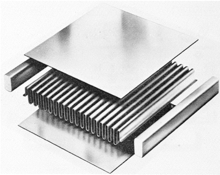
Figure 62: A diagram from Taylor [34] of a single PFHE layer including the corrugation sheet, parting sheets, and side bars.
