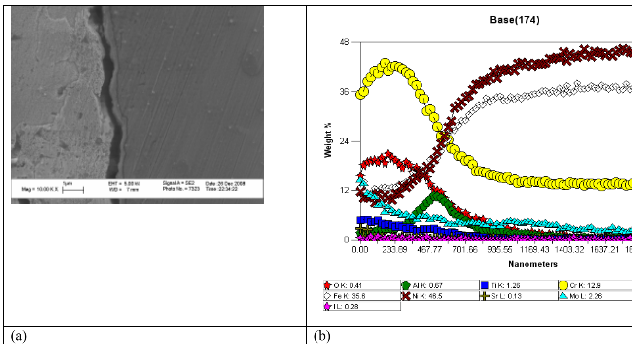
Figure 32: (a) SEM cross-sectional image of the oxide layer formed on Alloy PE16 after 1500 hours exposure and (b) the corresponding EDS compositional line-scan.
