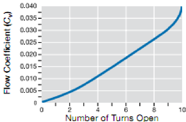
Figure 183 Flow coefficient for SS-31RS4 valve from Swagelok
