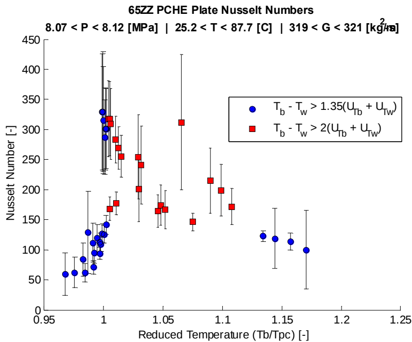
Figure 138: 65-degree zig-zag channel Nusselt number vs. reduced temperature at 8.1 MPa and low mass flux for cooling-mode flow using the measured geometry with error bars indicating propagated uncertainty.
