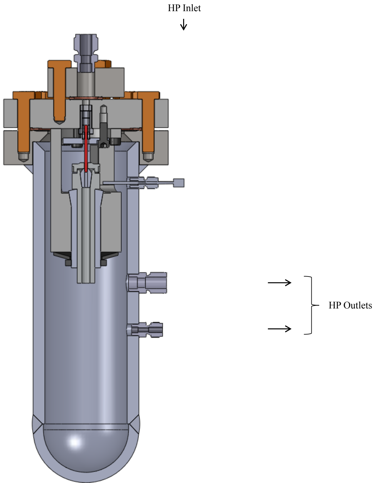
Figure 219 Detailed section view of test section
