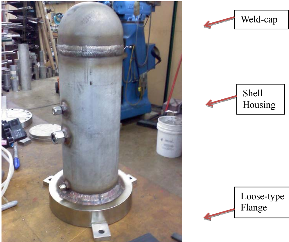
Figure 228 Final assembly of pressure vessel based on this analysis
