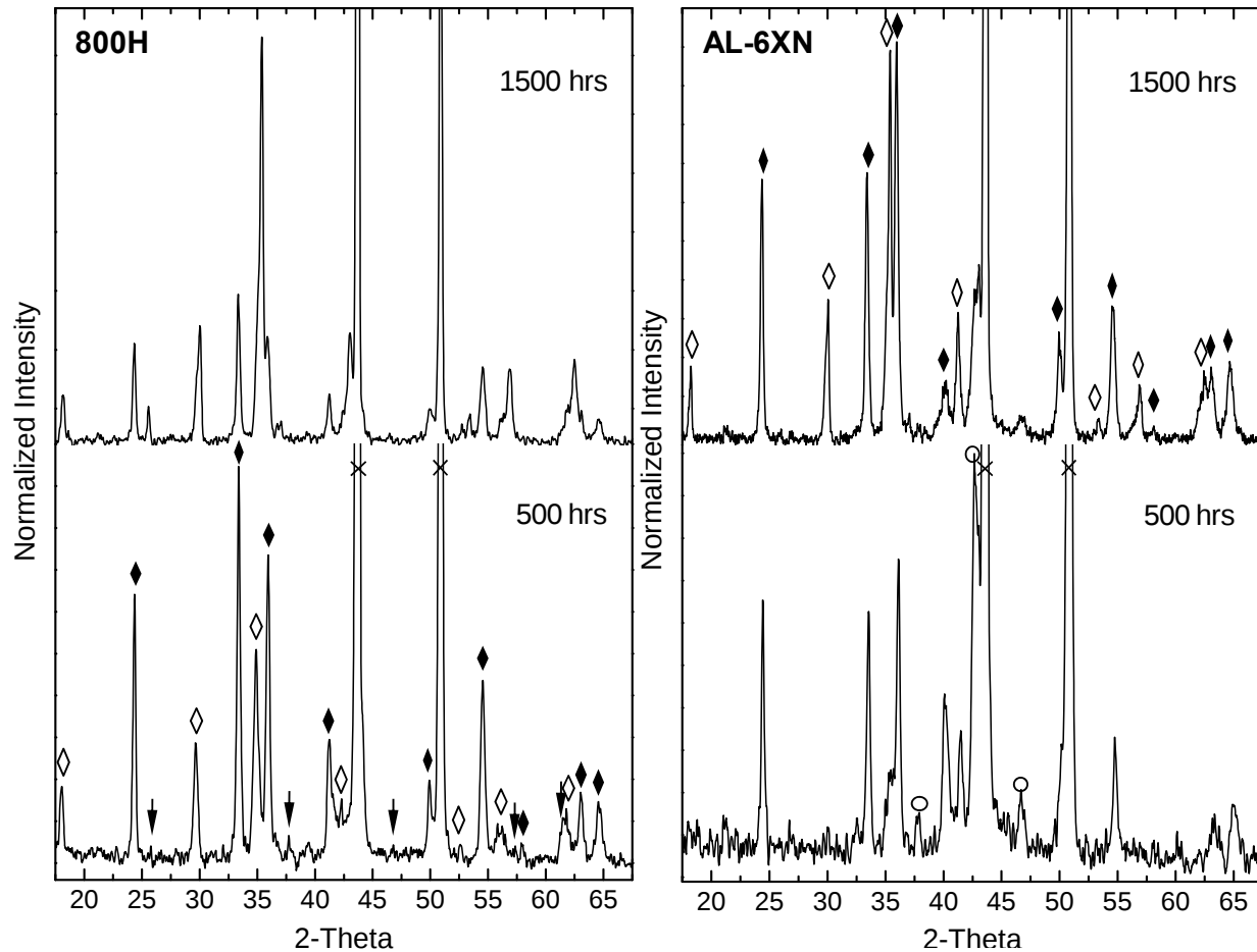
Figure 41: X-ray diffraction patterns of the alloys 800H and AL-6XN samples exposed to the SC-CO 2 at 650°C for 500 and 1500 hours. The symbols ◊, ◆, ↓, ○, and × denote spinel (e.g. (Cr,Mn,Fe) 3 O 4 [44-909]), chromium oxide (e.g. Cr 1.3 Fe 0.7 O 3 [35-1112] or Cr 2 O 3 [38-1479]), alumina (e.g. Al 2 O 3 [10-173]), sigma phase (Fe,Ni) 3 (Cr,Mo) 2 (e.g. Fe 18 Cr 6 Mo 5 [8-200]), and austenite (i.e. substrate), respectively
