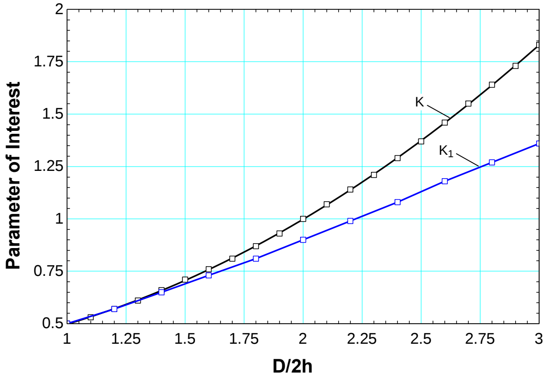
Figure 220 Parameters used to determine inner crown efficiency
