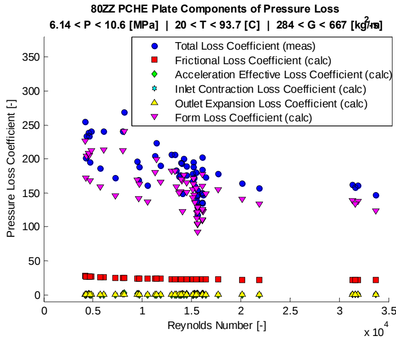
Figure 132: 80-degree zig-zag channel calculated pressure loss components using the measured geometry. Note that calculated acceleration, inlet contraction, and outlet expansion points are approximately the same and overlap.
