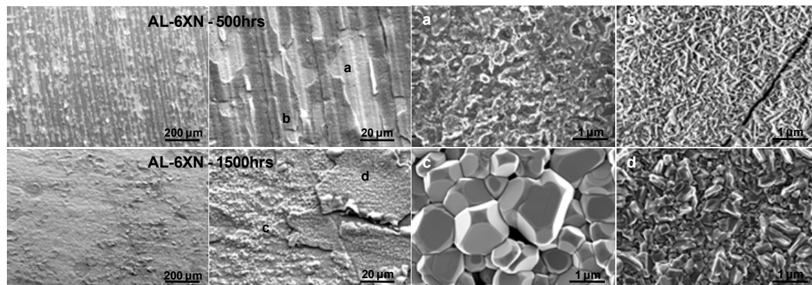
Figure 39: Surface morphologies of the alloy AL-6XN samples exposed to the S- \text{CO}_2 at 650C for 500
