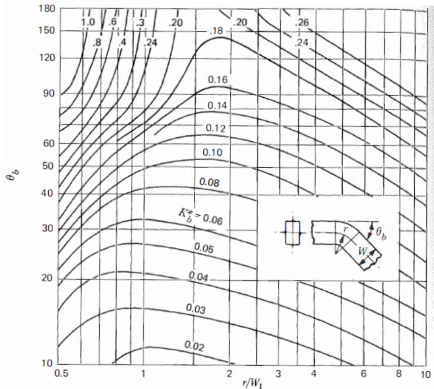
Figure 90: A diagram of the loss coefficient K_b^* for a bend in a rectangular pipe with an aspect ratio of 0.5 as a function of the bend angle \theta_b and the bend radius ratio r/w at a Reynolds number of 10^6 ; from Miller [12].
