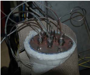
Figure 6 Image of pre-heat can with heaters and S-CO 2 tubing immersed in a copper powder matrix
