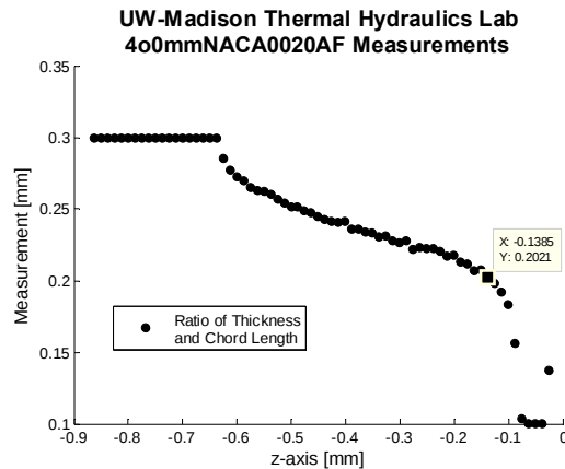
Figure 127: Ratio of thickness and chord length versus depth for the 4.0 mm
