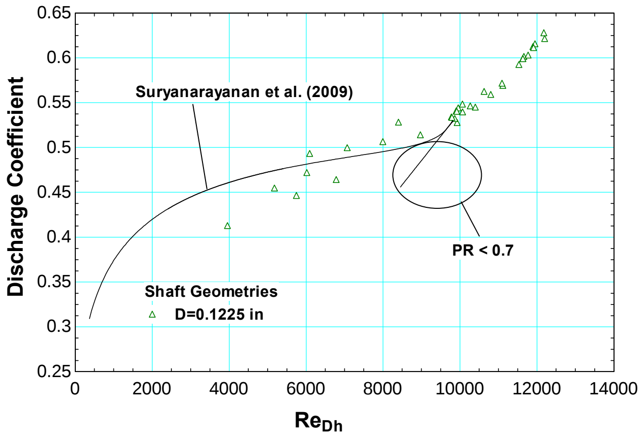
Figure 243 Discharge coefficient as a function of Re_D with compressibility effects included. Measurements demonstrated to deviate from empirical model at pressure ratios less than PR = 0.7 for length to hydraulic diameter ratios L/D_h = 110.3 .
