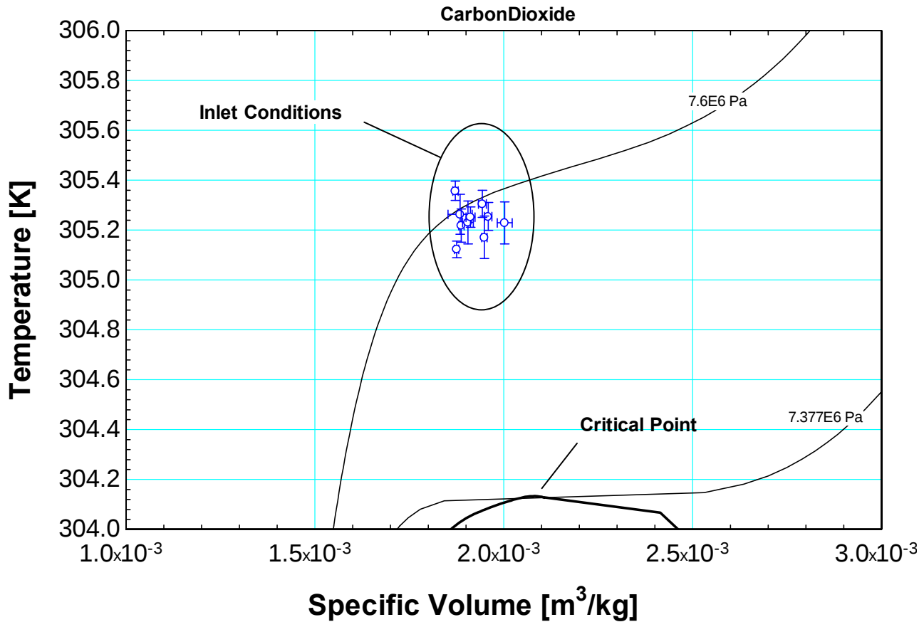
Figure 247 Standard deviation of measurements taken at P_{\text{inlet}}=7.58 \text{ MPa} and \rho_{\text{inlet}} = 500 \text{ kg/m}^3
