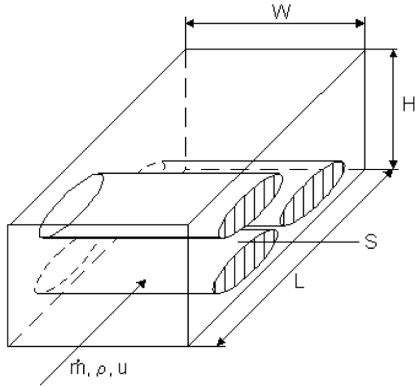
Figure 69: A diagram of a new regenerator comparison methodology proposed by Ruhlich and Quack [42].
