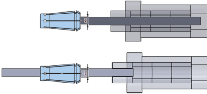
Figure 195 Focus solution which allowed imaging of shaft-seal interface at desired distance from collet tip
