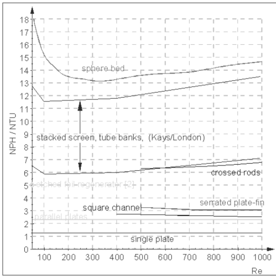
Figure 70: Laminar flow comparison of several regenerator types using porosity-based parameters for a Prandtl number of 0.7, from Ruhlich and Quack [41].
