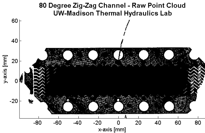
Figure 104: A XY view of the raw point cloud data from the 80 degree zig-zag channel surface scan.
