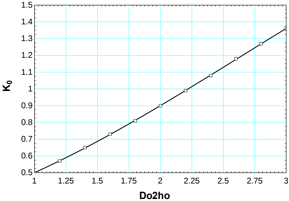
Figure 221 Parameters used to determine outer crown capacity
