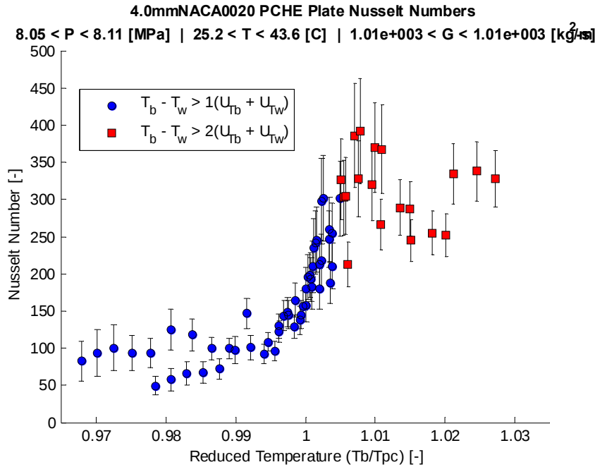
Figure 150: 4.0 mm NACA0020 airfoil fin channel Nusselt number vs. reduced temperature at 8.1 MPa and high mass flux for cooling-mode flow using the measured geometry with error bars indicating propagated uncertainty.
