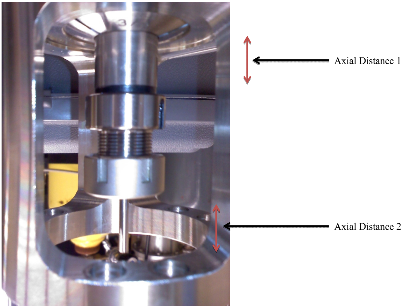
Figure 213 Collet holder sub-assembly shown in configured state with alignment gauge pin attached
