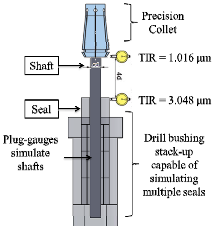
Figure 188 Schematic of components used in eccentricity tolerance calculation
