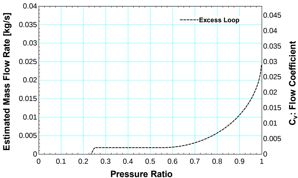
Figure 182 Excess flow loop valve coefficient estimation as a function of pressure ratio and estimated mass flow rate
