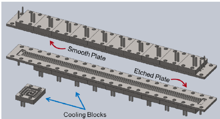
Figure 99: A solid model of the test section plate and cooling block assembly.
