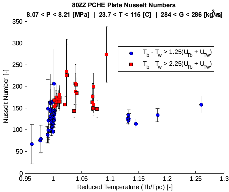
Figure 137: 80-degree zig-zag channel Nusselt number vs. reduced temperature at 8.1 MPa and low mass flux for cooling-mode flow using the measured geometry with error bars indicating propagated uncertainty.
