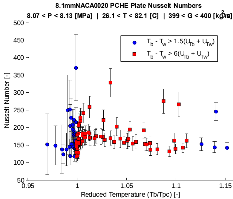
Figure 147: 8.1 mm NACA0020 airfoil fin channel Nusselt number vs. reduced temperature at 8.1 MPa and low mass flux for cooling-mode flow using the measured geometry with error bars indicating propagated uncertainty.
