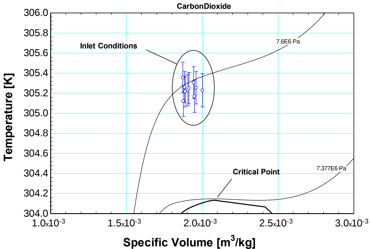
Figure 245 Measurement uncertainty of inlet conditions of data taken at P_{inlet}=7.58 \text{ MPa} and \rho_{inlet} = 500 \text{ kg/m}^3
