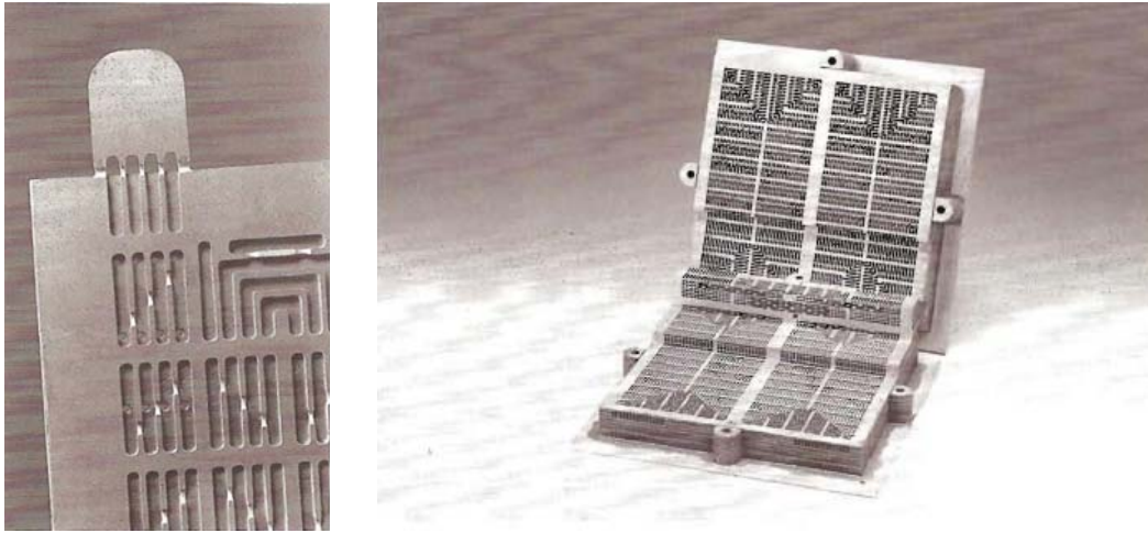
Figure 64: Detail and cut-away views of a CBHE from Hesselgreaves [6].
