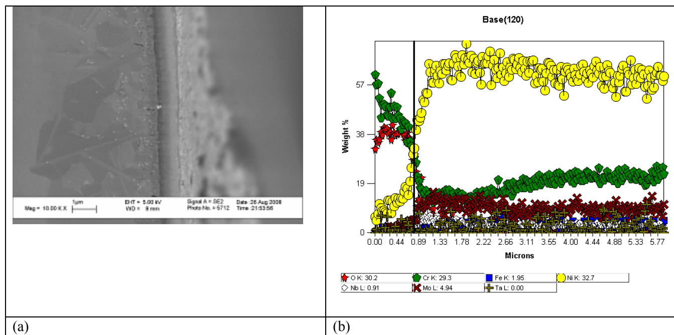
Figure 30: (a) SEM cross-sectional image of the oxide layer formed on Alloy 625 after 1500 hours exposure and (b) the corresponding EDS compositional line-scan
