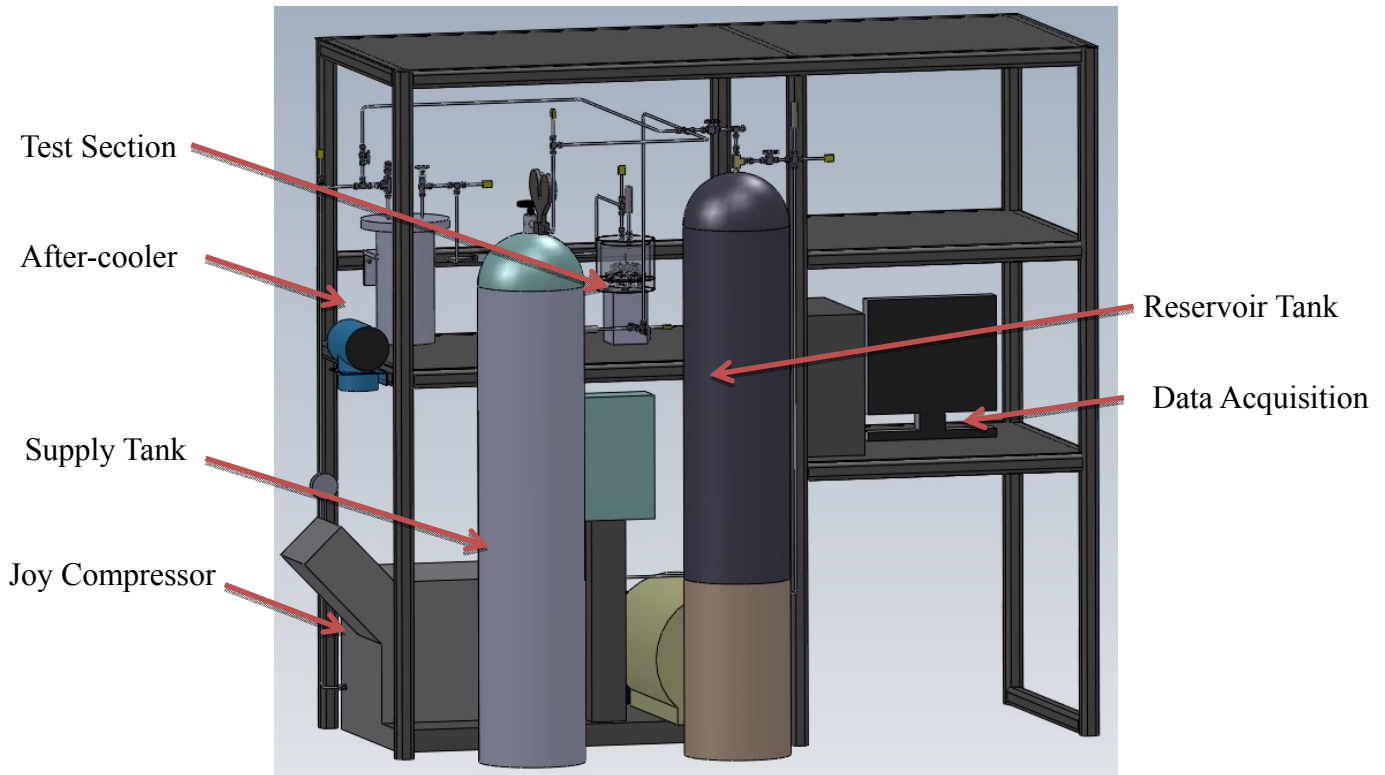
Figure 230 Initial SolidWorks representation of UW-Compression Loop facility
