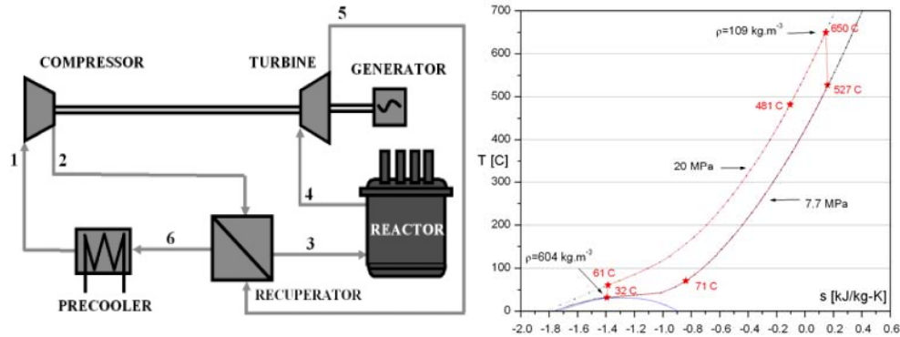
Figure 1: Simple CO 2 Brayton cycle and T-s diagram showing temperature and pressure variations. (Dostal 2006)
