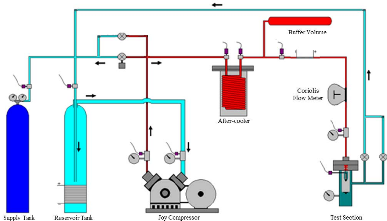
Figure 173 Test facility schematic; red=high pressure, cyan=low pressure
