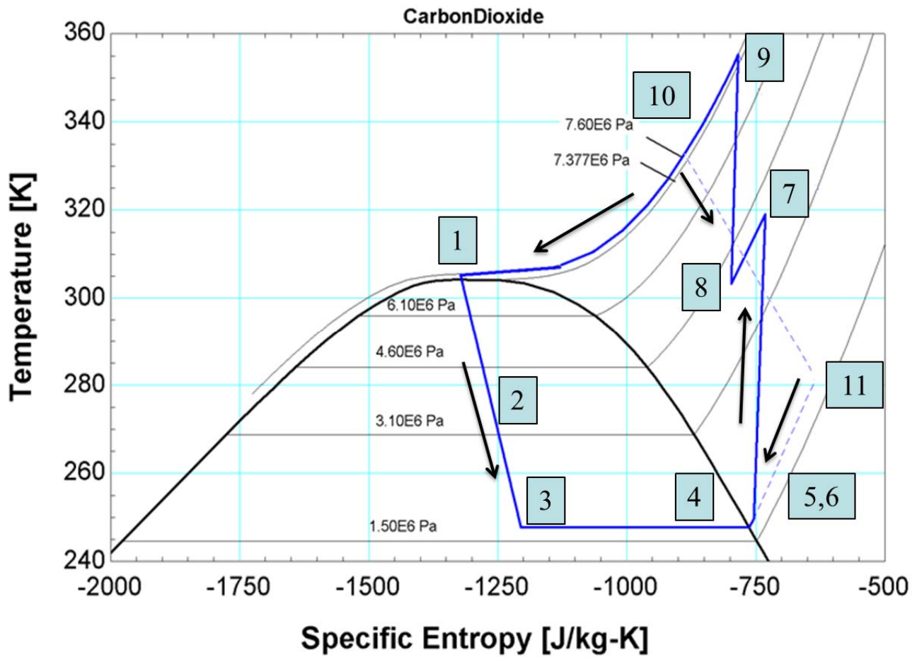
Figure 175 Temperature-entropy diagram of UW-Madison S-CO 2 Compression Loop facility
