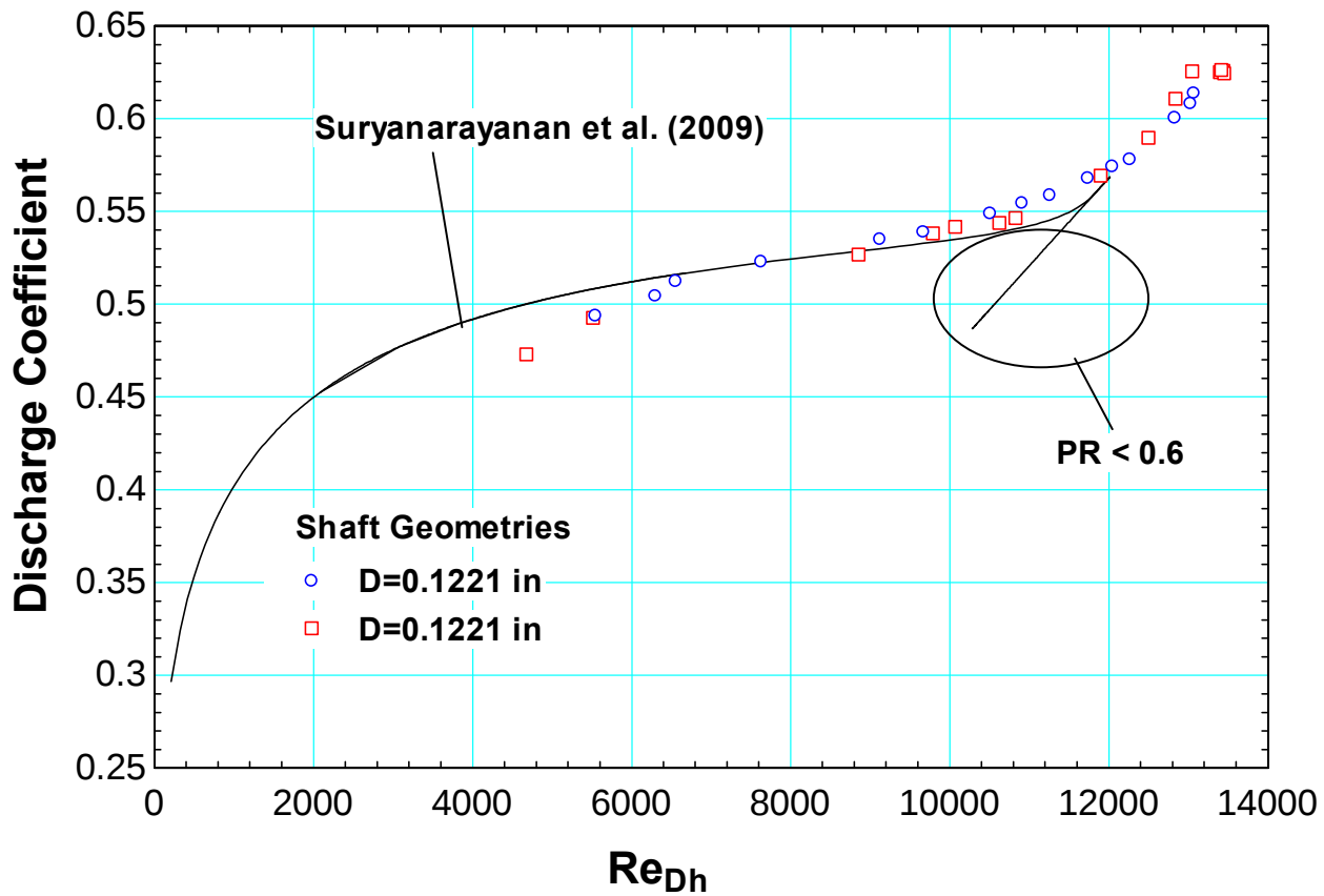
Figure 242 Discharge coefficient as a function of Re_D with compressibility effects included. Measurements demonstrated to deviate from empirical model at pressure ratios less than PR = 0.6 for length to hydraulic diameter ratios L/D_h = 96.2 .
