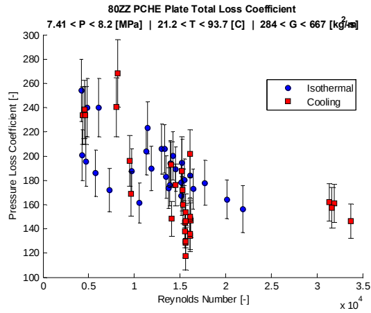
Figure 130: A plot of the 80-degree zig-zag channel isothermal and cooling-mode pressure loss coefficient using the design and measured geometry respectively with error bars indicating propagated uncertainty.
