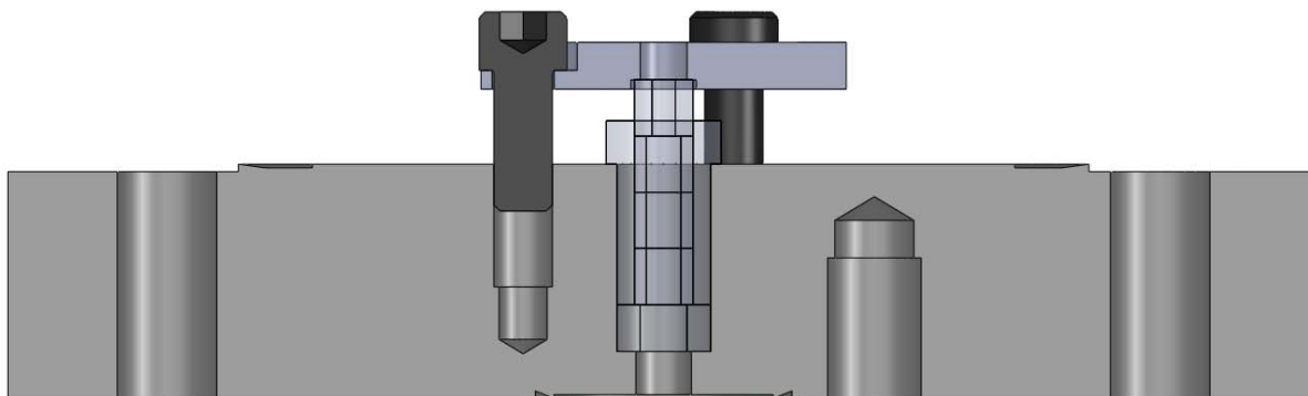
Figure 215 Conflat Flange seal-stackup bolting configuration
