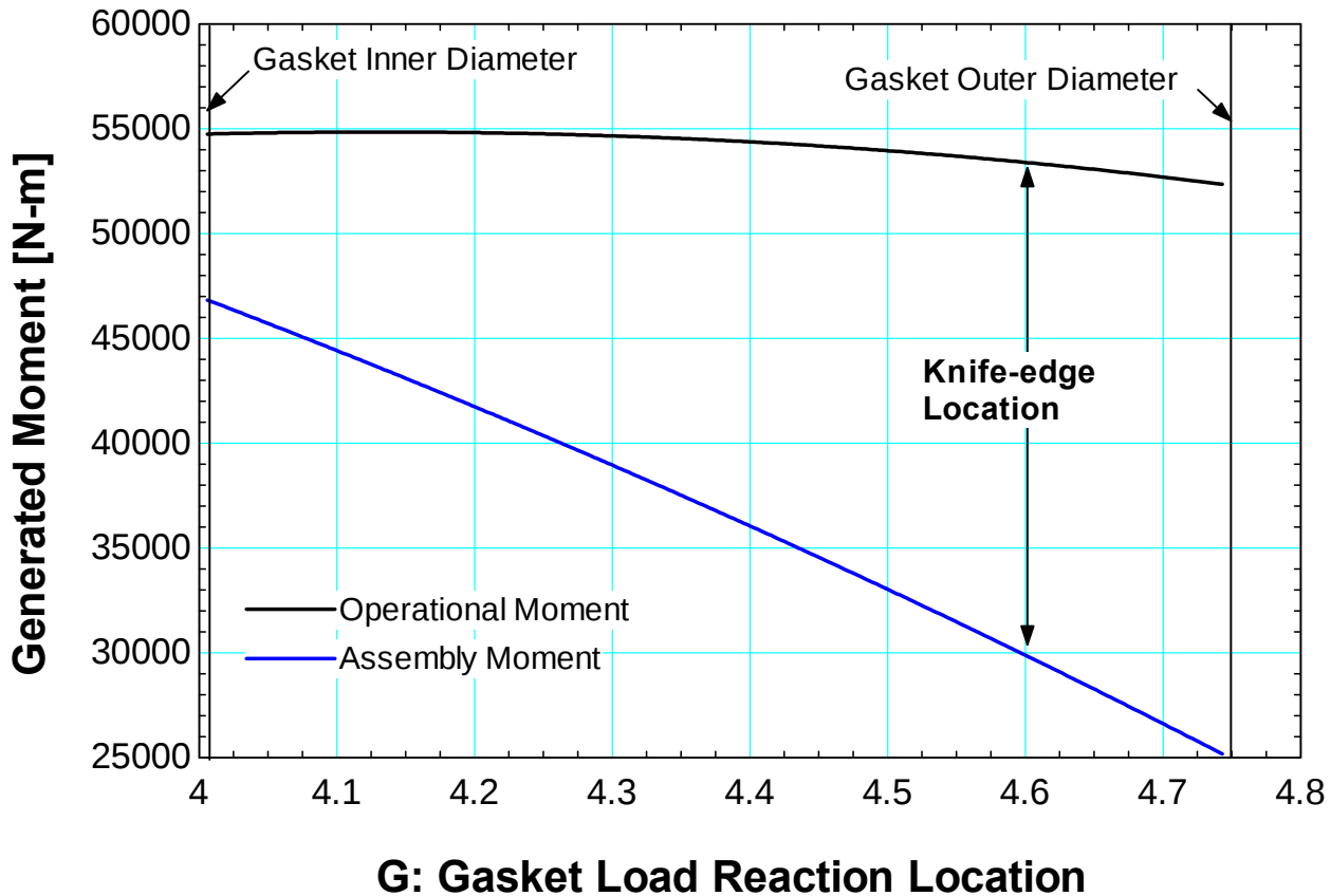
Figure 226 Assembly and operational moments generated as a function of gasket load reaction for the parameters listed in Table 4-19.
