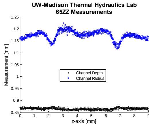
Figure 119: Channel depth and circular segment radius versus x-axis position for the 65-degree zig-zag surface.
