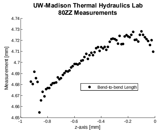
Figure 113: Bend-to-bend length versus depth for the 80-degree zig-zag surface.
