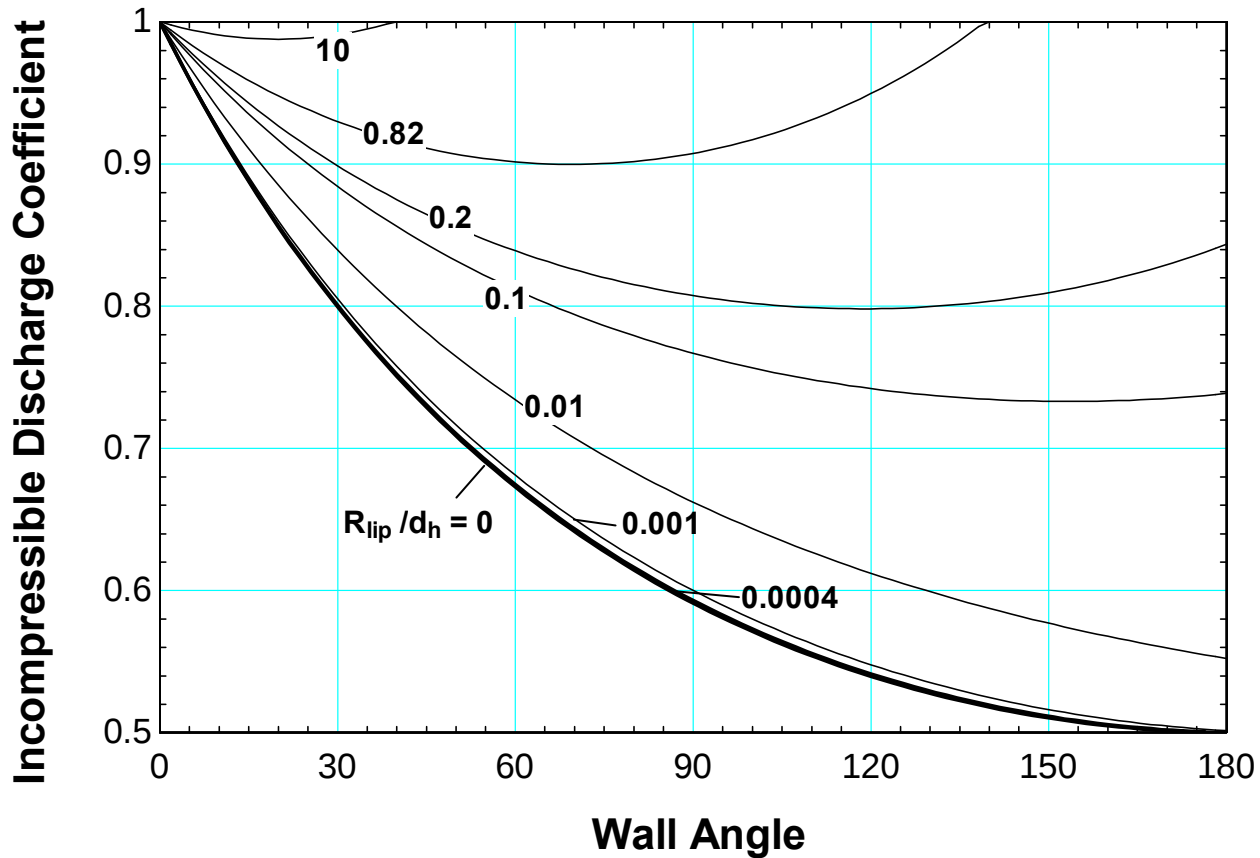
Figure 168 Discharge coefficient for PR=1 as a function of wall angle \alpha for flow through a restriction with different ratios of the lip radius to the diameter of the orifice, k=1.4
