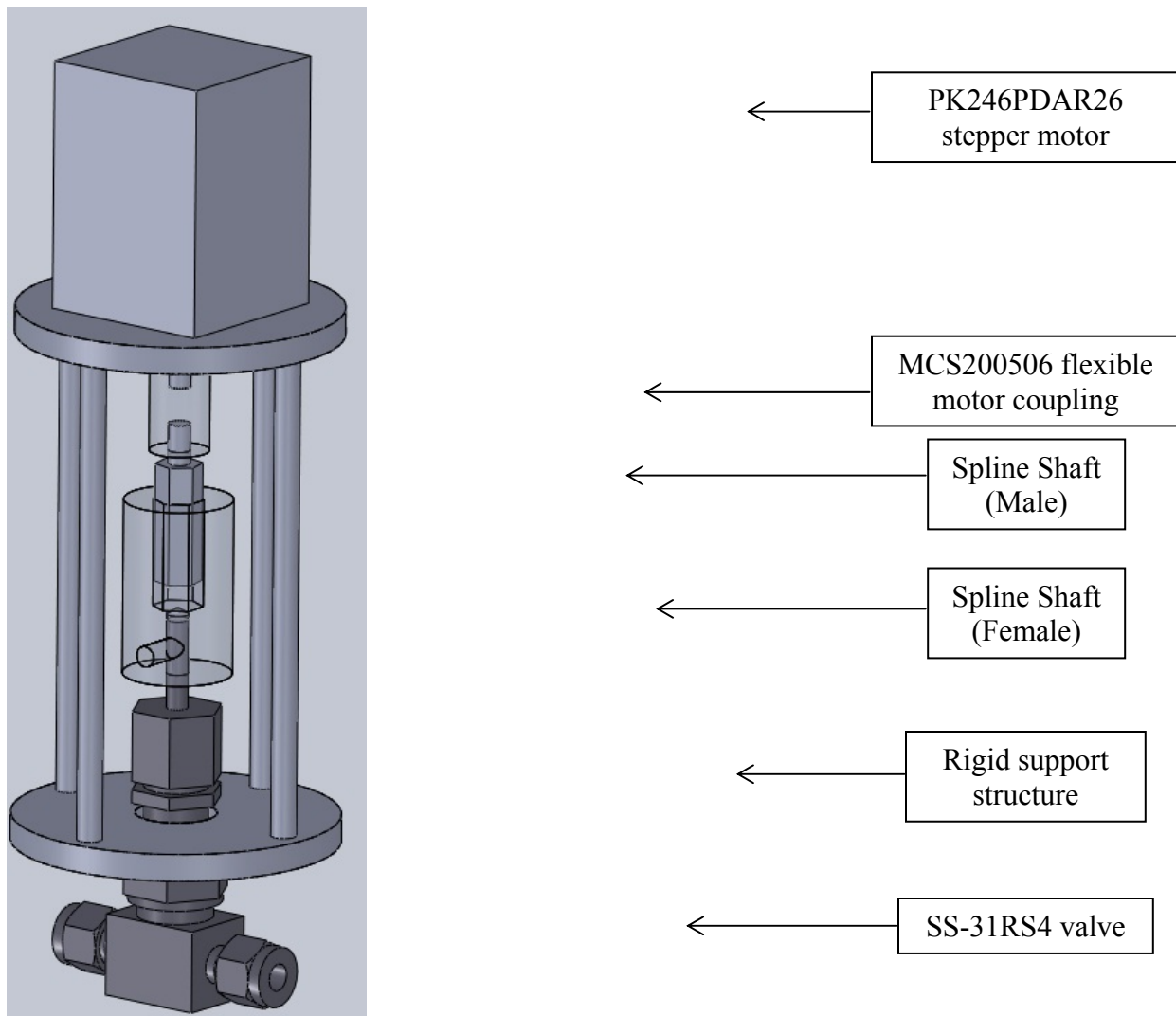
Figure 201 Automated valve which control test facility inlet pressure
