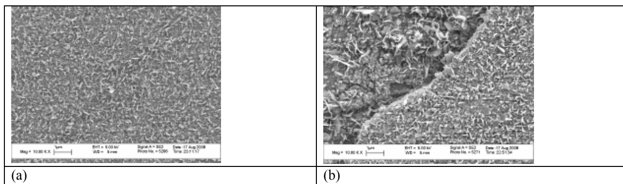
Figure 28: Surface morphology of alloy 625 after 1500 hours exposure (a) typical structure, and (b) sporadic spallation (<5%)
