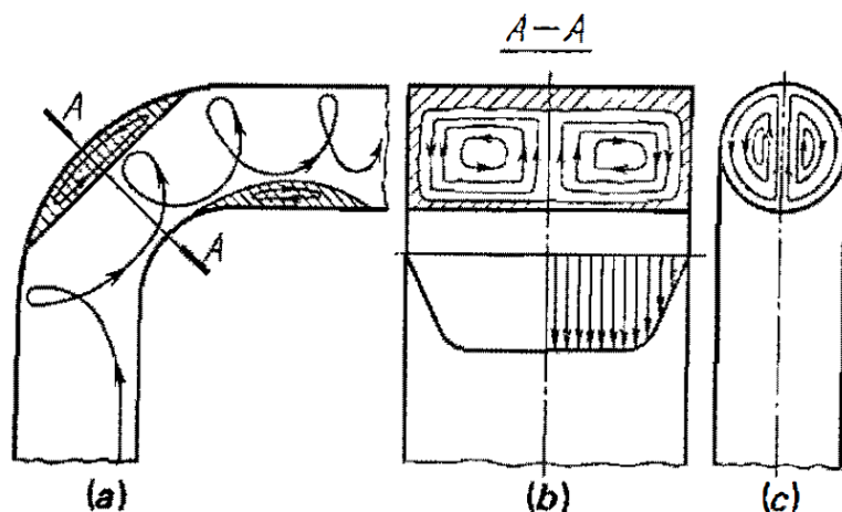
Figure 89: A diagram of the separation regions, swirling flow, and vortex pairing in a curved channel; from Idel'chik[16].
