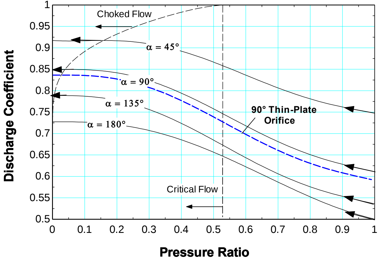
Figure 166 Conceptual basis for Standard Graph approach. The trend of the discharge coefficient of the prototype is estimated to be approximately equal to that of a planar element evaluated at a particular wall angle \alpha , k=1.4
