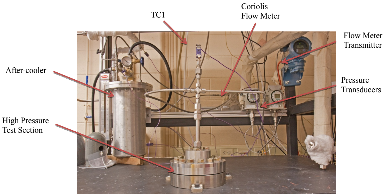
Figure 233 High pressure test section along with primary instrumentation
