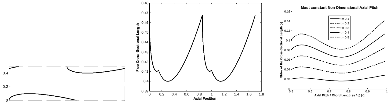
Figure 82: Left: A plane view of a sample airfoil fin channel and the resulting free cross-sectional length distribution along the flow axis. Right: A plot of the standard deviation of the free flow cross-sectional length distribution as a function of the ratios of airfoil thickness to chord length and axial pitch to chord length.
