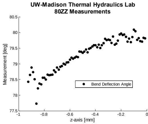
Figure 114: Bend deflection angle versus depth for the 80-degree zig-zag surface.
