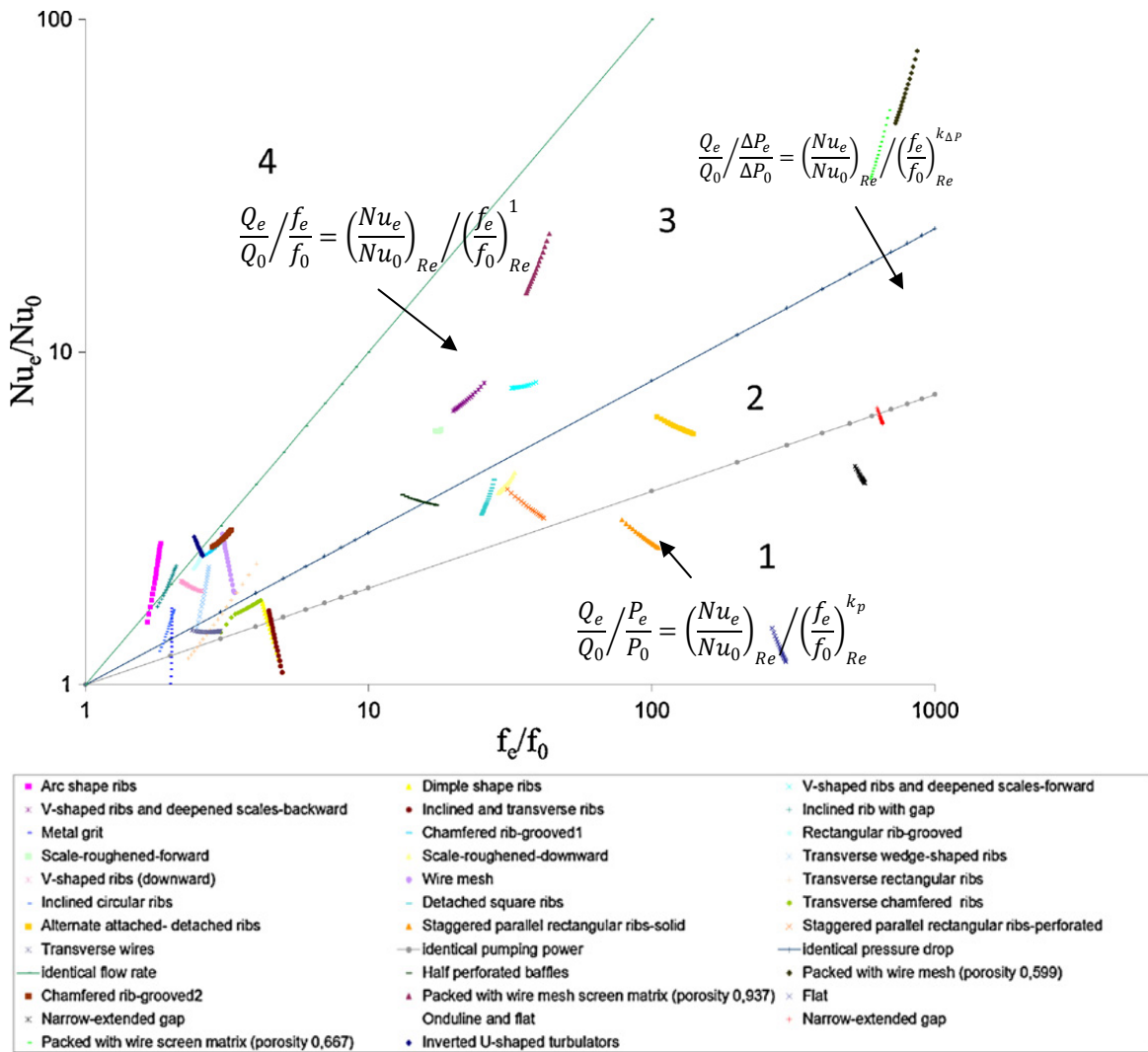
Figure 71: A comparison of the Nusselt number versus the Darcy friction factor scaled to the performance of flow between flat plates for a plate and frame heat exchanger, from Li et al. [33] (equations and arrows mine).
