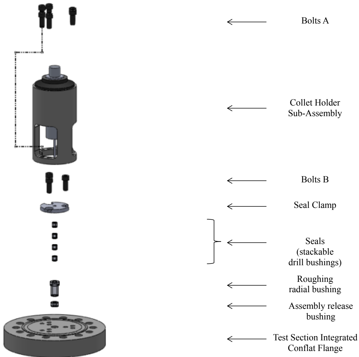
Figure 214 Assembly procedure of Shaft-Seal Sub-Assembly
