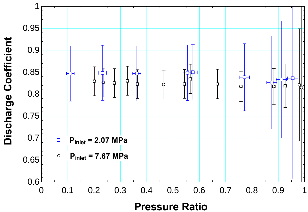
Figure 236 Discharge coefficient for measurements taken with an orifice at P_{\text{inlet}} = 2.07 \text{ MPa} and P_{\text{inlet}} = 7.67 \text{ MPa}
