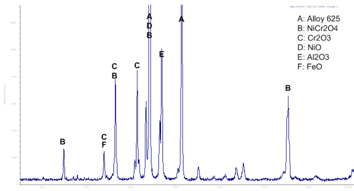
Figure 29: X-ray diffraction pattern of the surface oxide formed on Alloy 625 after 1500 hours exposure (a) typical structure, and (b) sporadic spallation (<5%)
