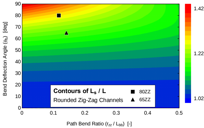
Figure 88: A plot of the contours of the length ratio for a rounded zig-zag channel path with the length ratios for the two zig-zag styles discussed in this work.
