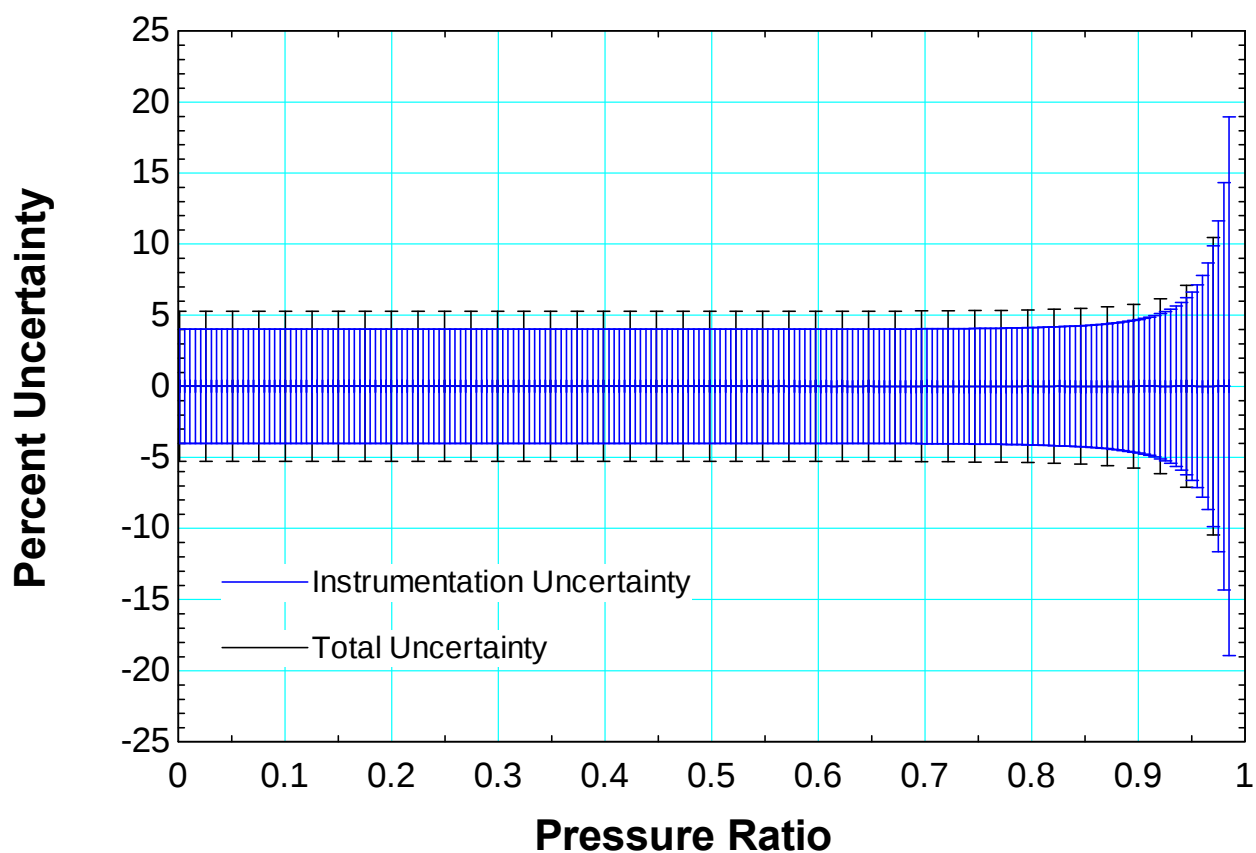
Figure 210 Percent uncertainty at nominal upstream test conditions of 7.6 MPa and 500 kg/m 3
