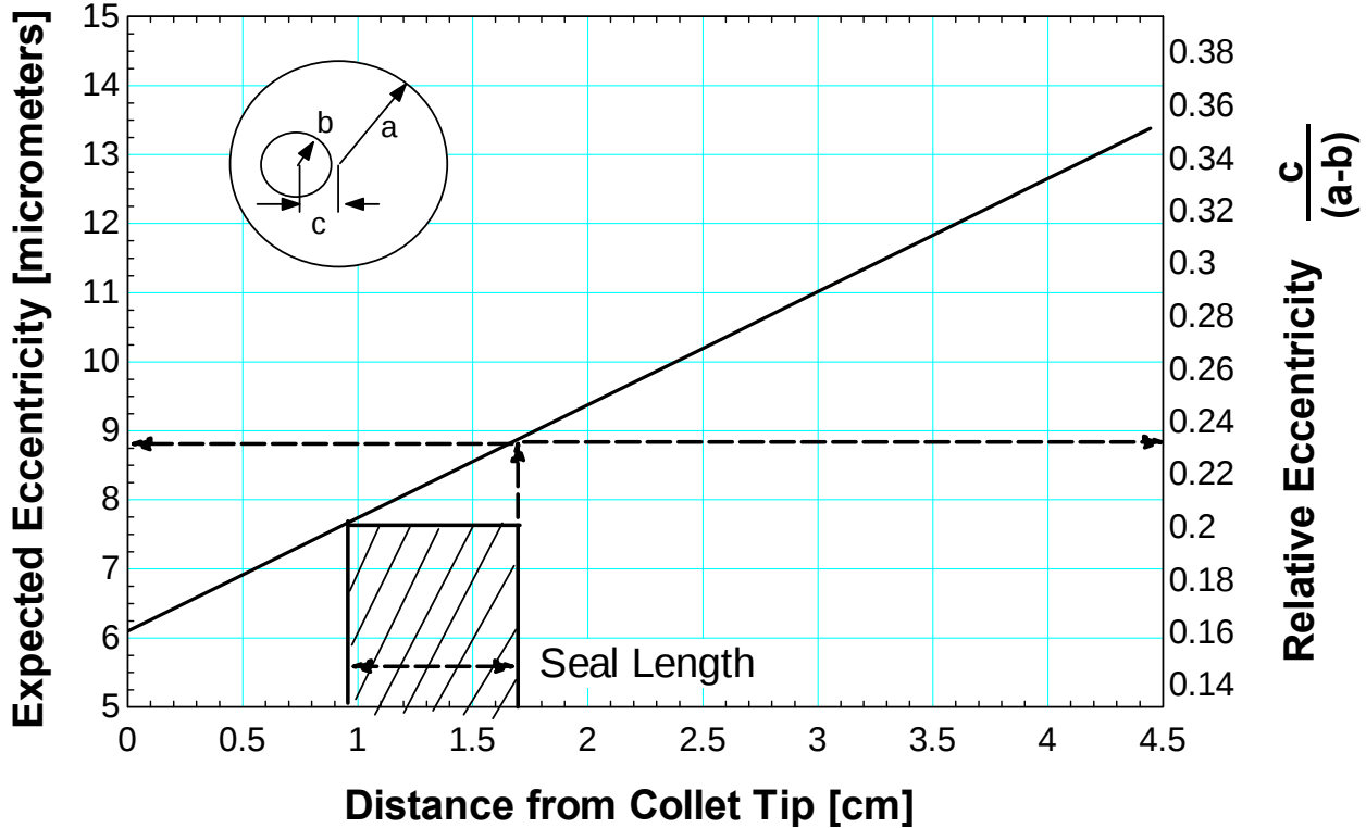
Figure 193 Expected eccentricity and relative eccentricity as a function of the distance from the collet tip.
