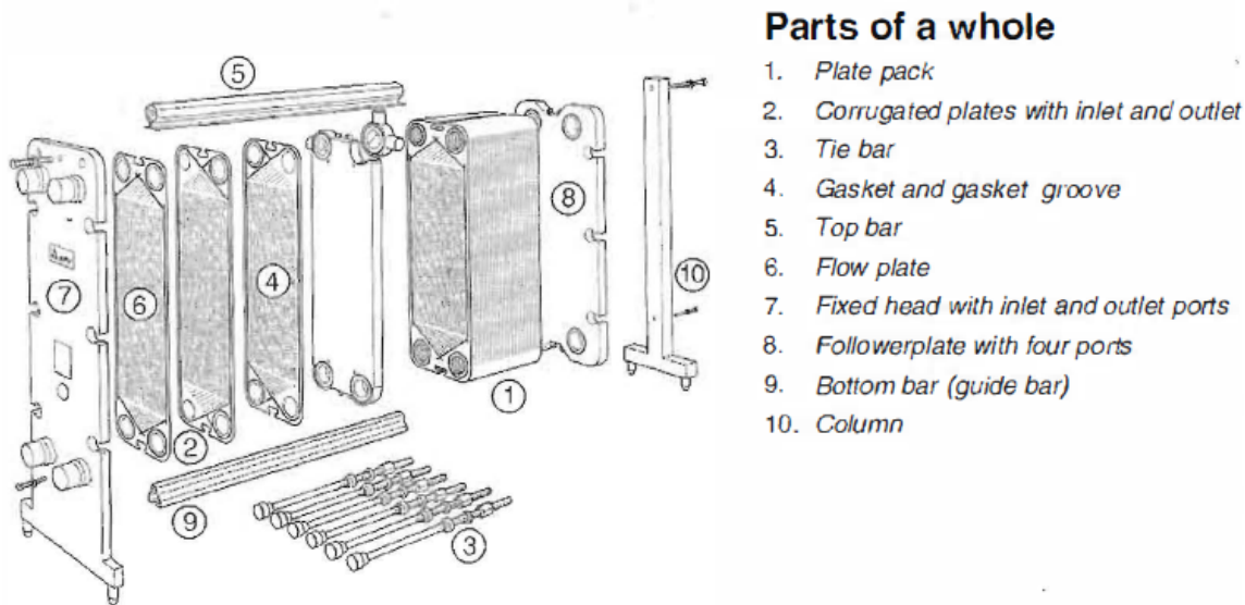
Figure 61: A diagram of a plate and frame heat exchanger from Hesselgreaves [6].
