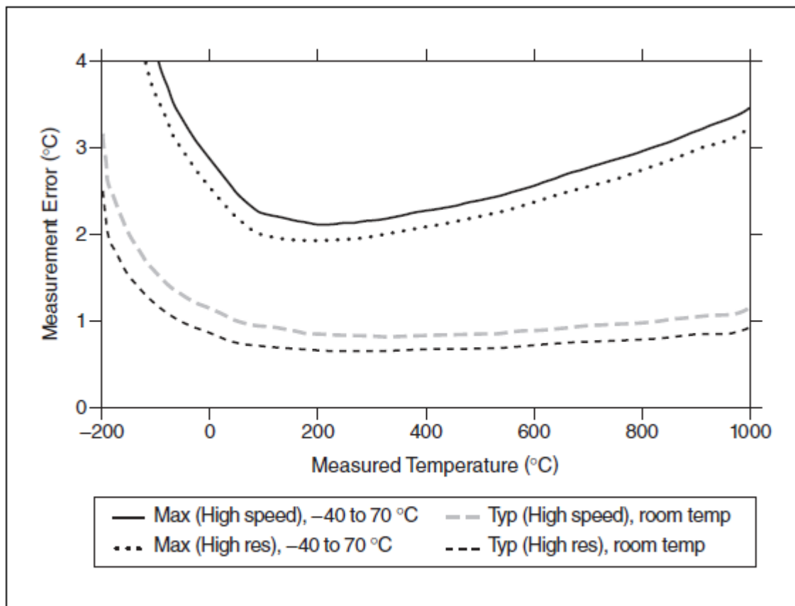
Figure 8. Thermocouple Types T and E Errors
