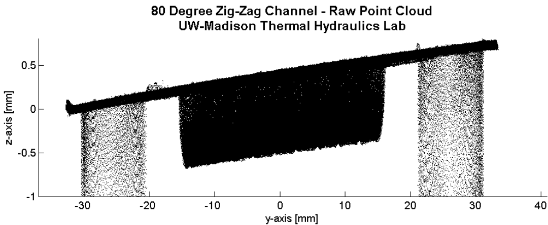
Figure 106: A YZ view of the raw point cloud data from the 80 degree zig-zag channel surface scan.
