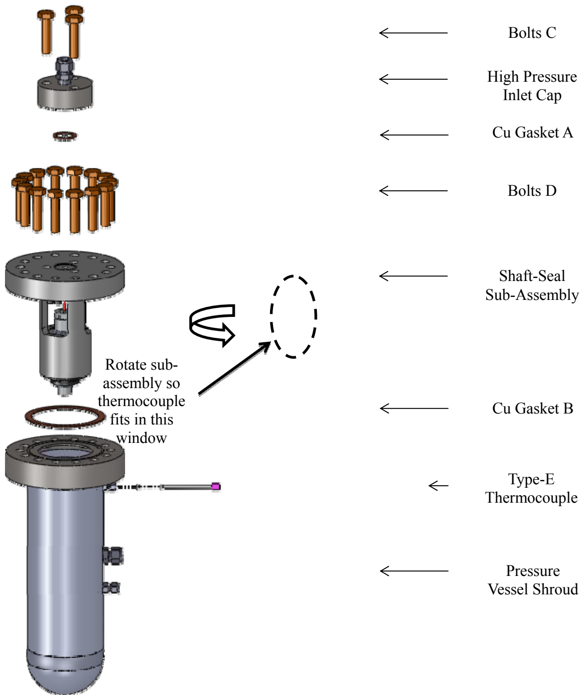
Figure 218 Final assembly procedure for configuring test section
