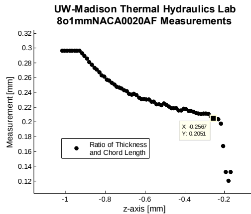
Figure 124: Ratio of thickness and chord length versus depth for the 8.1 mm NACA0020 surface.
