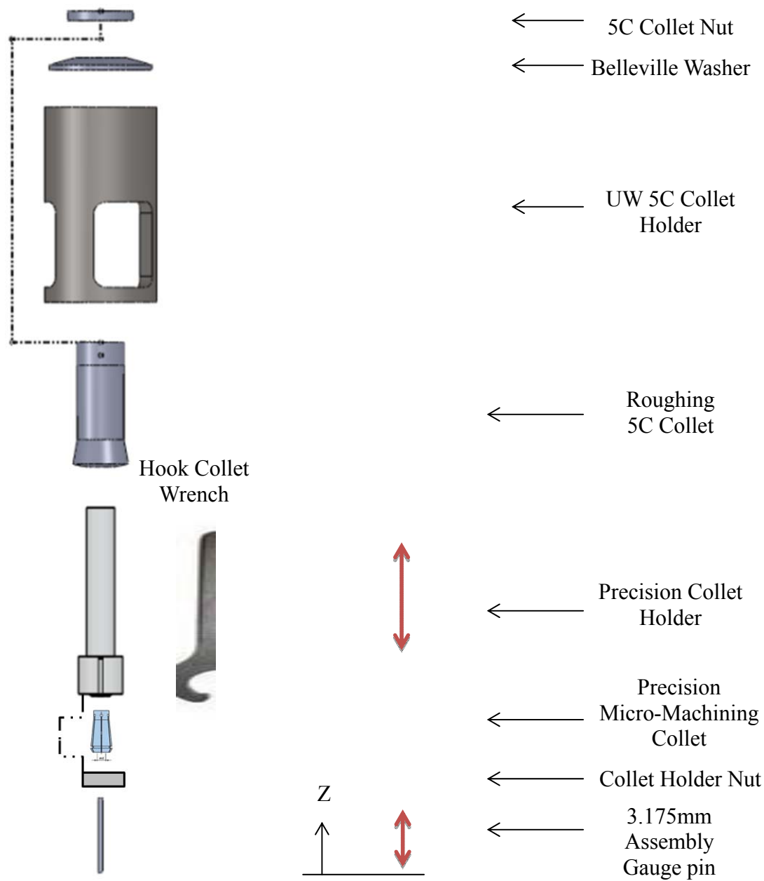
Figure 212 Assembly procedure of Collet Holder Sub-Assembly
