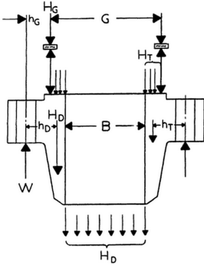
Figure 223 Illustration of critical parameters used to evaluate flanges by Bickford and Nassar (1998)
