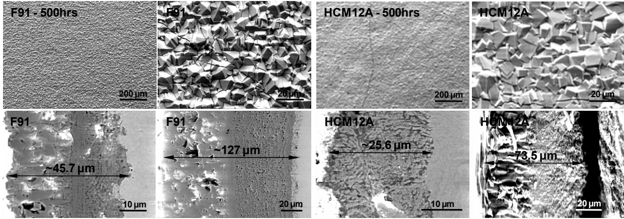
Figure 42: Surface morphologies and cross-section of the F91 and HCM12A samples exposed to the SC-CO 2 at 650°C for 500 hours.
