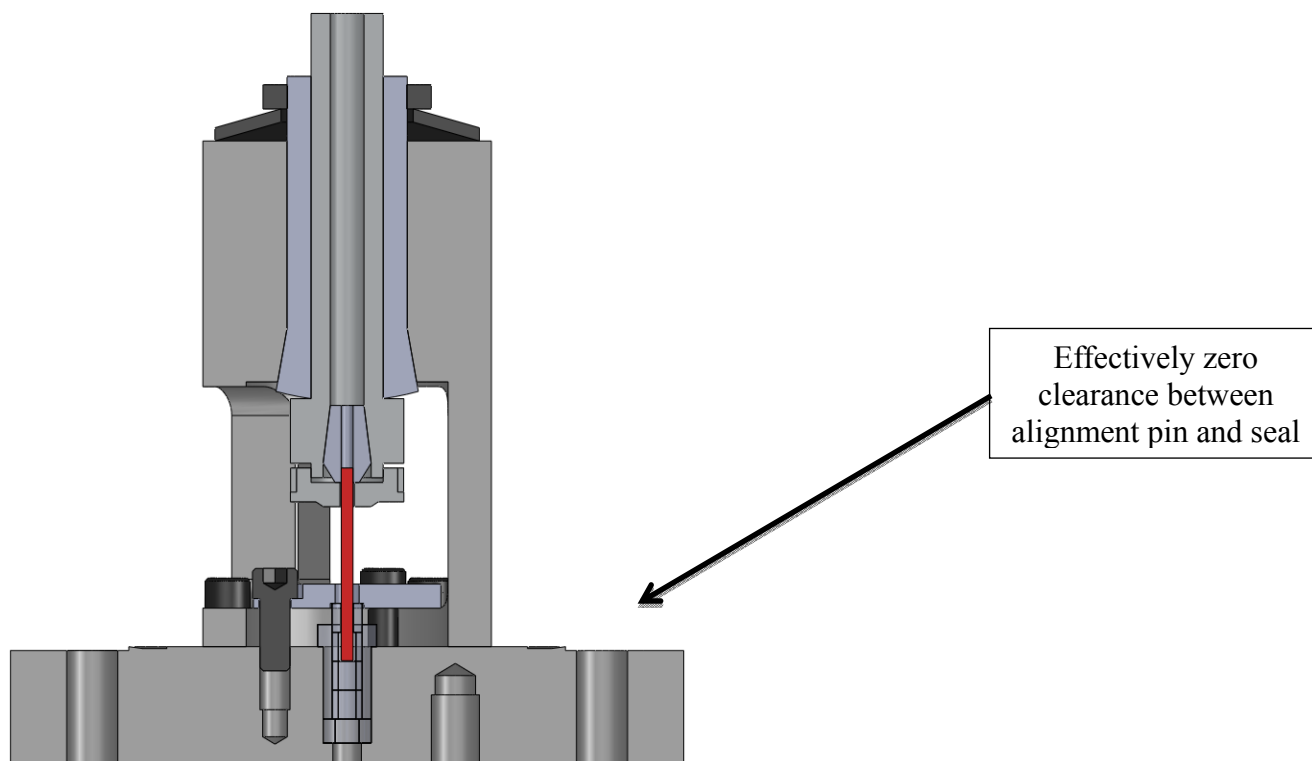
Figure 216 Shaft-Seal Sub-Assembly with 3.175mm gauge pin used to align multiple seals; shown here aligning only one seal
