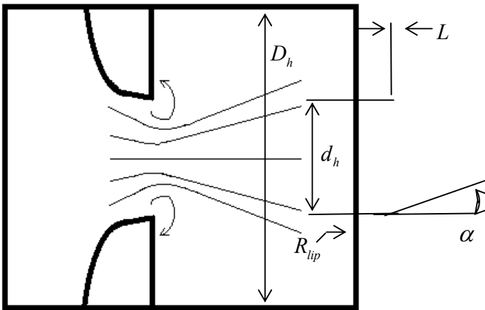
Figure 162 Geometrical properties related to critical discharge coefficient
