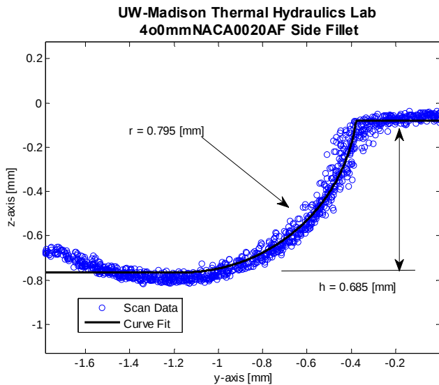
Figure 128: A plot of the averaged unit cell YZ slice at the widest section of the airfoil fit to the “StepFillet” function with the measured height and radius overlaid for the 4.0 mm NACA0020 surface.
