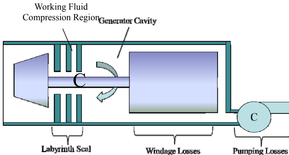
Figure 157 S-CO 2 compressor-generator assembly
