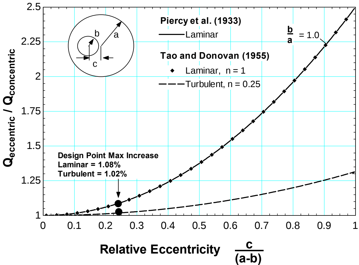
Figure 187 Flow rates through narrow eccentric annular gaps where b/a = 1 for both laminar and turbulent regimes; the results obtained from Piercy et al. (1933) and Tao and Donovan (1955) are reported.
