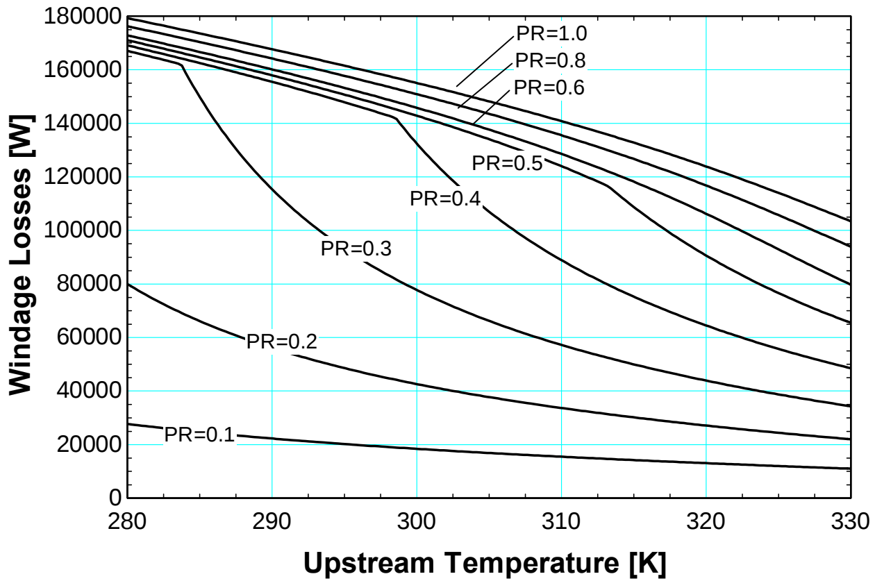
Figure 159 Calculated windage losses as a function of inlet temperature at different pressure ratios for the geometry shown in Table 4-2. The pressure ratio relates the cavity pressure to the compressor upstream pressure.
