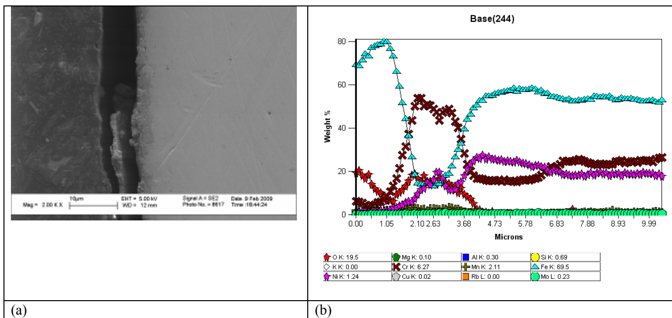
Figure 35: (a) SEM cross-sectional image of the oxide layer formed on 310 stainless steel after 1500 hours exposure and (b) the corresponding EDS compositional line-scan.
