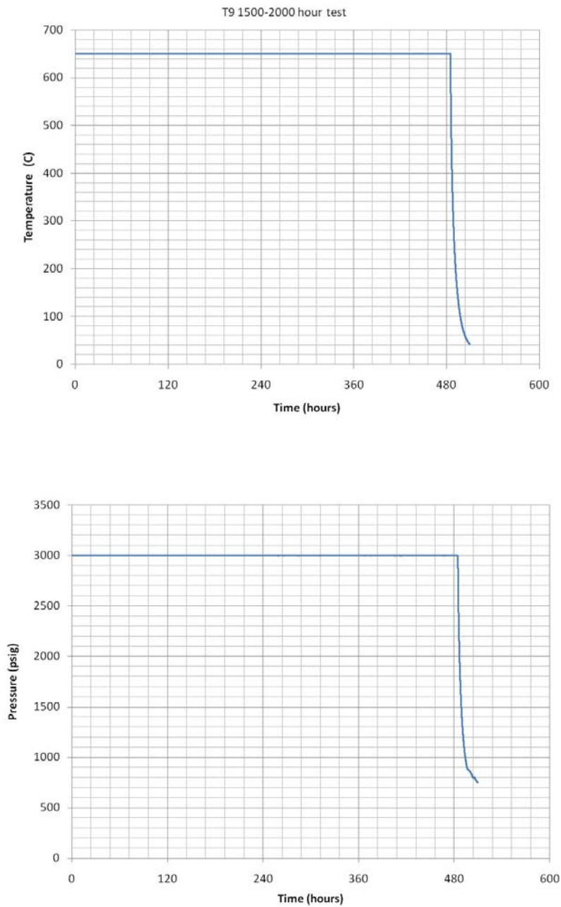
Figure 22 Temperature and pressure history for the 1500-2000 hour test duration
