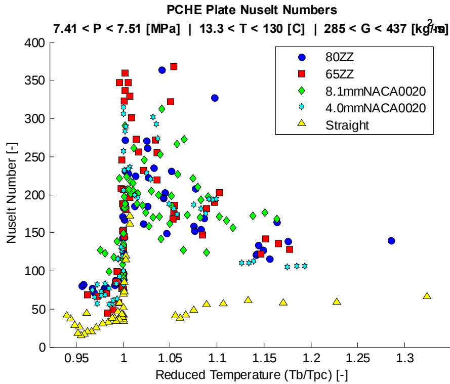
Figure 152: A combined comparison of the thermal performance of different PCHE channel geometries at a pressure of 7.5 MPa and a low mass flux.
