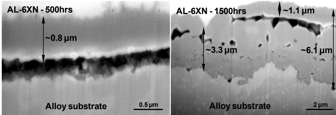
Figure 40: Secondary electron images of the cross-sectional alloy AL-6XN samples exposed to the S-CO 2 at 650°C for 500 and 1500 hours
