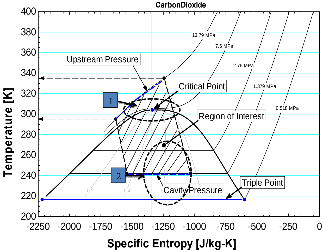
Figure 176 Test facility desired operating range
