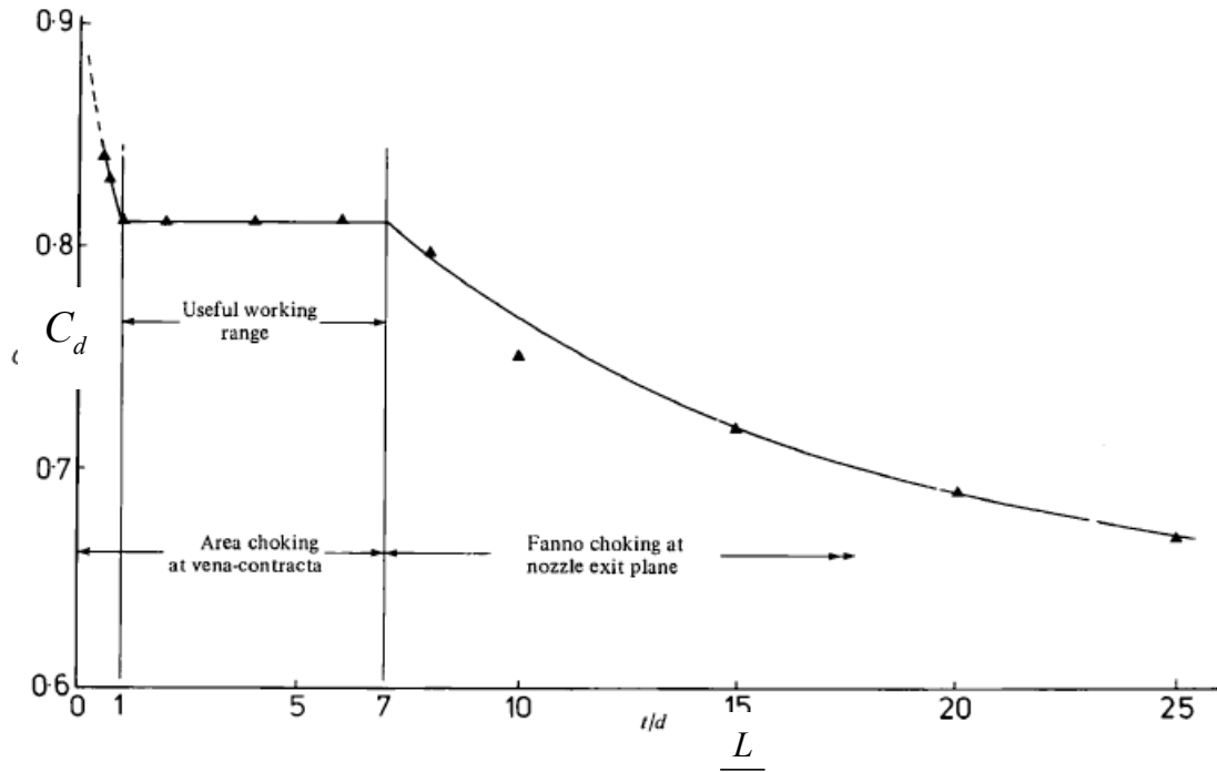
Figure 169 Functional relationship between discharge coefficient C_d and the ratio of the orifice length to the orifice diameter. Reproduced from Ward-Smith (1979).
