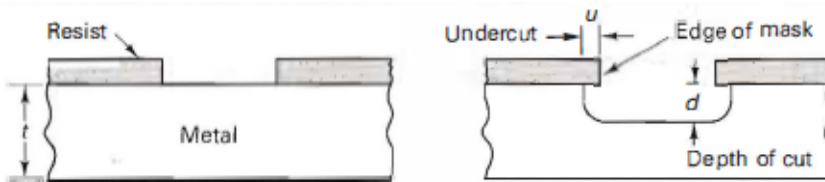
Figure 74: A diagram of the etch radius in photochemical machining from Black et al [36].
