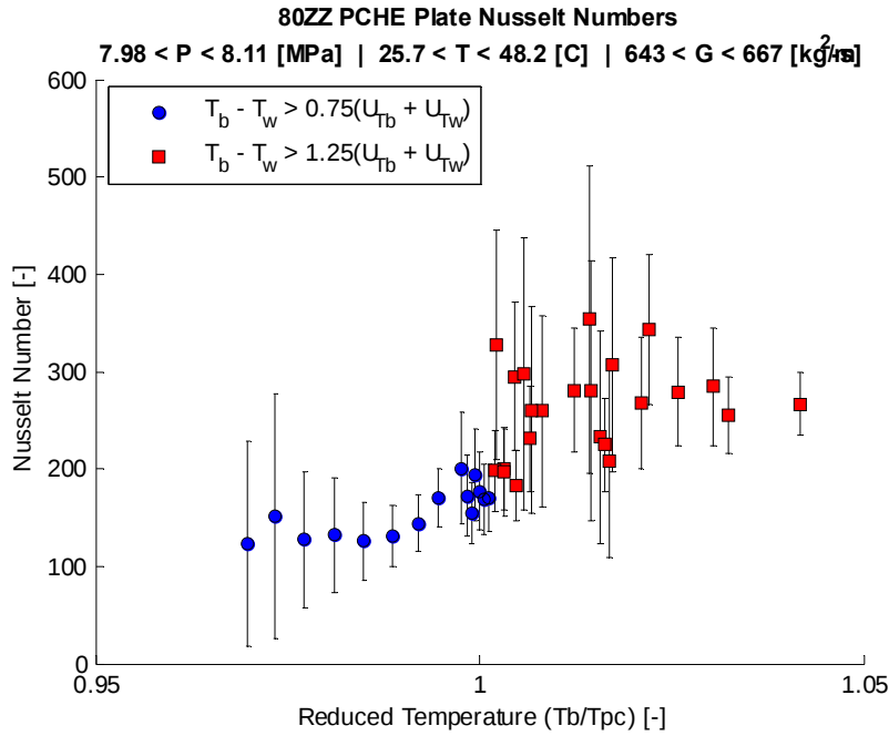
Figure 139: 80-degree zig-zag channel Nusselt number vs. reduced temperature at 8.1 MPa and high mass flux for cooling-mode flow using the measured geometry with error bars indicating propagated uncertainty.
