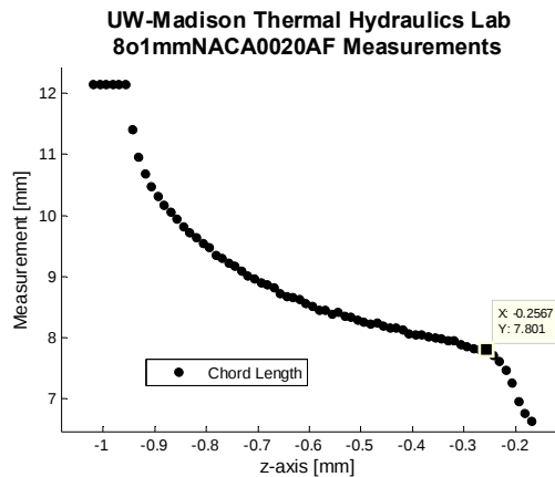
Figure 123: Measured chord length versus depth for the 8.1 mm NACA0020 surface.
