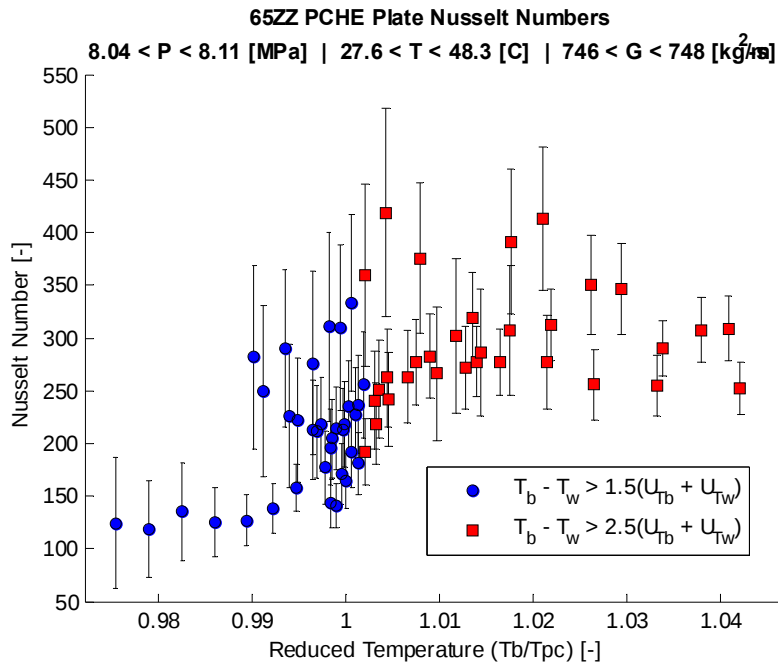
Figure 140: 65-degree zig-zag channel Nusselt number vs. reduced temperature at 8.1 MPa and high mass flux for cooling-mode flow using the measured geometry with error bars indicating propagated uncertainty.
