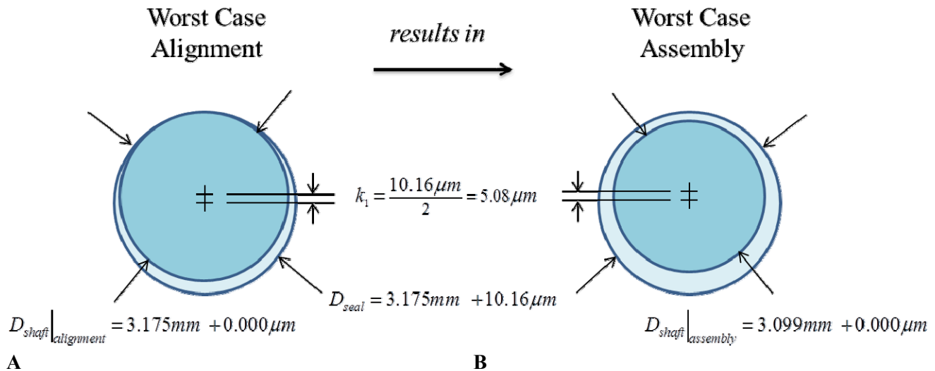
Figure 191 Shaft to seal alignment and final assembly process demonstrations; A – alignment pin used to center shaft and seal assembly; B – final assembled position of shaft and seal
