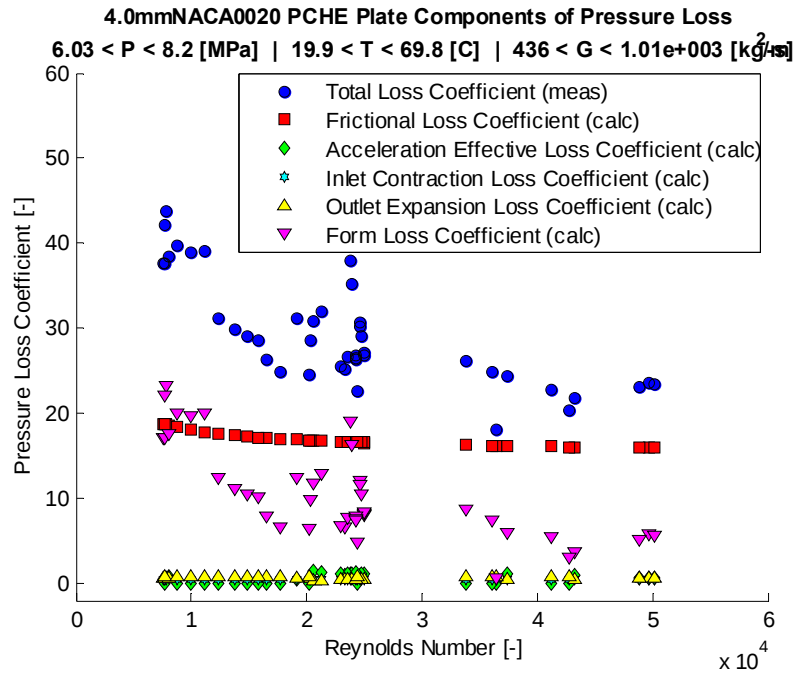
Figure 144: 4.0 mm NACA0020 airfoil fin channel calculated pressure loss components using the measured geometry. Note that calculated acceleration, inlet contraction, and outlet expansion points are approximately the same and overlap.
