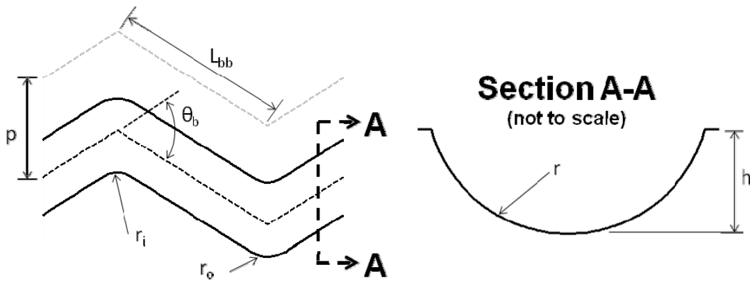
Figure 111: A diagram for an arbitrary rounded zig-zag PCHE channel unit cell.
