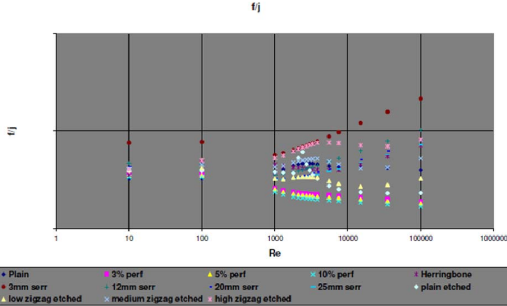
Figure 68: A plot of the ratio of the fanning friction factor (shown temporarily as f ) and the Colburn j factor of several PFHE and PCHE surfaces, from Southall et al. [40].
