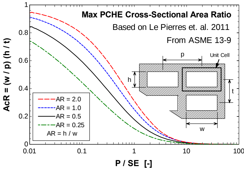
Figure 87: A plot of the maximum possible cross-sectional area ratio as a function of pressure containment ratio for several aspect ratio PCHE channels.
