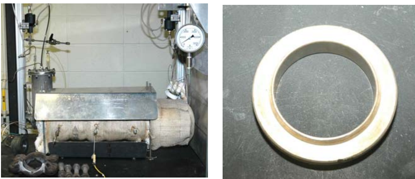
Figure 9 (Left) Photograph of the insulated autoclave with one end of the Grayloc fittings removed for sample insertion. Figure 2.8 (Right) Photograph of seal ring for Grayloc end cap
