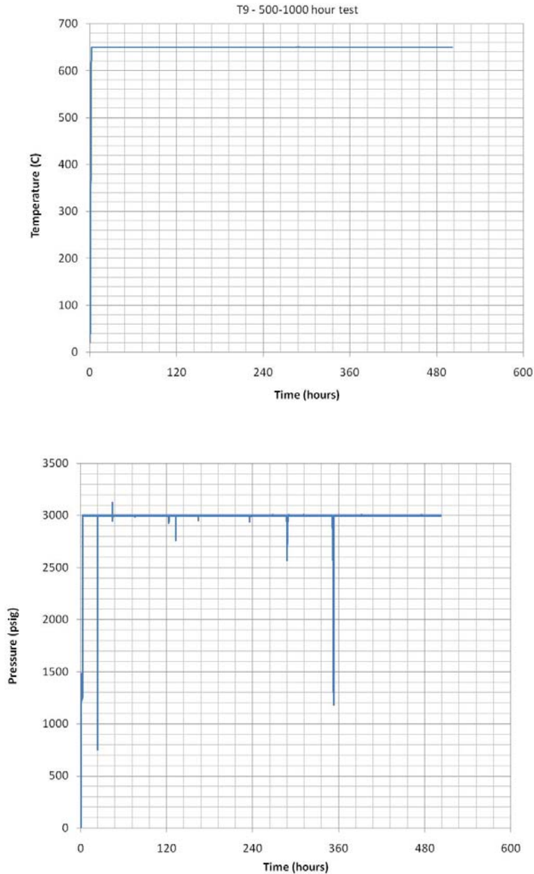
Figure 20 Temperature and pressure history for the 500-1000 hour test duration
