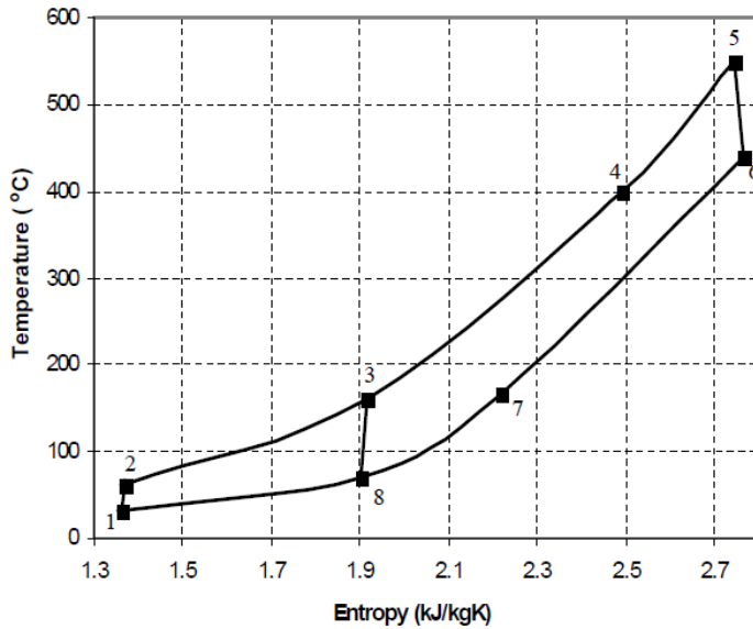
Figure 48: A T-s diagram for the recompression SCO 2 cycle from Dostal [4].
