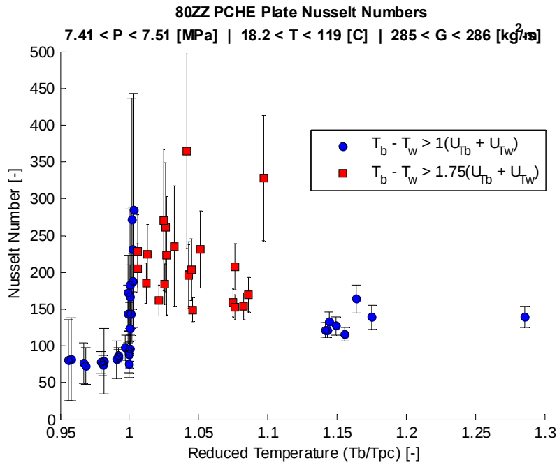
Figure 135: 80-degree zig-zag channel Nusselt number vs. reduced temperature at 7.5 MPa and low mass flux for cooling-mode flow using the measured geometry with error bars indicating propagated uncertainty.
