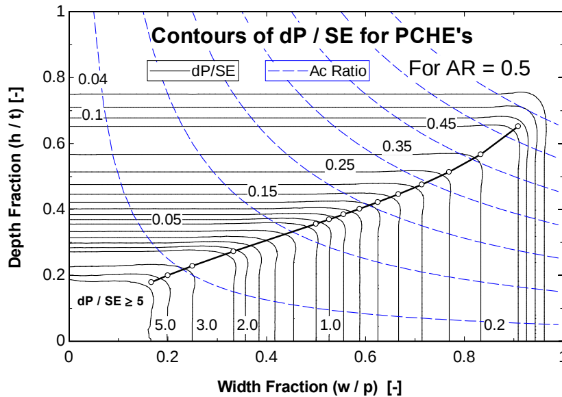
Figure 86: A plot of contours of the pressure containment ratio as a function of width fraction and depth fraction for an aspect ratio of 0.5, with lines of constant area ratio overlaid. The maximum pressure containment ratio as a function of cross-sectional area ratio is also shown by the connected open circles.
