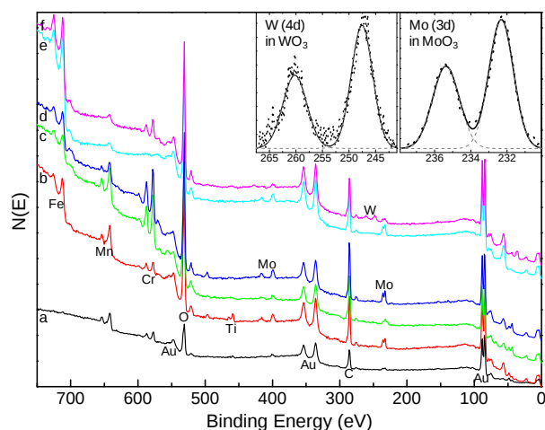
Figure 44: XPS spectra of the surfaces of the SC-CO 2 exposed samples: a) 800H/500 hours, b) 800H/1500 hours, c) AL-6XN/500 hours, d) AL-6XN/1500 hours, e) F91/500 hours, and f) HCM12A/500 hours. The high-resolution spectra of Mo 3d (from d) and W 4d (from f) are shown as insets. Gold (Au) was used as a standard for the spectra.
