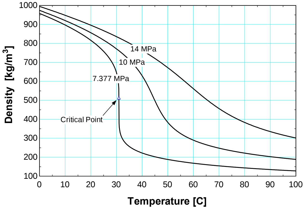
Figure 172 Thermodynamic property variation of carbon dioxide near the critical point
