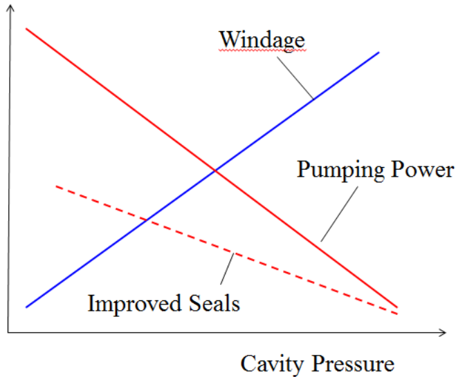
Figure 158 Conceptual interpretation of natural tradeoff in system demonstrating the effect of cavity pressure on overall power reduction
