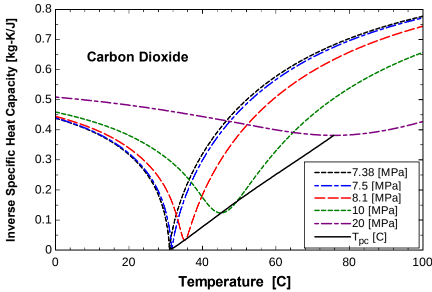
Figure 52: A plot of the inverse of specific heat versus temperature of carbon dioxide with several isobars and the pseudo-critical line shown.
