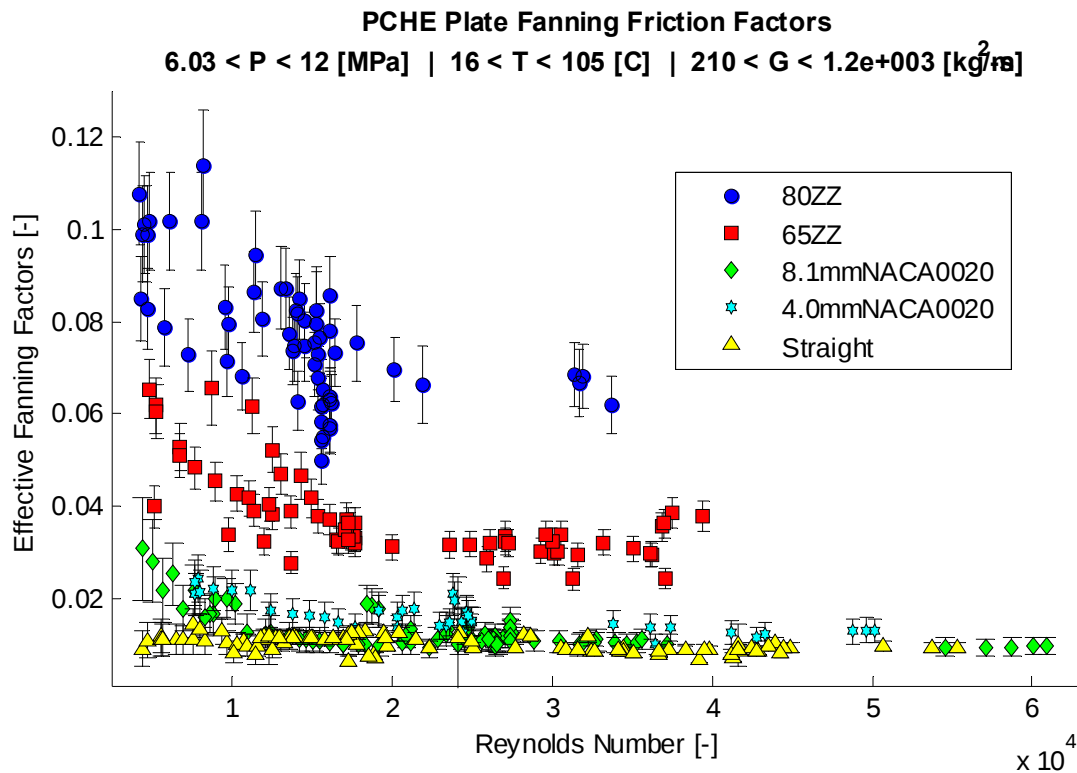
Figure 151: A combined comparison of the hydraulic performance of different PCHE channel geometries using the effective Fanning friction factor based on the total pressure drop and the channel path length.
