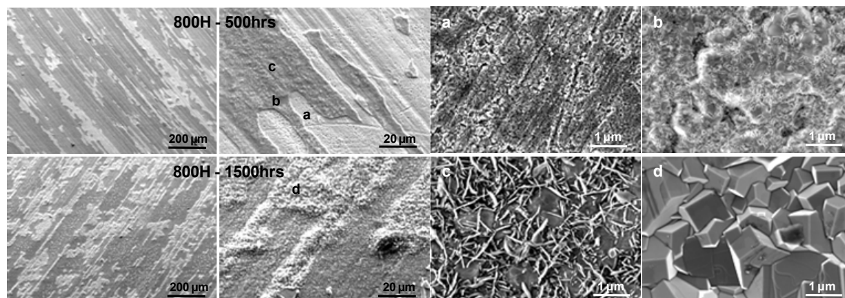
Figure 37: Surface morphologies of the alloy 800H samples exposed to the S- \text{CO}_2 at 650C for 500 and 1500 hours. The detailed morphologies of the features labeled with a-d are shown in the secondary electron images on the right.
