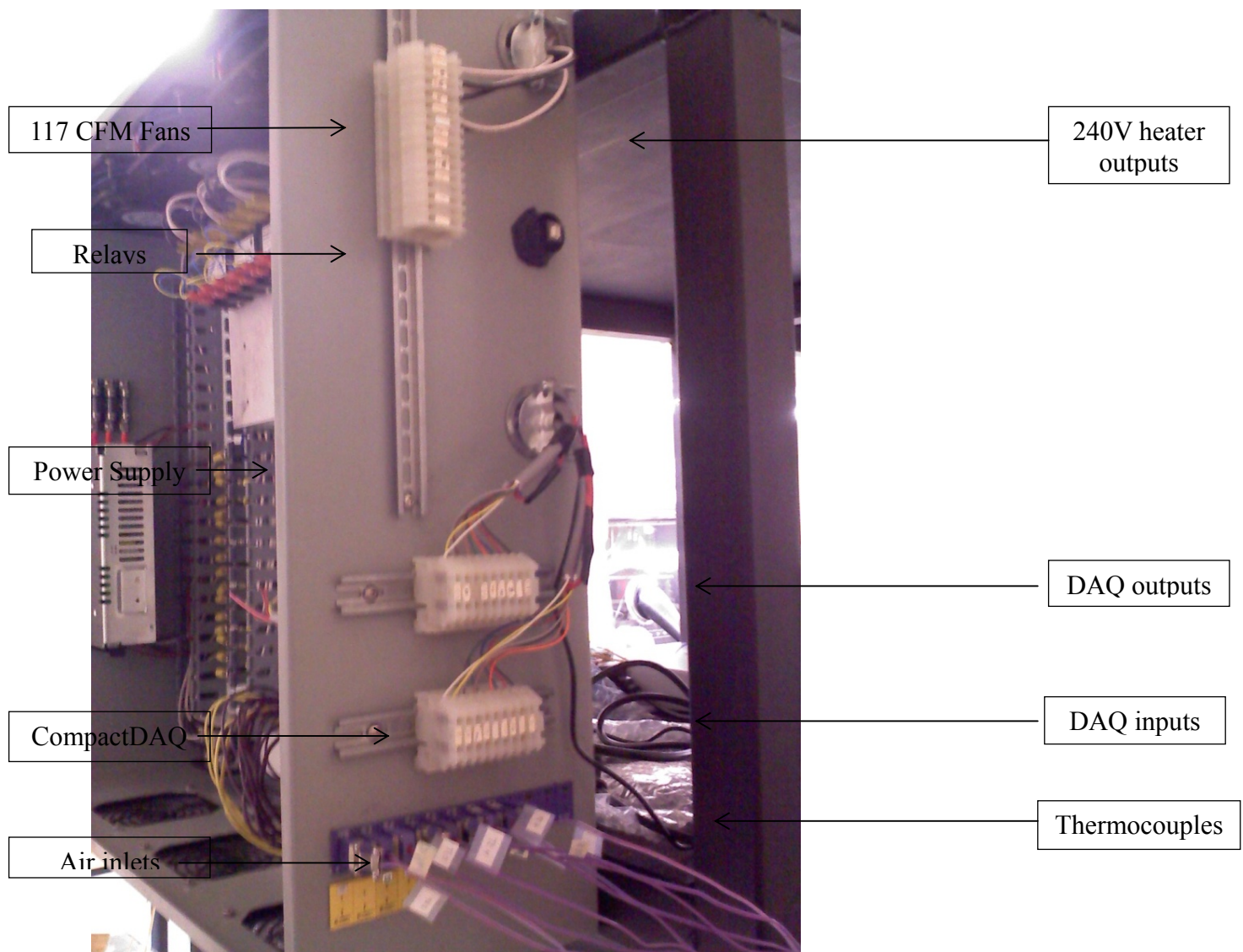
Figure 204 Safety and instrumentation panel box
