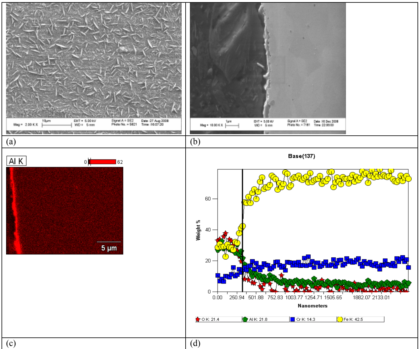
Figure 33: (a) SEM-EDS analysis of the oxide layer formed on PM2000 after exposure for 1500 hours, (a) plan view, (b) cross-sectional view, (c) x-ray mapping showing Al-rich oxide layer, and (d) EDS line scan confirming an Al-rich oxide layer.
