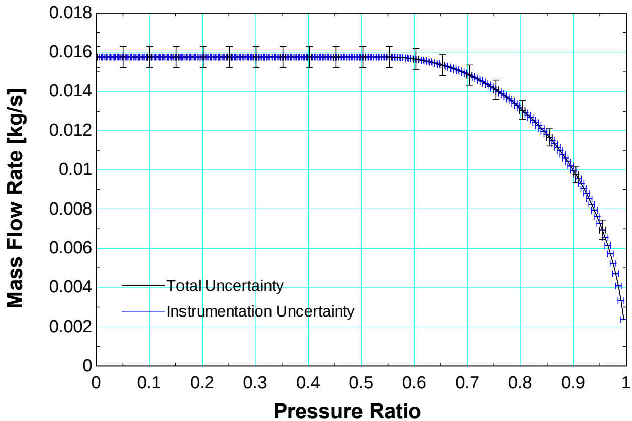
Figure 209 Uncertainty at nominal upstream test conditions of 7.6 MPa and 500 kg/m 3
