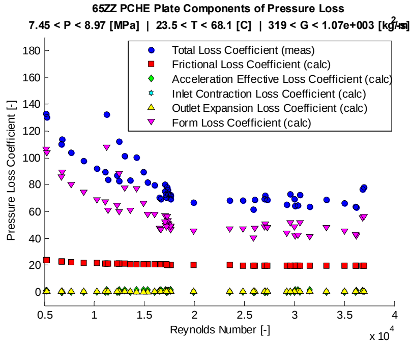
Figure 133: 65-degree zig-zag channel calculated pressure loss components using the measured geometry. Note that calculated acceleration, inlet contraction, and outlet expansion points are approximately the same and overlap.
