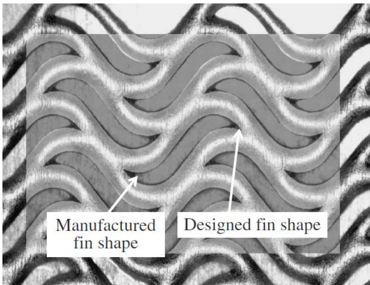
Figure 76: A plan view of the s-shaped fin PCHE surface investigated by Tsuzuki et al. [48] showing in particular the rounding effect of the etch factor on the sharp-designed leading and trailing edges of the fin.
