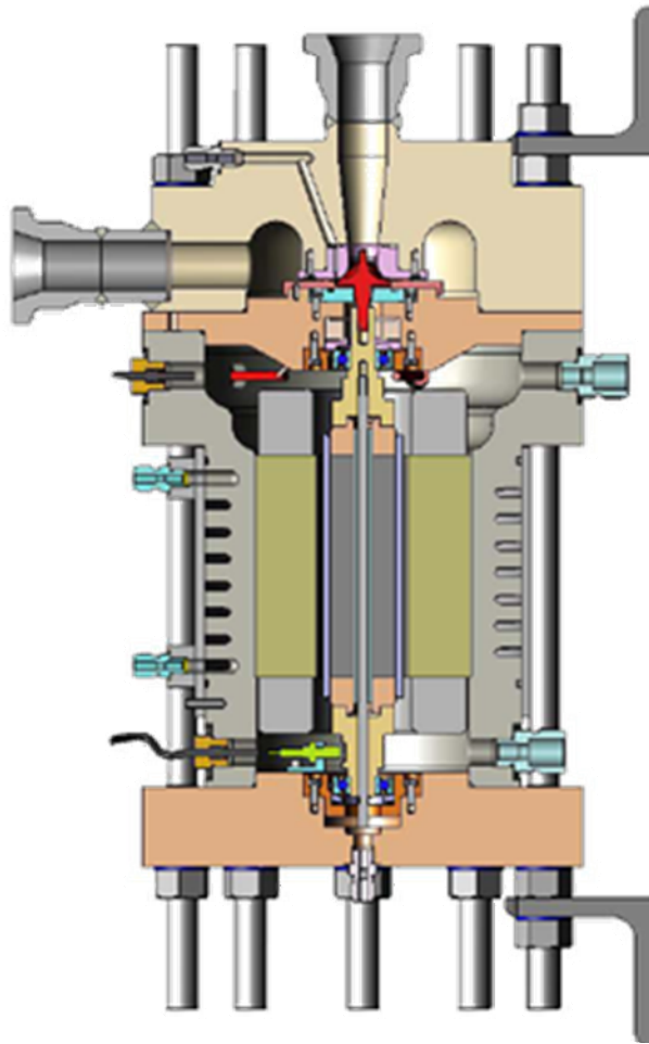
Figure 160 Supercritical carbon dioxide brayton cycle developed by Sandia National Laboratory and Barber-Nichols. (a) Assembled version of S-CO 2 cycle (b)
