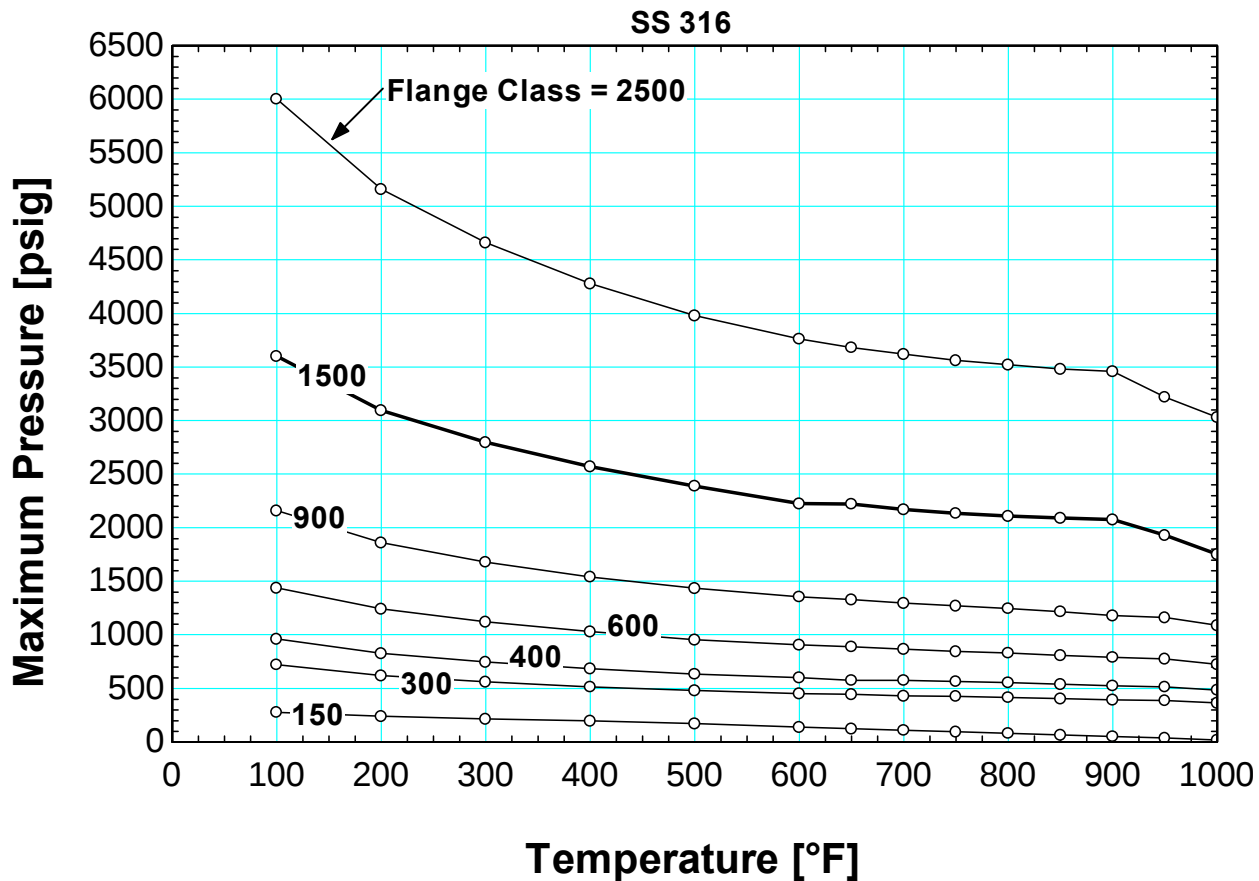
Figure 222 ASME SS 316 flange rating for different flange classes based on temperature
