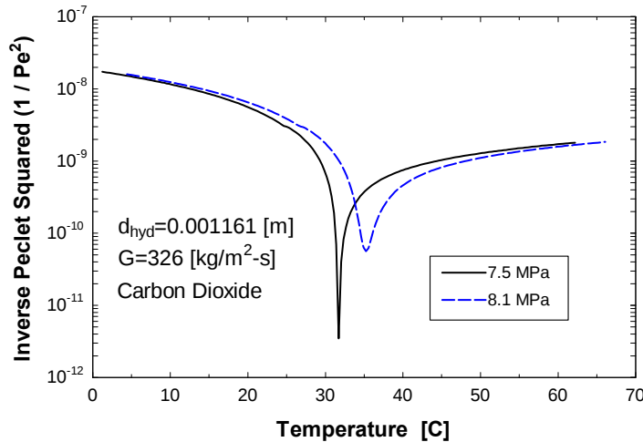
Figure 57: The variation in the squared inverse of the Peclet number vs. temperature at several pressures.
