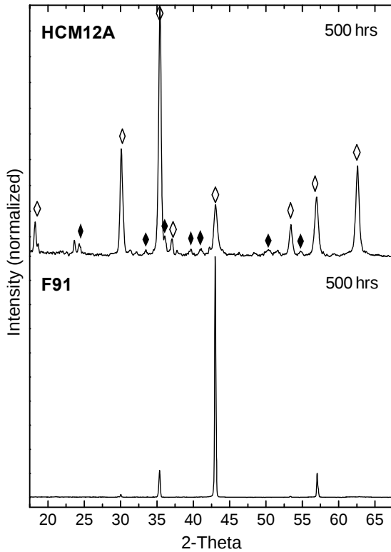
Figure 43: X-ray diffraction patterns of the F91 and HCM12A samples exposed to the SC-CO 2 at 650°C for 500 hours. The symbols ◇ and ♦ denote magnetite (e.g. Fe 3 O 4 [19-629]) and chromium oxide (e.g. Cr 1.3 Fe 0.7 O 3 [35-1112]), respectively. The unlabeled peaks in the HCM12A pattern correspond to tungsten oxide (e.g. WO 3 [01-089-8052]).
