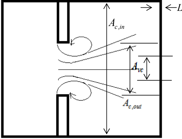
Figure 163 Ratio between the cross-sectional areas of the orifice to that of the vena contracta.
