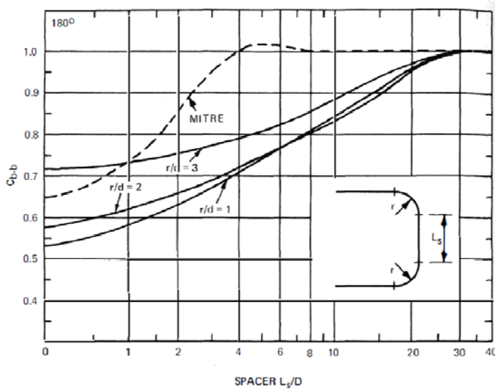
Figure 95: A chart of the bend-bend correction factor for use with low aspect ratio rectangular channels, from Miller [12]. For zig-zag PCHE channels the spacer length ratio L_s / D is the ratio of the zig-zag bend length to the channel width L_{bb} / w , while the bend radius ratio r / d is the ratio of the bend radius to the channel width r / w .
