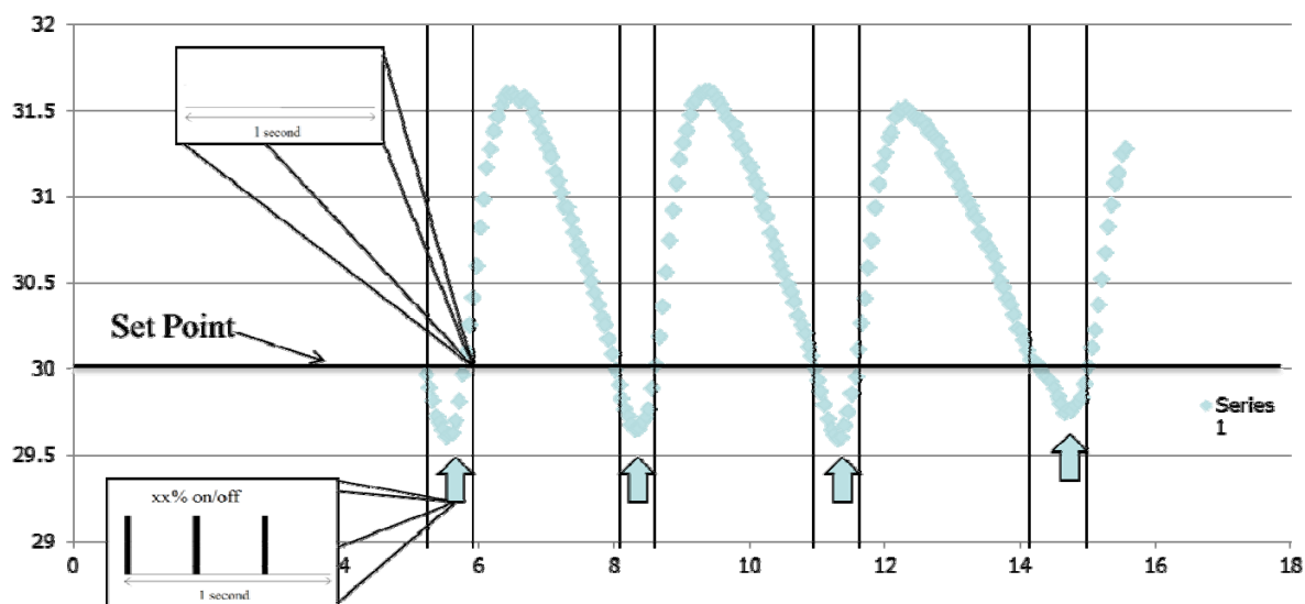
Figure 206 Description of PID operated heaters
