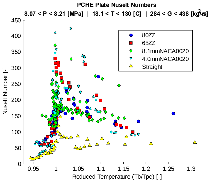
Figure 153: A combined comparison of the thermal performance of different PCHE channel geometries at a pressure of 8.1 MPa and a low mass flux.
