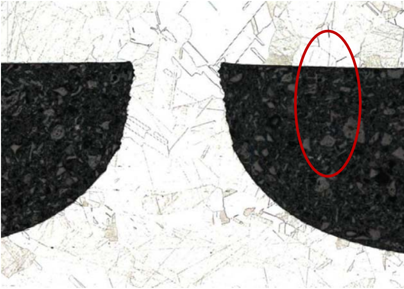
Figure 75: A micrograph of a Heatic PCHE plate section showing the smooth roundness of the bottom of the channel indicative of undercutting as well as a rougher area near the top of the fin likely due to compression during diffusion bonding, from Southall [47].
