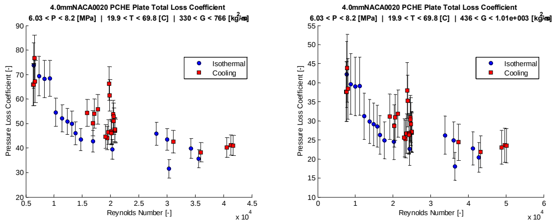
Figure 142: 4.0 mm NACA0020 total loss coefficient vs. Reynolds number for cooling-mode flow using the design and measured geometry respectively with error bars indicating propagated uncertainty.
