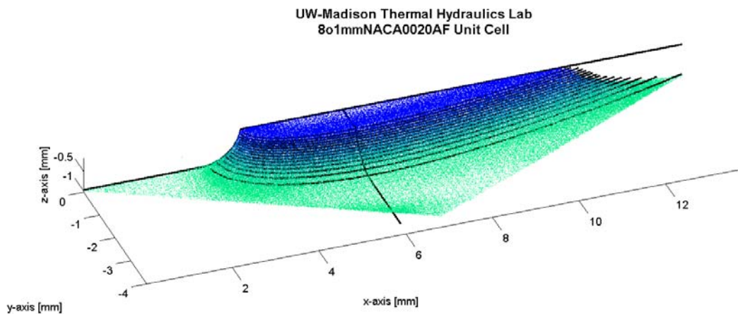
Figure 121: The 8.1mm NACA0020 unit cell point cloud shaded from blue near the plate surface to green at the bottom of the channel, and with several depth-wise and step fillet cutting plane fit curves shown in black.
