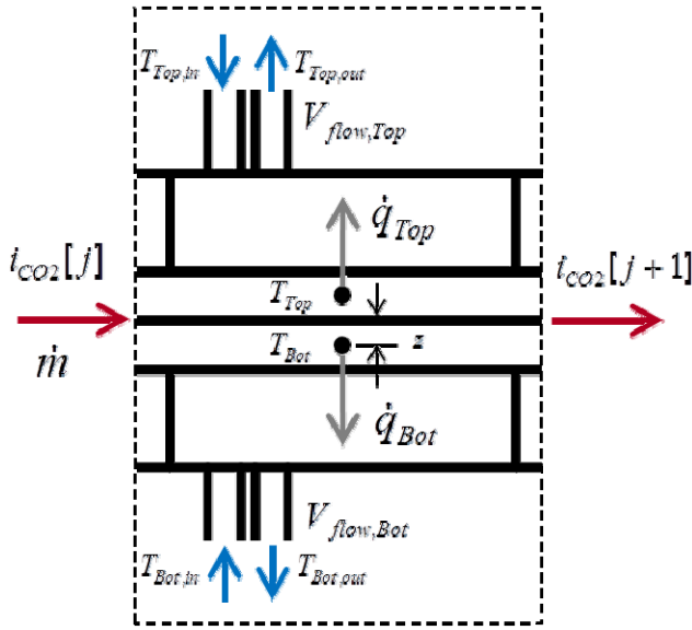
Figure 129: Diagram of the heat transfer coefficient calculation for each cooling block section.
