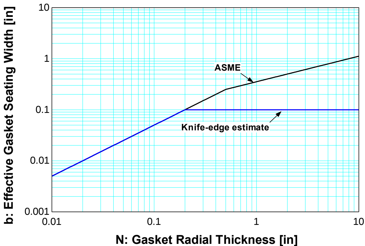
Figure 224 Effective gasket seating width based on ASME specification and new design shown with knife-edge estimate
