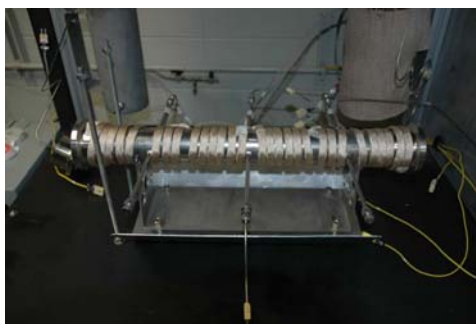
Figure 7 Photograph of the end of the autoclave system where the samples are inserted
