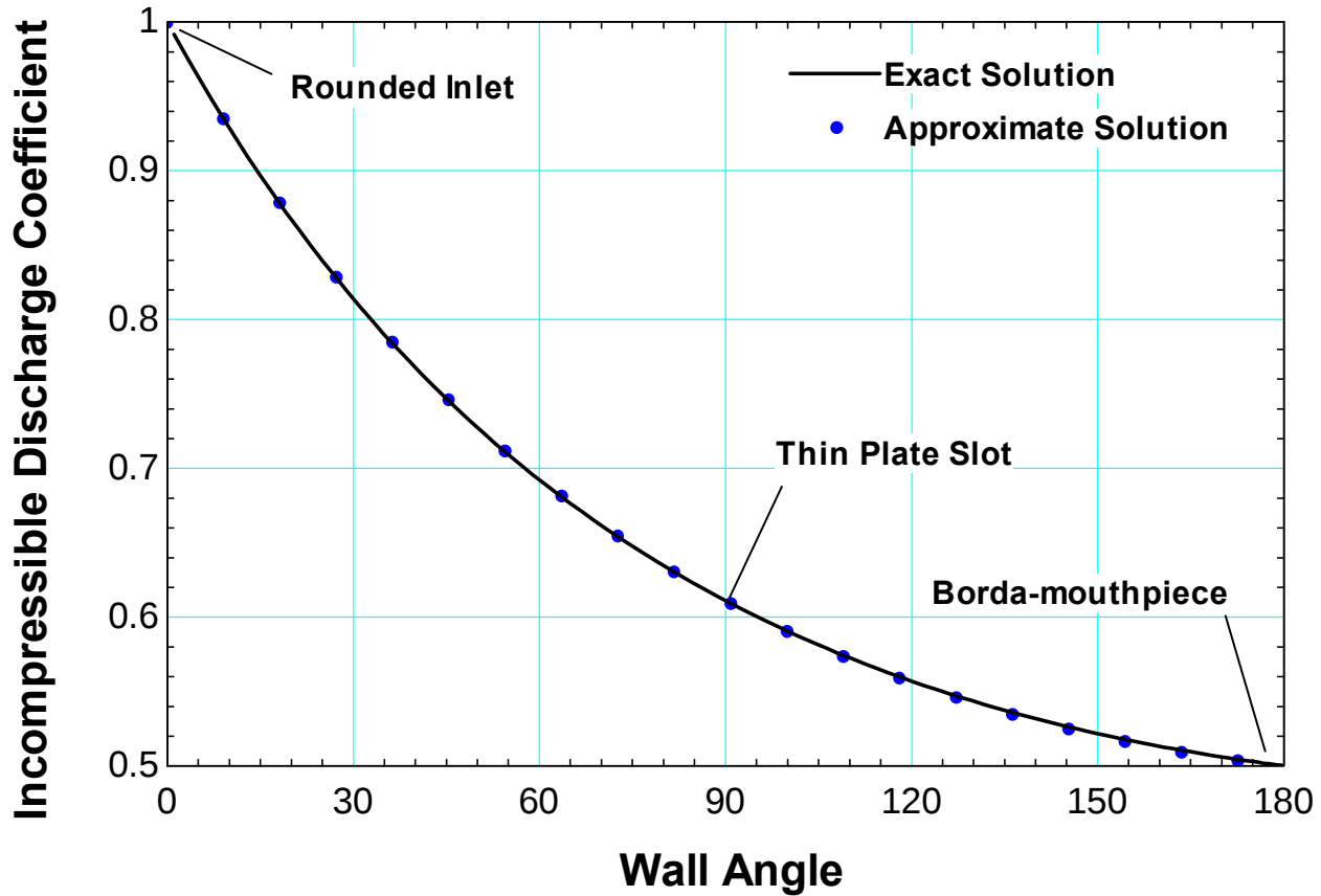
Figure 165 Discharge coefficient for PR=1 as a function of wall angle \alpha for planar flow; basis for Standard Graph approach, k=1.4
