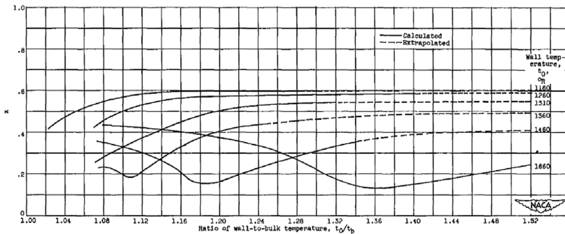
Figure 59: A plot of weighting factor x versus the ratio of wall and bulk temperature, where x is defined by T(x) = x (T_w - T_b) + T_b , for the friction factor of water at a pressure of 5000 psi from Deissler and Taylor [30].
