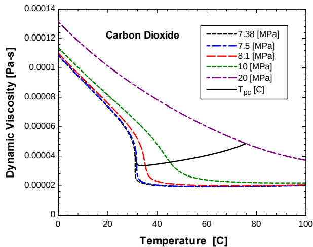
Figure 55: A plot of the dynamic viscosity versus temperature of carbon dioxide with several isobars and the pseudo-critical line shown.
