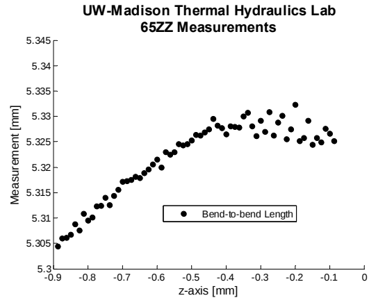
Figure 117: Bend-to-bend length versus depth for the 65-degree zig-zag surface.
