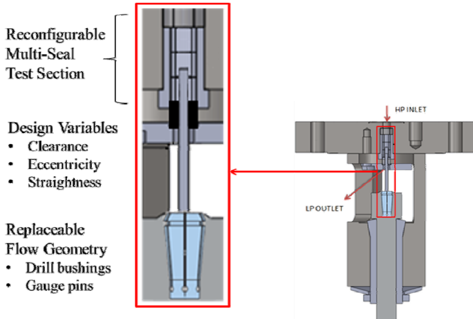
Figure 211 Design variables considered in the design of the test section
