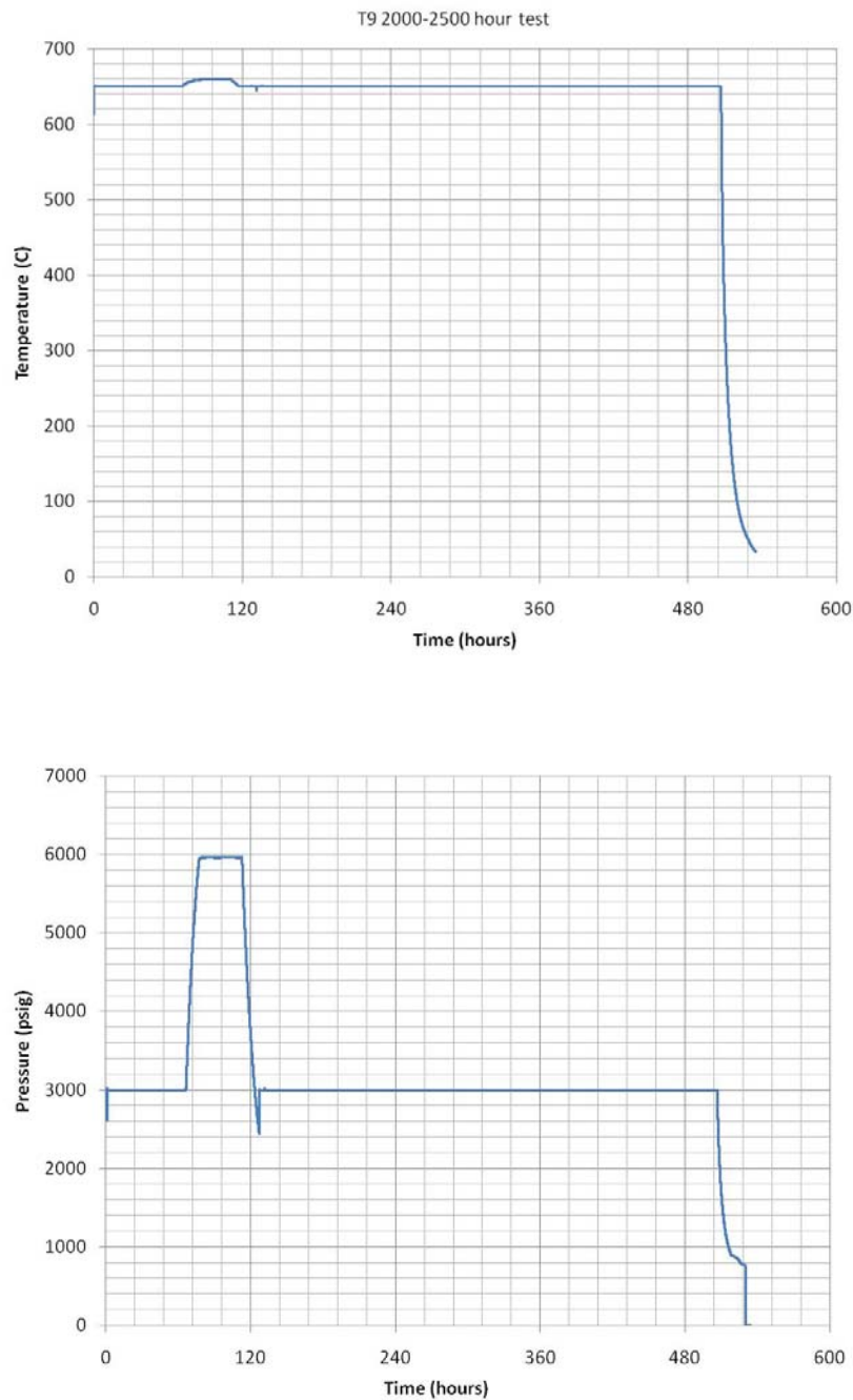
Figure 23 Temperature and pressure history for the 2000-2500 hour test duration
