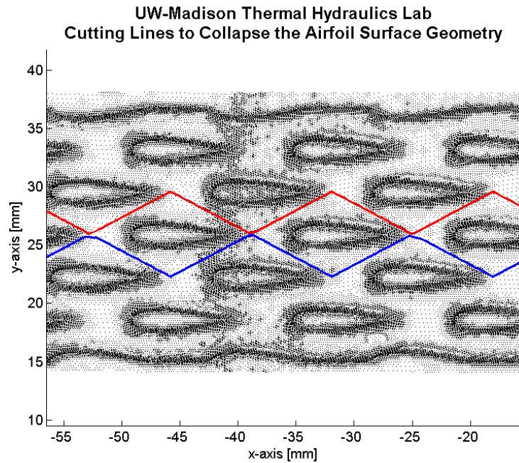
Figure 120: A XY view of the trimmed point cloud data from the 8.1 mm NACA0020 surface scan with cutting lines for the center row of airfoils (red and blue) used to collapse the point cloud into a unit cell overlaid.
