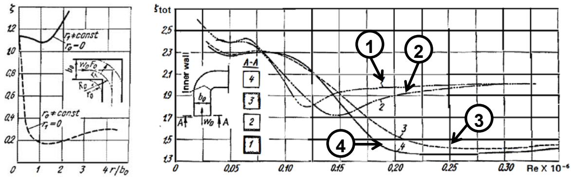
Figure 92: (left) A plot indicating the asymmetric importance of interior corner roundness relative to exterior corner roundness, where the solid line shows the loss coefficient for a 90-degree bend with a sharp interior corner as the roundness of the exterior corner is increased as scaled by the channel width, and the dashed line shows the opposite where the interior corner is rounded and the exterior corner is kept sharp; (right) A plot indicating the importance of interior corner roughness relative to roughness throughout the curved section, where the total loss across a bend is shown as a function of the Reynolds number of the flow. Line 1 shows a bend with roughness on the entire interior, while line 2 shows a bend with the same roughness applied only to the interior corner, line 3 shows a bend with a smooth interior wall and a rough wall elsewhere, and line 4 shows a bend with all smooth walls. Both from Idel'chik [16].
