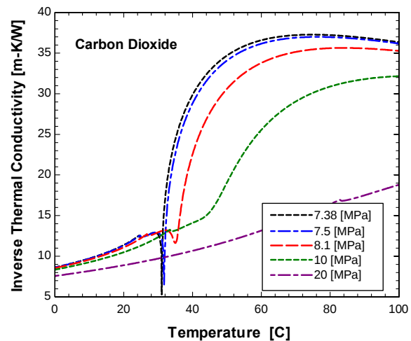
Figure 56: A plot of the inverse of thermal conductivity versus temperature of carbon dioxide with several isobars shown. The pseudo-critical line is left off for clarity.
