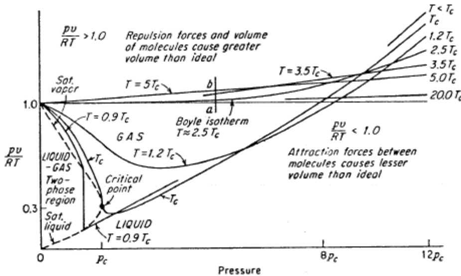
Figure 51: A diagram of compressibility versus pressure for a generic pure fluid with the saturation curve and several isotherms shown (REPLACE WITH CLEANER VERSION AND CITE?).
