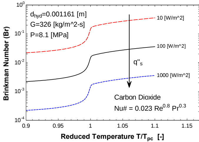
Figure 58: The variation in the Brinkman number vs. temperature at several heat fluxes.
