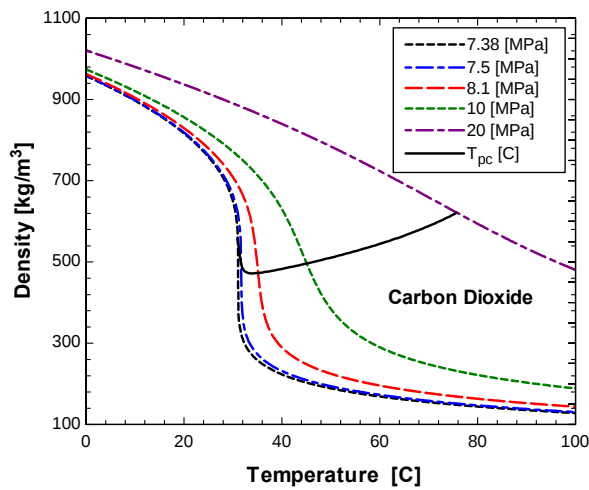
Figure 53: A plot of the temperature versus density of carbon dioxide with several isobars and the pseudo-critical line shown.
