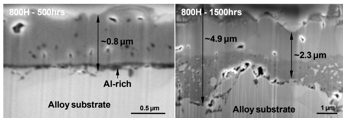
Figure 38: Secondary electron images of the cross-sectional alloy 800H samples exposed to the s- \text{Co}_2 at 650C for 500 and 1500 hours
