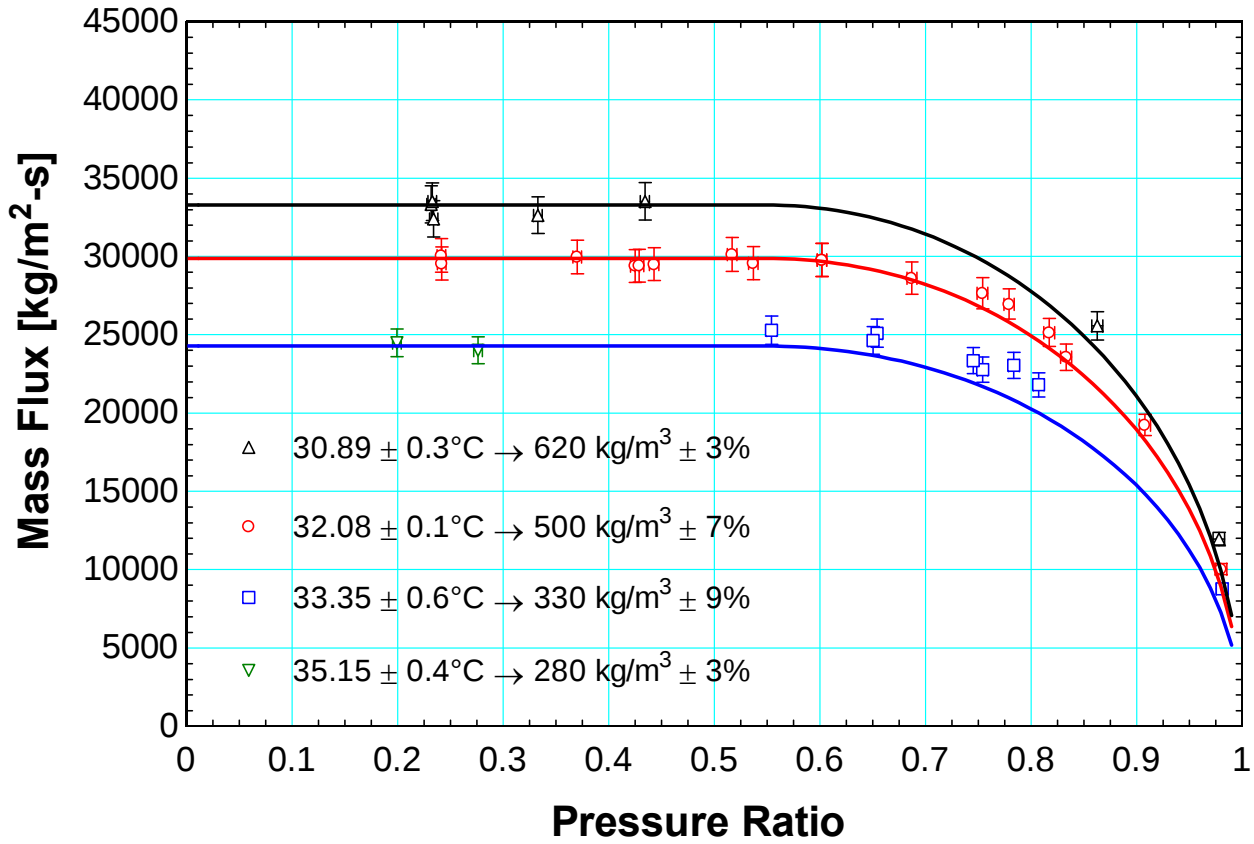
Figure 248 Mass flux versus pressure ratio for measurements taken at P_{inlet}=7.58 MPa and different inlet densities. Discharge coefficient of 0.75 fit to data.
