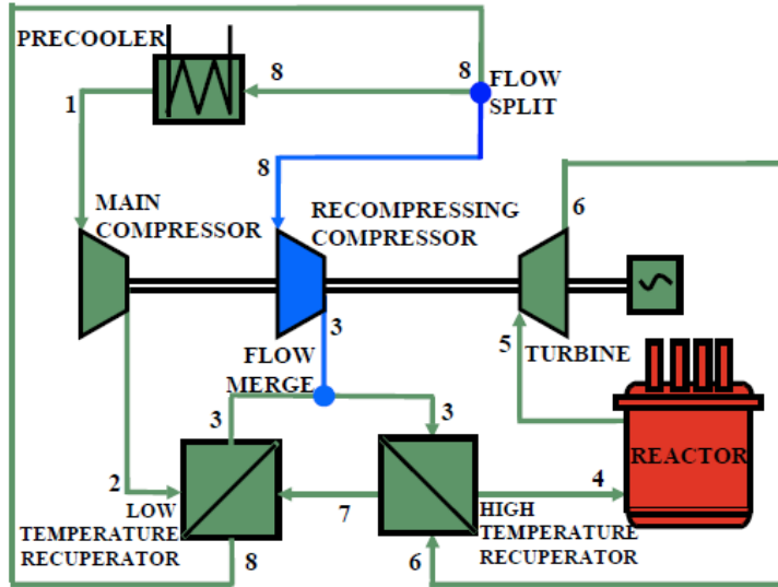
Figure 47: A diagram of the recompression supercritical carbon dioxide Brayton cycle, from Dostal [4].
