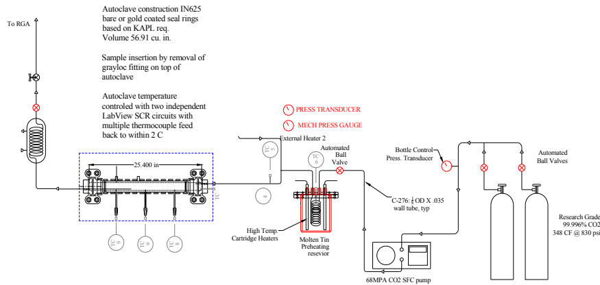
Figure 2 Supercritical carbon dioxide corrosion system diagram
