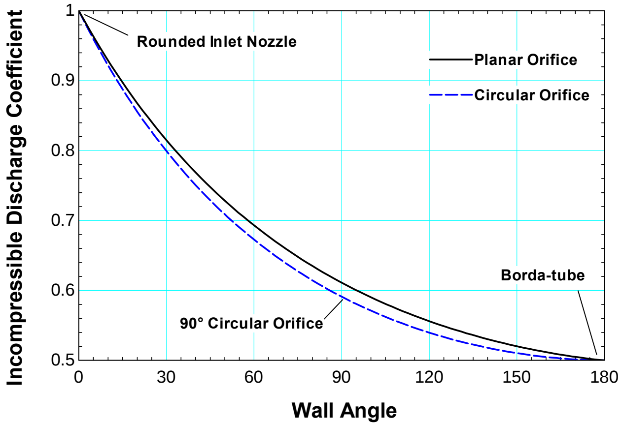
Figure 167 Discharge coefficient for PR=1 as a function of wall angle \alpha for planar flow and axisymmetric flow, k=1.4
