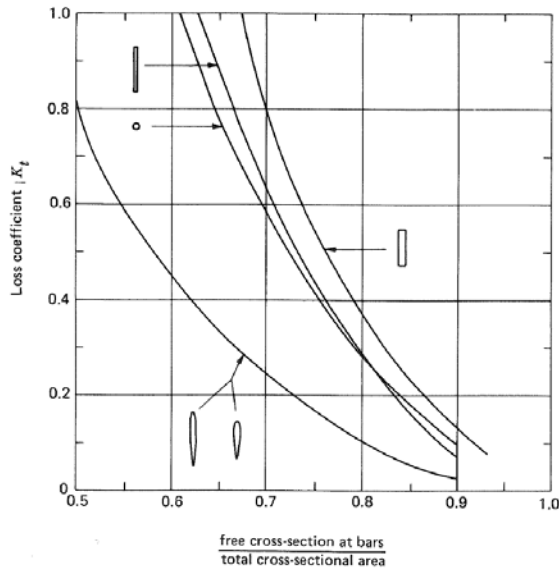
Figure 96: Loss coefficients for a single trashrack plane consisting of bars of various cross section from Miller [12], assumed at sum large Reynolds number consistant with findings of the Reynolds number dependence of pipe bend loss coefficients described by Miller.
