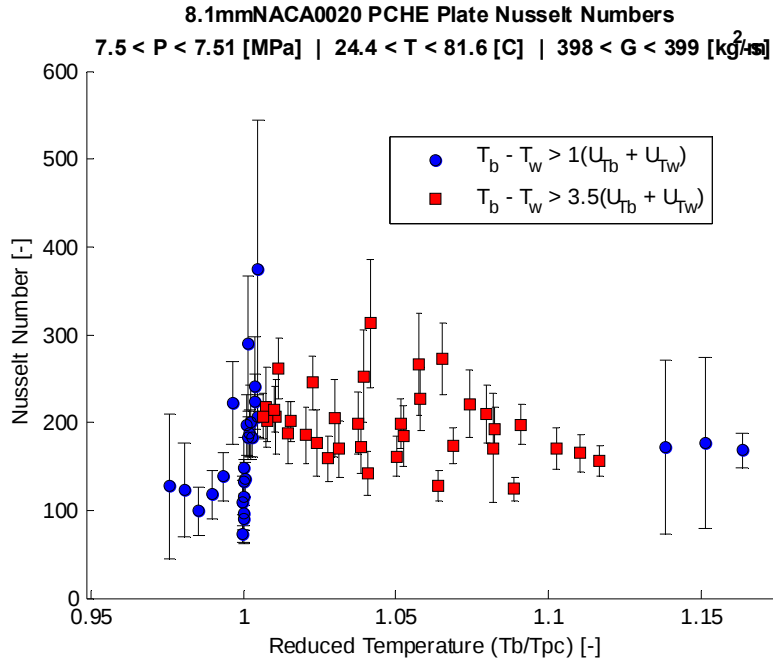
Figure 145: 8.1 mm NACA0020 airfoil fin channel Nusselt number vs. reduced temperature at 7.5 MPa and low mass flux for cooling-mode flow using the measured geometry with error bars indicating propagated uncertainty.
