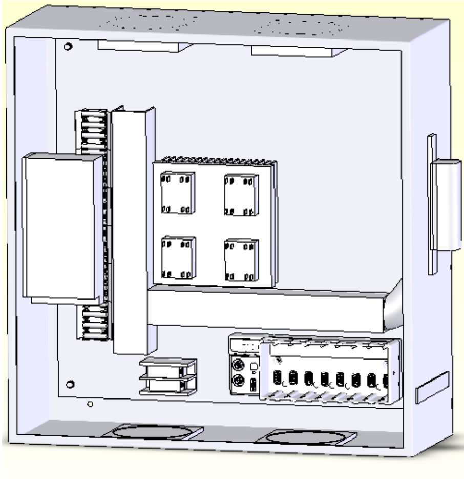
Figure 203 Layout of safety and instrumentation panel box
