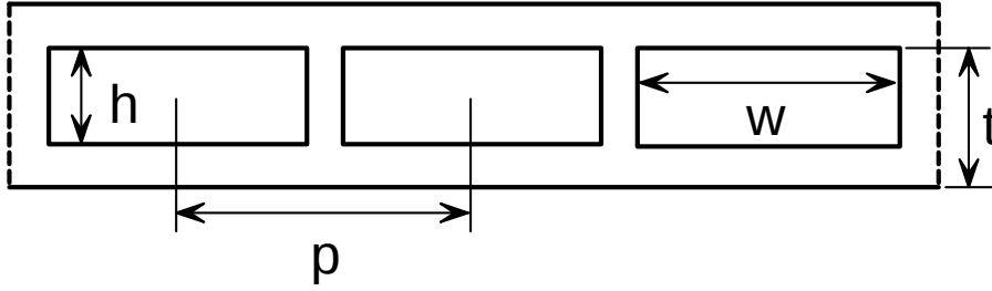
Figure 85: A diagram of a section of a PCHE stack-up where channel cross-sections are idealized by their circumscribing rectangles, where h is the channel height, w is the channel width, p is the lateral channel pitch, and t is the plate thickness.
