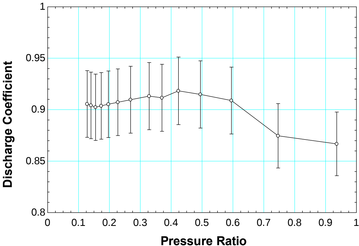
Figure 238 Manufacturer’s Flow Coefficient Data in terms of Discharge Coefficient
