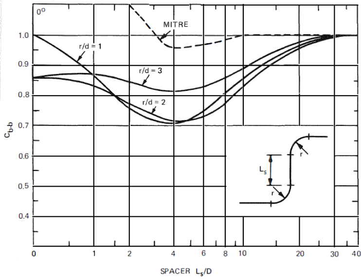
Figure 94: A plot by Miller of the bend-bend interaction coefficient for two in-plane 90-degree bends of various radius ratios and separation lengths; from Miller [12].
