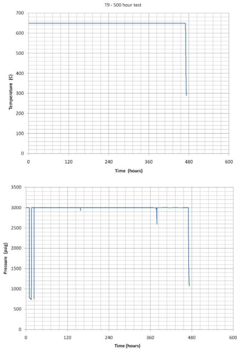
Figure 19 Temperature and pressure history for the first 500 hour test duration
