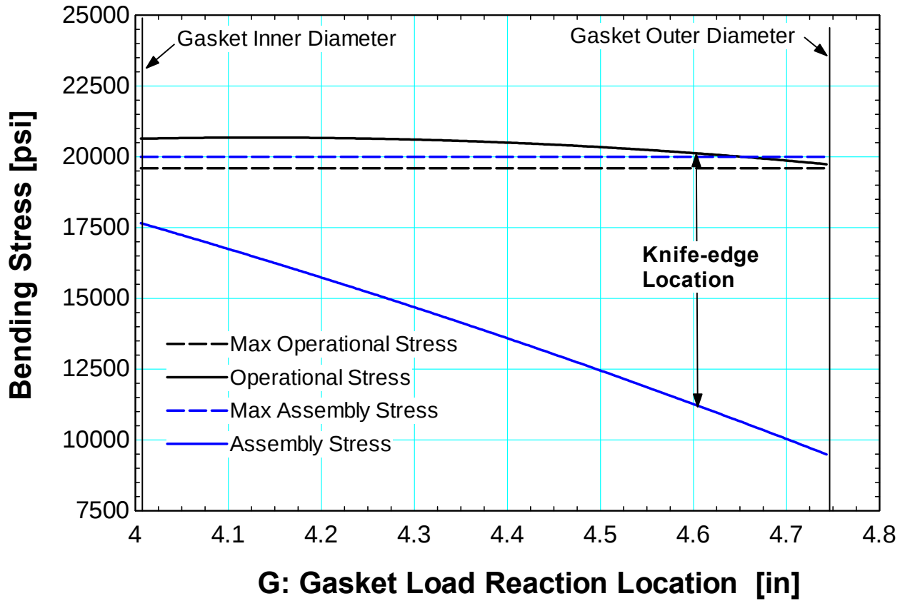
Figure 227 Assembly and operational stress as a function of gasket load reaction for the parameters listed in Table 4-19.
