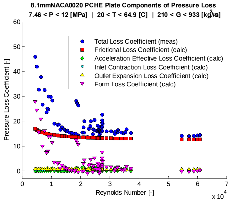
Figure 143: 8.1 mm NACA0020 airfoil fin channel calculated pressure loss components using the measured geometry. Note that calculated acceleration, inlet contraction, and outlet expansion points are approximately the same and overlap.
