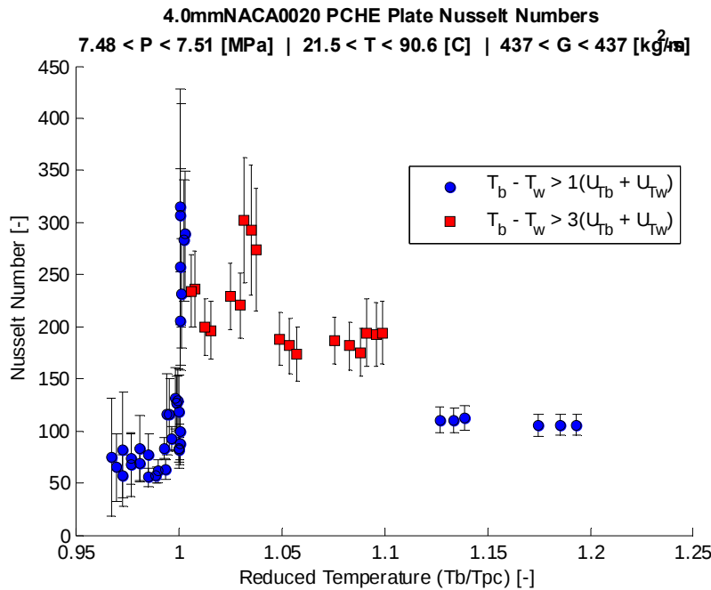
Figure 146: 4.0 mm NACA0020 airfoil fin channel Nusselt number vs. reduced temperature at 7.5 MPa and low mass flux for cooling-mode flow using the measured geometry with error bars indicating propagated uncertainty.
