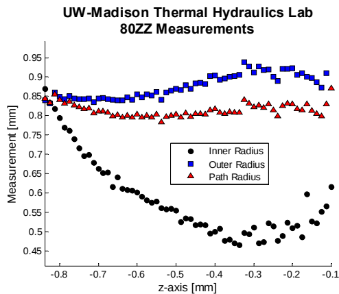
Figure 112: Measured inner and outer corner radii, as well as the central path line radii versus depth for the 80-degree zig-zag surface.
