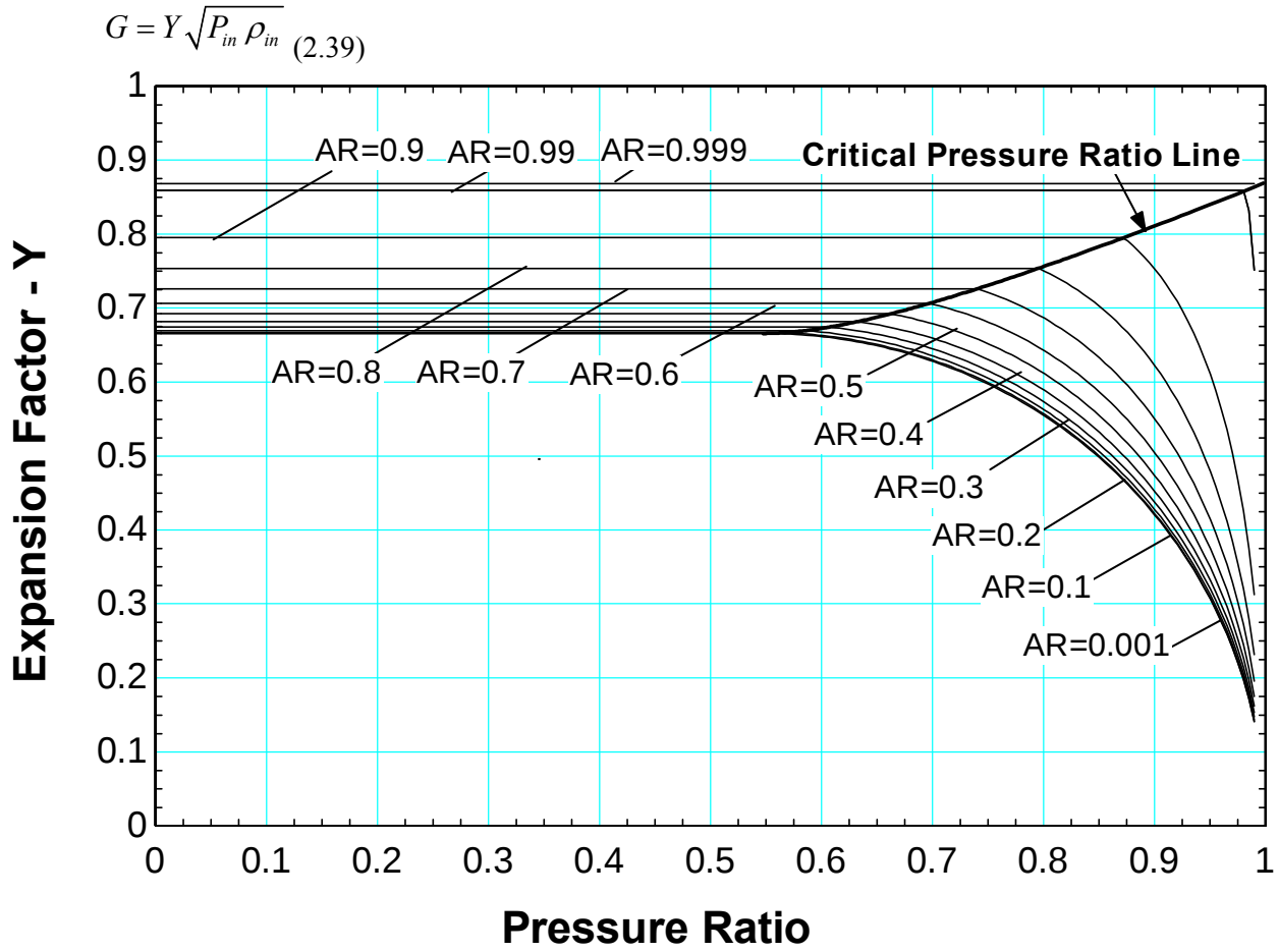
Figure 161 Expansion factor Y as a function of pressure ratio for various aspect ratios; also shown is the calculated critical pressure ratio line as defined by equation (2.33); The specific heat ratio was taken to be k=1.292 , corresponding to carbon dioxide at 300 K and ideal gas conditions.
