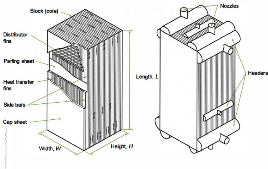
Figure 63: A diagram of a PFHE as well as typical header and nozzle attachments from the ALPEMA Standards [35].
