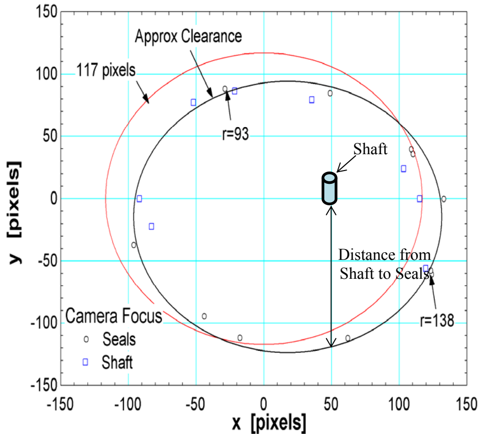
Figure 199 Results obtained from pixel counting program detailing the pixel distance from the center shaft to the seal.
