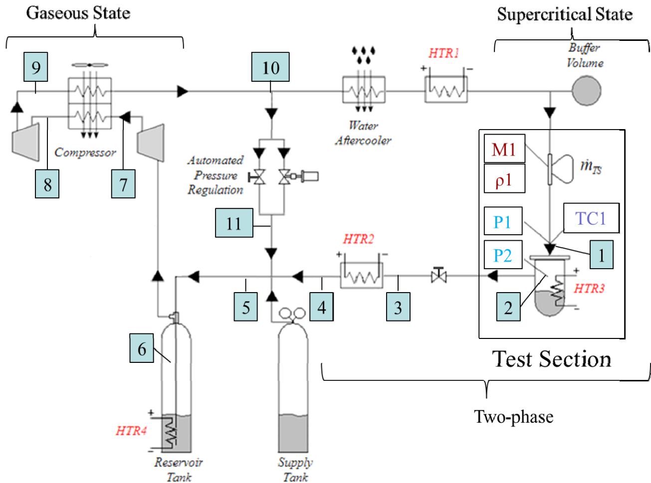
Figure 174 Schematic of UW compression loop facility
