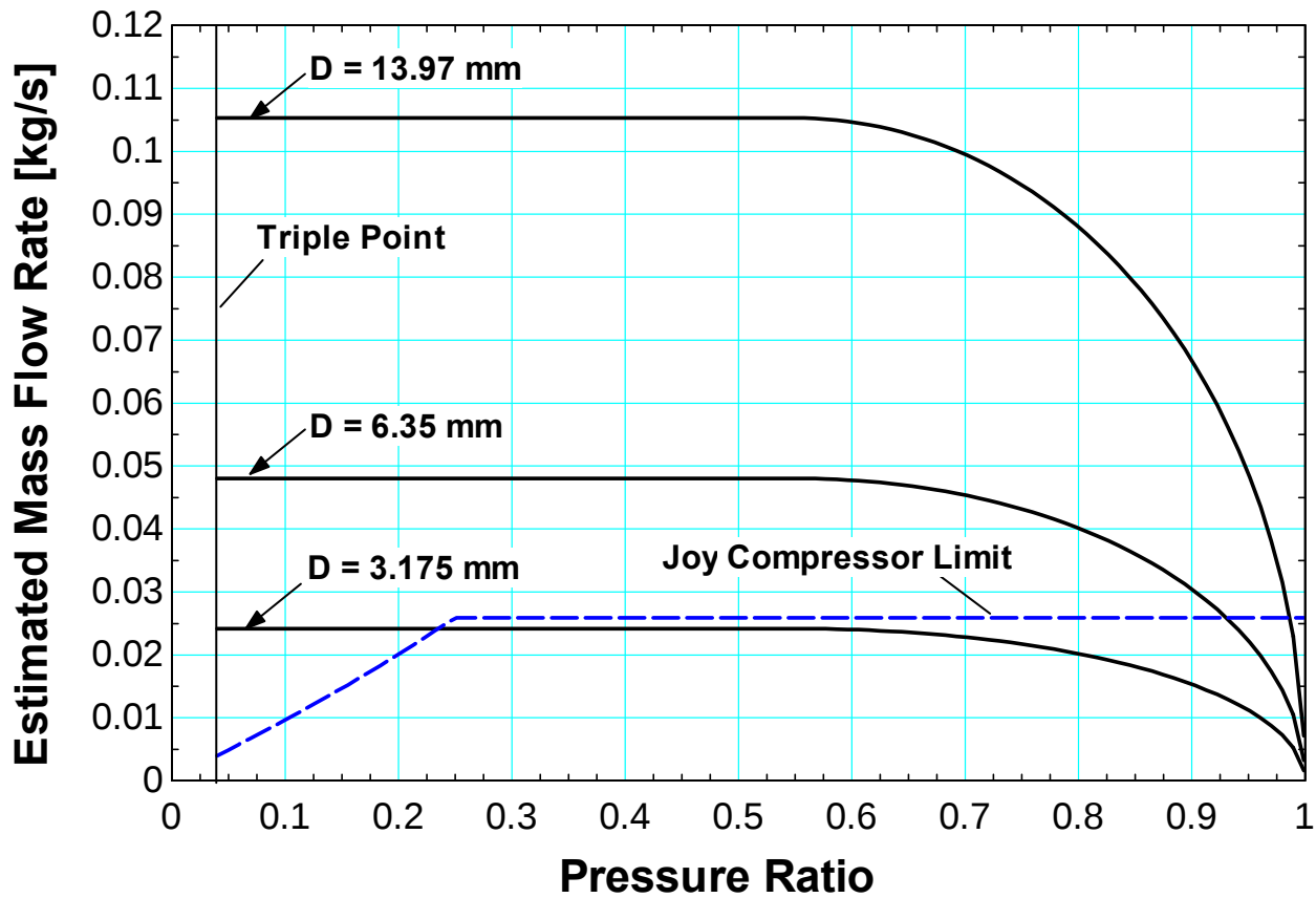
Figure 178 Estimate of mass flow rate for several different journal diameters at an inlet pressure of 13.8 MPa and temperature of 325 K. Compressor limit based on equation (3.34) through (3.40)
