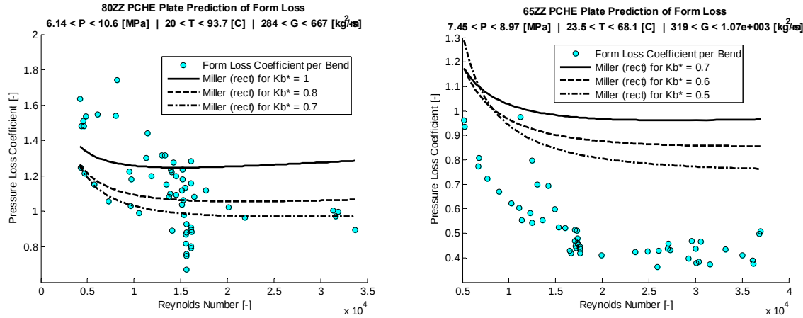
Figure 134: A comparison of Miller's correlations for zig-zag pipe channels vs. the calculated form loss coefficient per bend for the 80-degree zig-zag channel and the 65-degree zig-zag channel using measured geometry.
