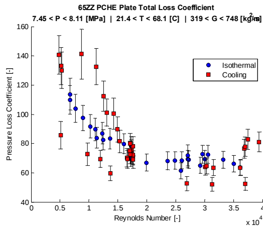
Figure 131: A plot of the 65-degree zig-zag channel isothermal and cooling-mode pressure loss coefficient using the design and measured geometry respectively with error bars indicating propagated uncertainty.
