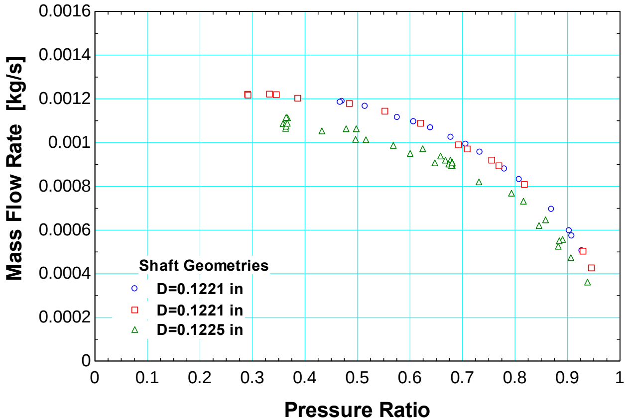
Figure 241 Raw data of measurements obtained with test facility at P_{inlet} = 2.065 MPa and \rho_{inlet} = 24 kg/m^3 . Offset in mass flow rate clearly apparent for 10 \mu m difference in shaft diameter.
