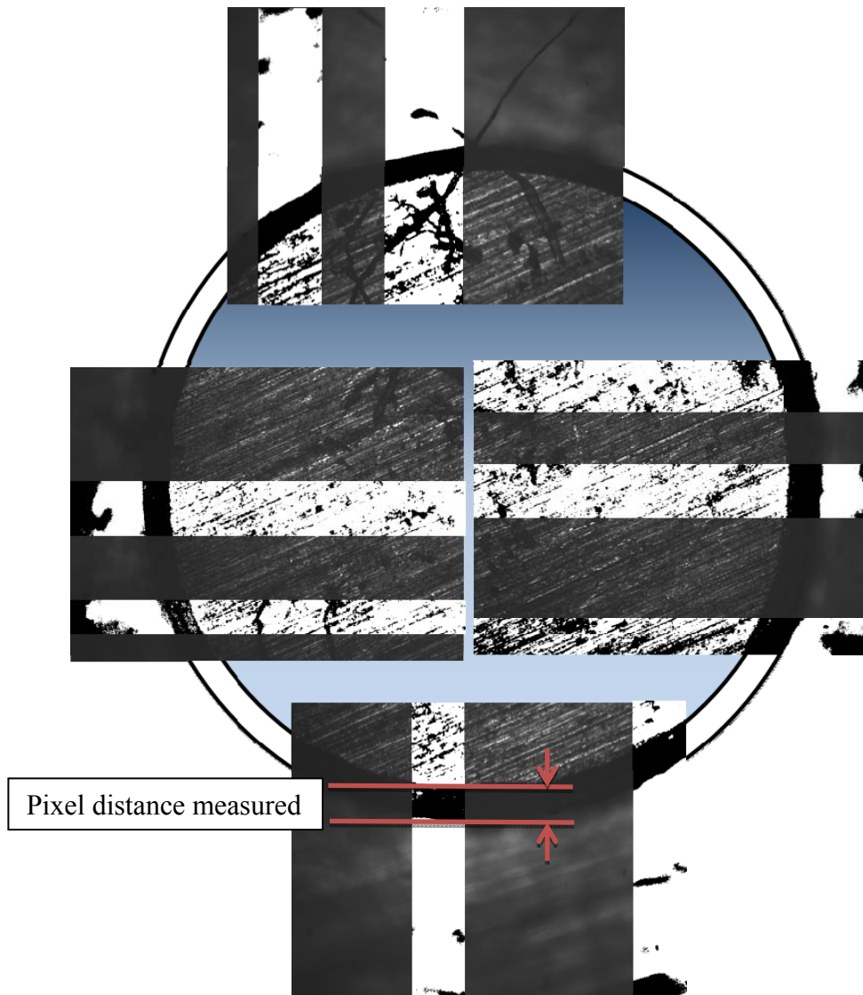
Figure 198 MATLAB filtered images placed over raw images of assembled shaft-seal interface
