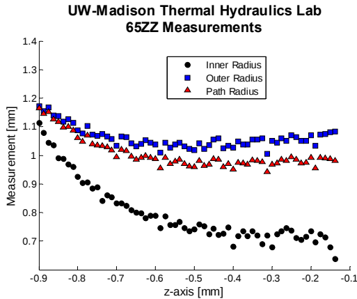
Figure 116: Measured inner and outer corner radii, as well as the central path
