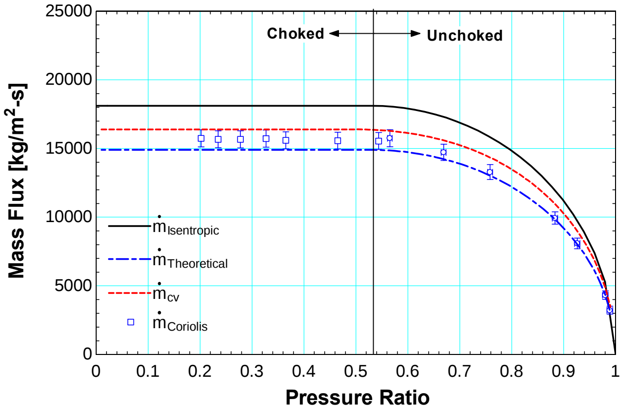
Figure 235 Measurements obtained with a knife-edge orifice at P_{inlet} = 7.67 \text{ MPa} and \rho_{inlet} = 92 \text{ kg/m}^3 . Discharge coefficient evaluated at C_d = 0.84 for the data shown.
