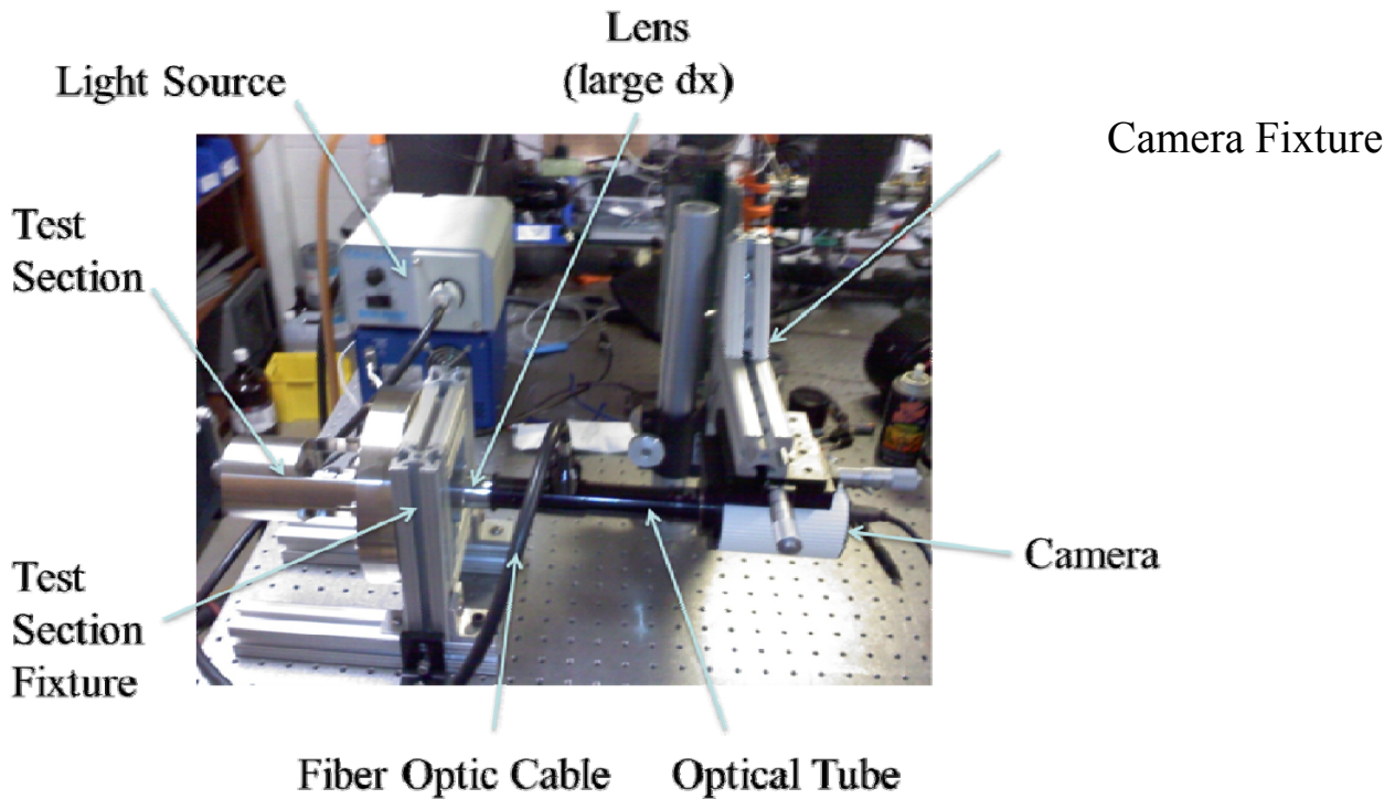
Figure 194 Optical setup used to verify the expected eccentricity
