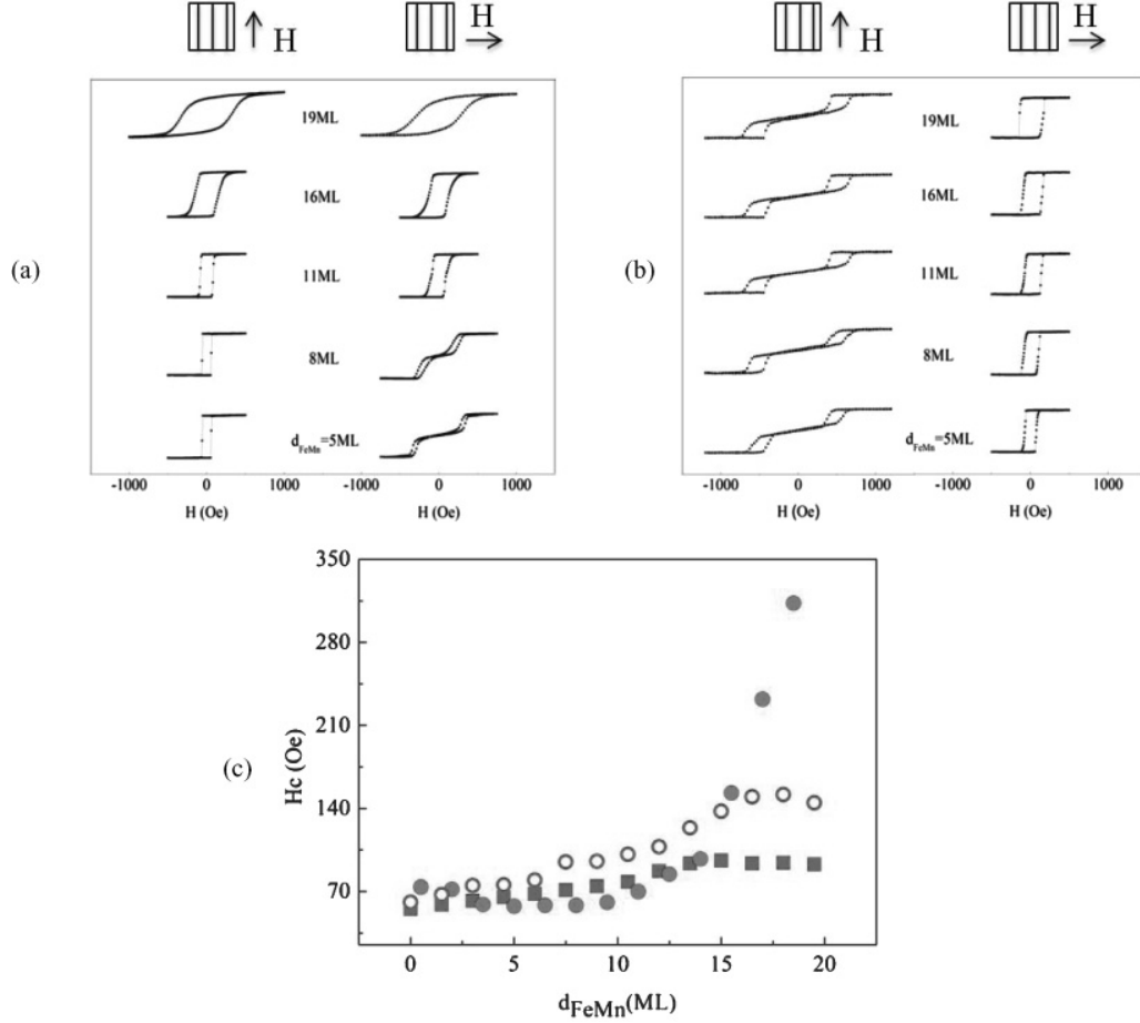
FIG. 2. (Color online) (a) MOKE hysteresis loops of FeMn/Fe(2ML)/Co/Cu(1,1,10) at room temperature. (b) MOKE hysteresis loops of FeMn/Fe(8ML)/Co/Cu(1,1,10) at T = 90 K. (c) Coercivity of the easy axis loops for d_{\text{Fe}} = 2 ML sample at room temperature (red solid dots), d_{\text{Fe}} = 8 ML sample at room temperature (blue squares), and d_{\text{Fe}} = 8 ML sample at T = 90 K (blue open circles).
