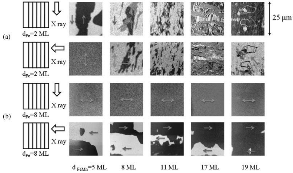
FIG. 4. (Color online) XMCD-PEEM images ( 25 \mu\text{m} \times 25 \mu\text{m} ) of FeMn/Fe/Co/Cu(1,1,10). The characteristic domain evolution in the FM phase fcc Fe ( d_{\text{Fe}} = 2 \text{ ML} ) sample no longer exists in the AFM phase fcc Fe ( d_{\text{Fe}} = 8 \text{ ML} ) sample. Each pair of images is taken at the same position of the sample.
