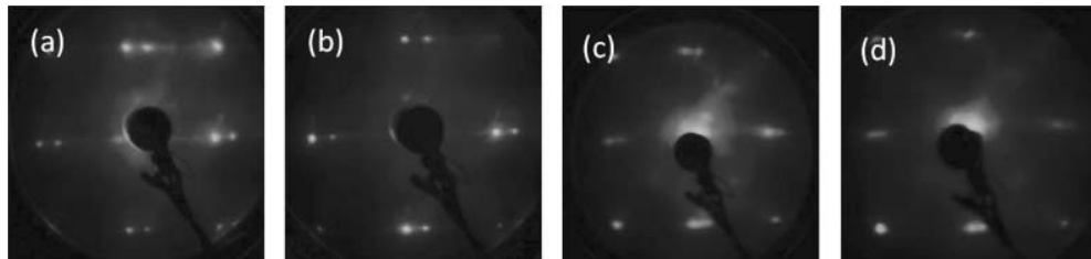
FIG. 1. (Color online) LEED patterns taken at \sim 123 \text{ eV} at each stage of the FeMn(10ML)/Fe(2ML)/Co(20ML)/Cu(1,1,10) sample growth. (a) Cu(1,1,10) substrate, (b) after 20 ML Co growth, (c) after 2 ML Fe growth, and (d) after 10 ML FeMn growth.
