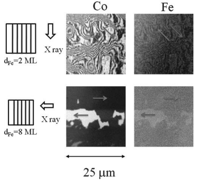
FIG. 3. (Color online) XMCD-PEEM images ( 25 \mu\text{m} \times 25 \mu\text{m} ) of FeMn/Fe/Co/Cu(1,1,10). The same domain pattern for Co and Fe shows that the FM fcc Fe at 2 ML and the induced FM Fe in the AFM fcc Fe at 8 ML are coupled ferromagnetically to the Co moment.
