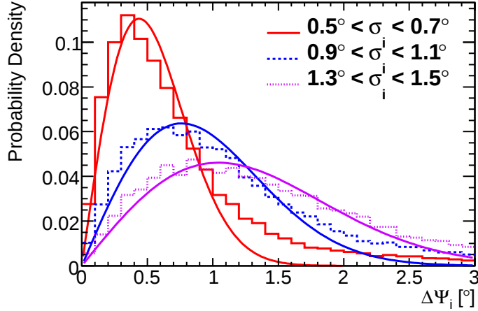
Fig. 9.— Angular deviation between neutrino and reconstructed muon direction \Delta\Psi for ranges in \sigma_i , the reconstructed angular uncertainty estimator. Fits of these distributions to 2-dimensional Gaussians projected into \Delta\Psi are also shown. The value of \sigma_i is correlated to the track reconstruction error. A small fraction of events are not well-represented by the Gaussian distribution, but these are the least well-reconstructed events and contribute the least to signal detection.
