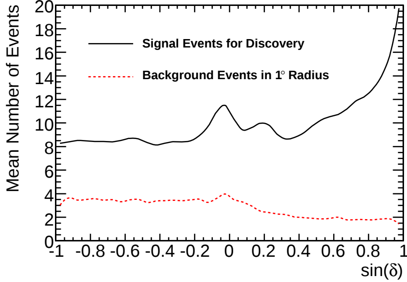
Fig. 20.— Mean number of E^{-2} \nu_\mu + \bar{\nu}_\mu signal events at the final cut level required for a discovery at 5\sigma in 50% of trials and the mean number of background events in a circular bin with a radius of 1^\circ versus sine of the declination.
