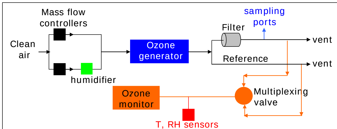
Figure 1-S: Experimental setup
