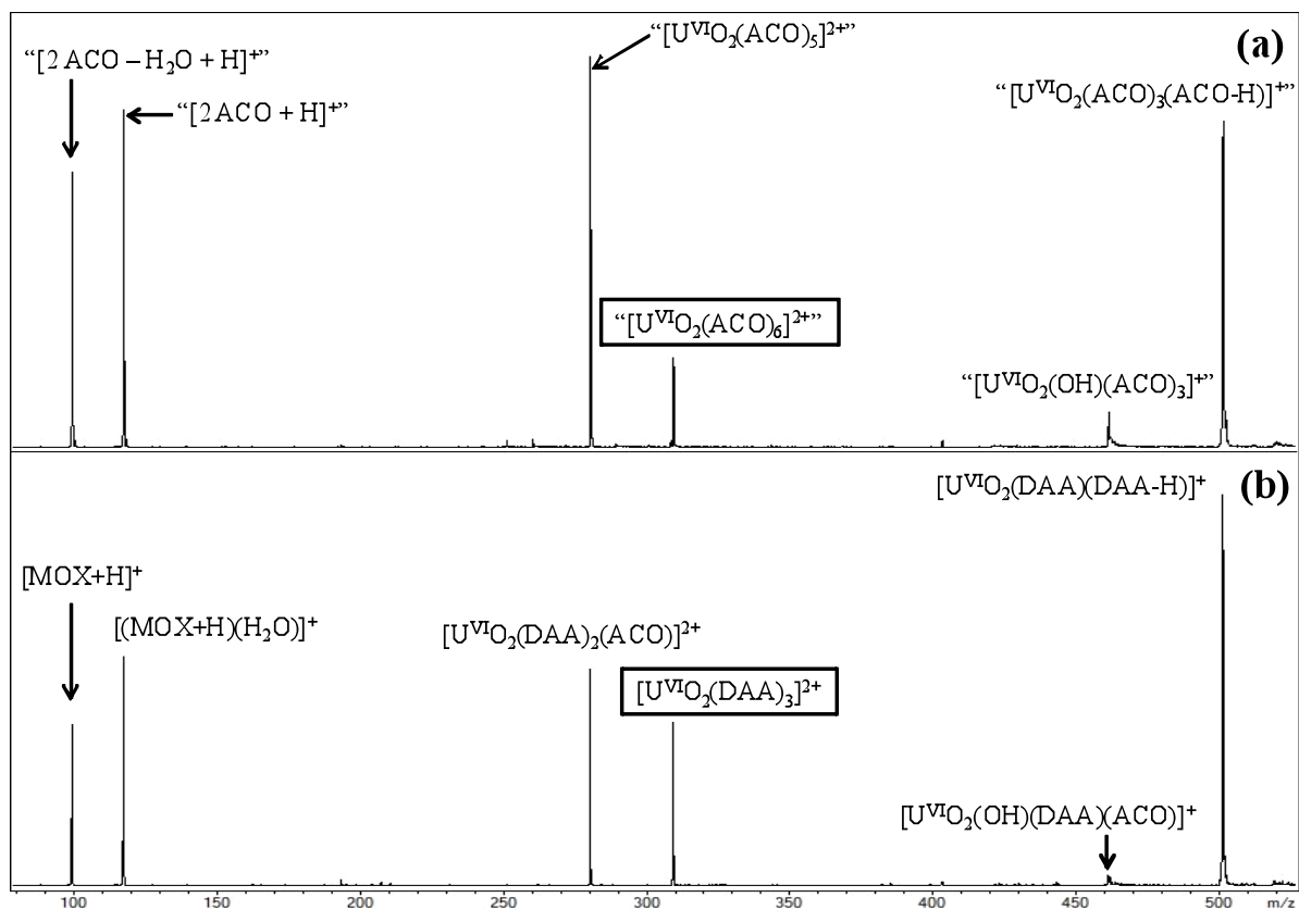
Figure 3. CID product spectra for precursor ions (identified in boxes) with a nominal equatorial coordination number of 6. Spectrum (a) is for the species with m/z = 309 , which corresponds to [\text{UO}_2(\text{ACO})_6]^{2+} , produced from nominally “pure acetone”. Spectrum (b) is for the species with the same atomic composition as (a), but with the known ligand composition [\text{UO}_2(\text{DAA})_3]^{2+} .
