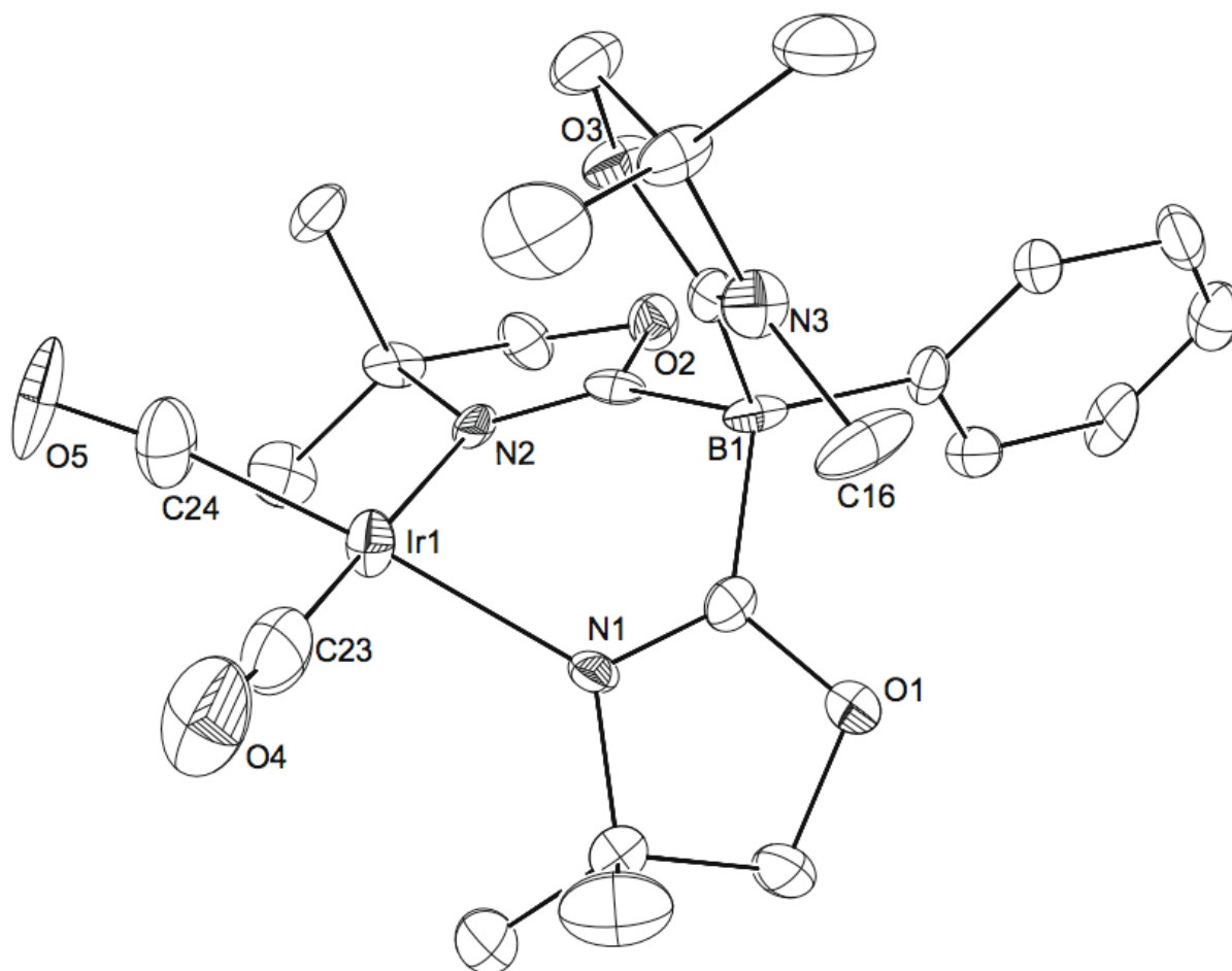
Figure 5. ORTEP diagram of [\text{Ir}(\kappa^2\text{-To}^{\text{M}}\text{-Me})(\text{CO})_2][\text{OTf}] ( 5 ). Centroids are drawn at 50% probability. Hydrogen atoms, the \text{OTf}^- counterion, and a co-crystallized benzene molecule are hidden for clarity. Distances (given in Å): Ir1-N1, 2.090(8); Ir1-N2, 2.074(8); Ir1-C23, 1.82(2); Ir1-C24, 1.87(1); C23-O4, 1.17(2); C24-O5, 1.12(1); N3-C16, 1.46(1). Angles given in °: C23-Ir1-C24, 87.1(5); N1-Ir1-N2, 85.9(3); N1-Ir1-C23, 93.2(4); N2-Ir1-C24 94.0(4).
