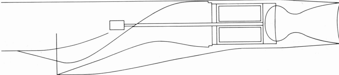
Fig. 5.6 - Ramjet power-plant configuration, bottom inlet
