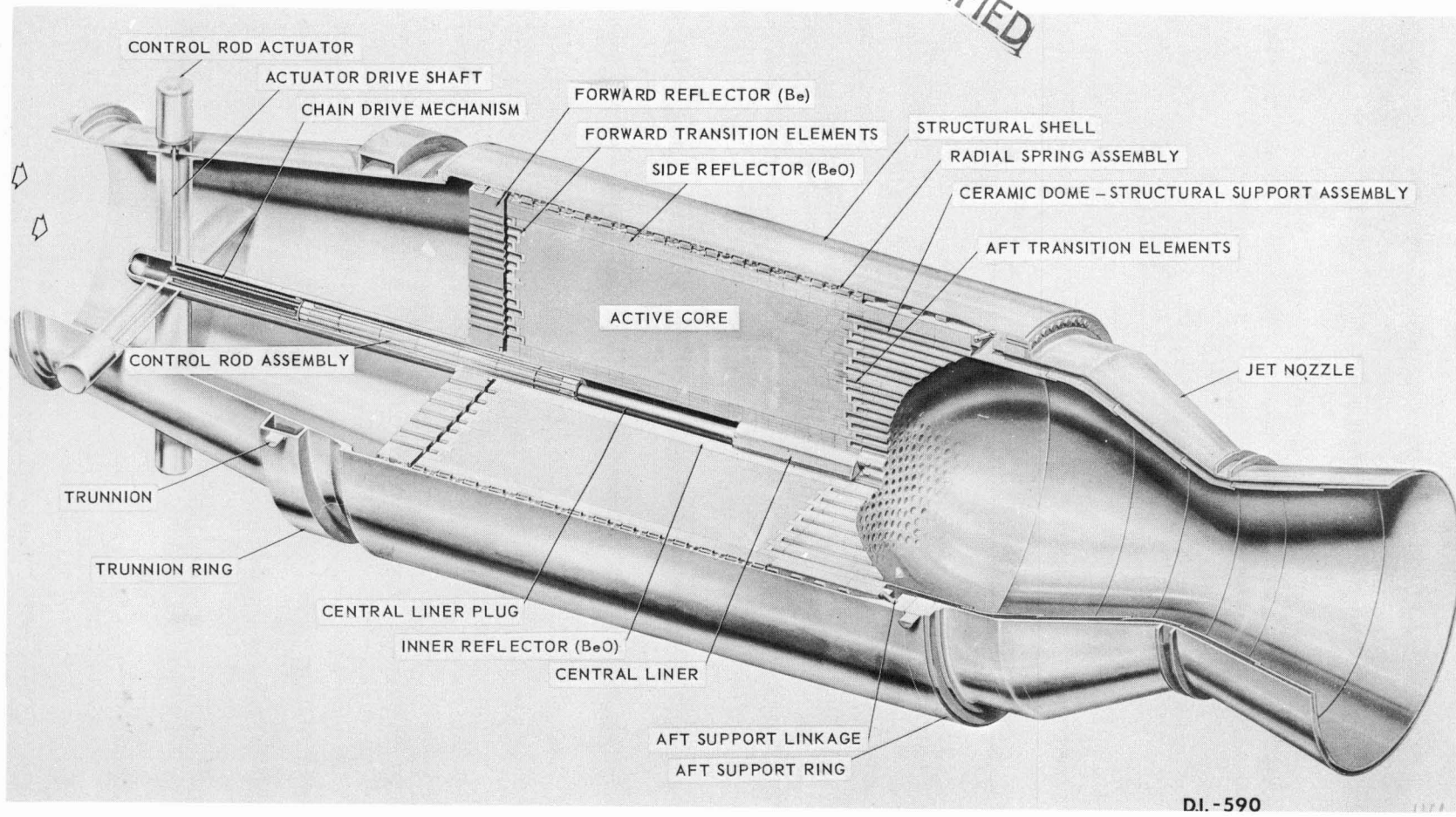
Fig. 5.5 - Nuclear ramjet reactor
