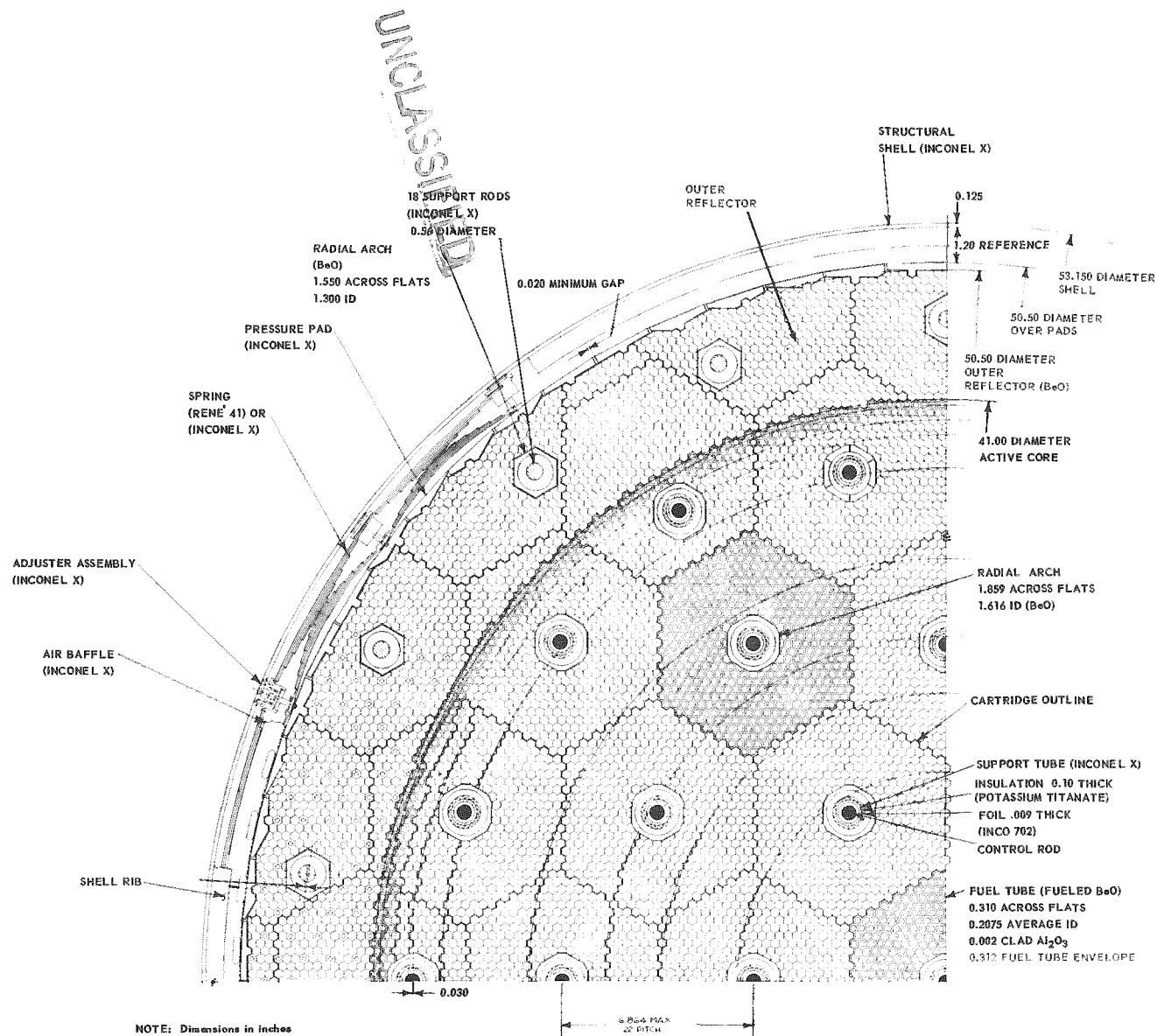
Fig. 3.21—D141A-1 reactor for the proposed CCT
