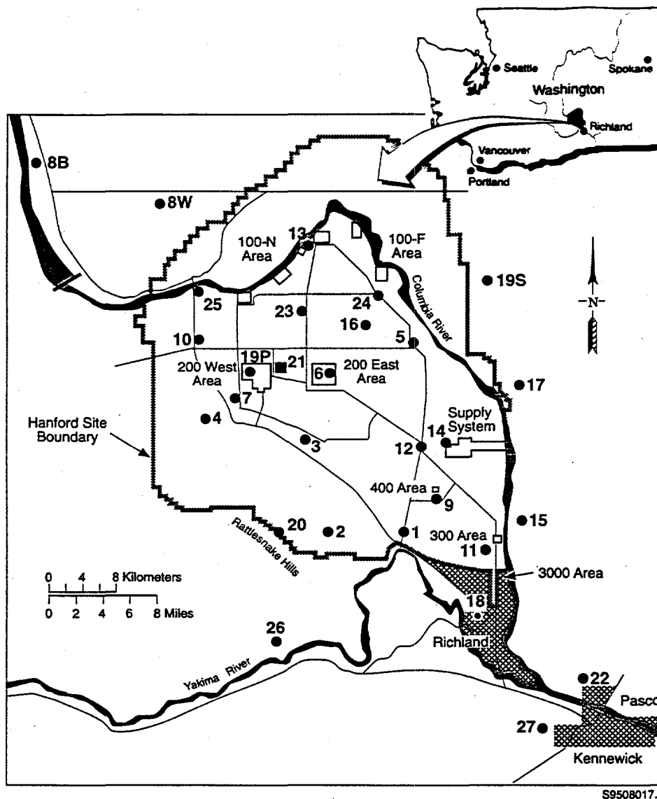
Figure 4.1-1. Hanford Meteorological Monitoring Network.
