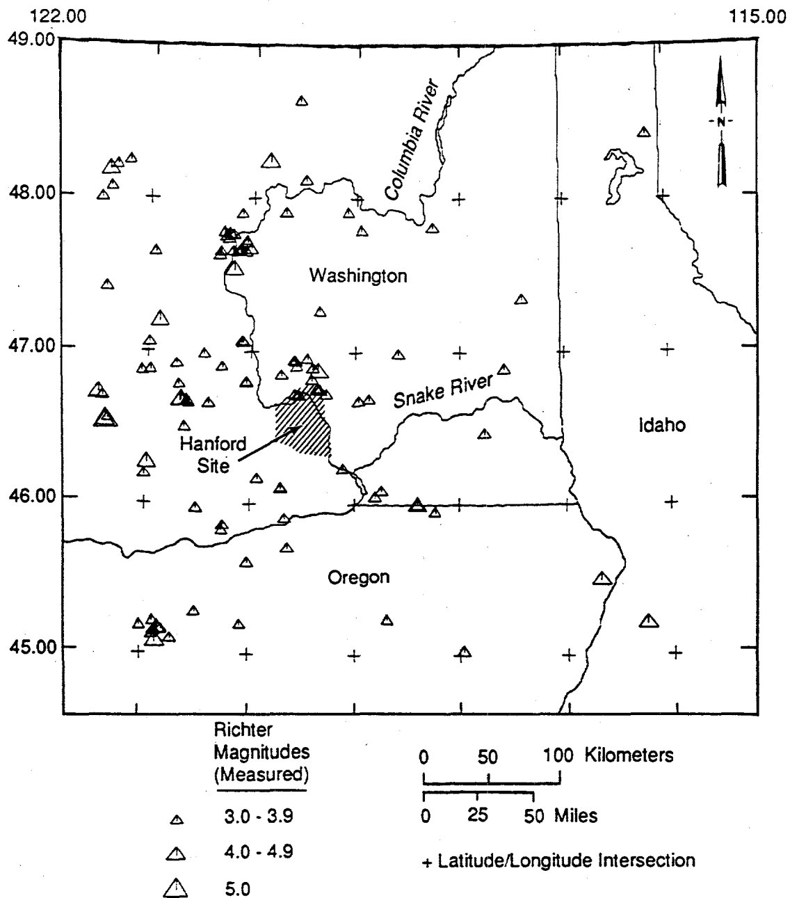
Figure 4.2-9. Seismicity of the Columbia Plateau and surrounding areas as measured by seismographs. All earthquakes between 1969 and 1989 with magnitude 3 or larger are shown (Rohay 1989).
