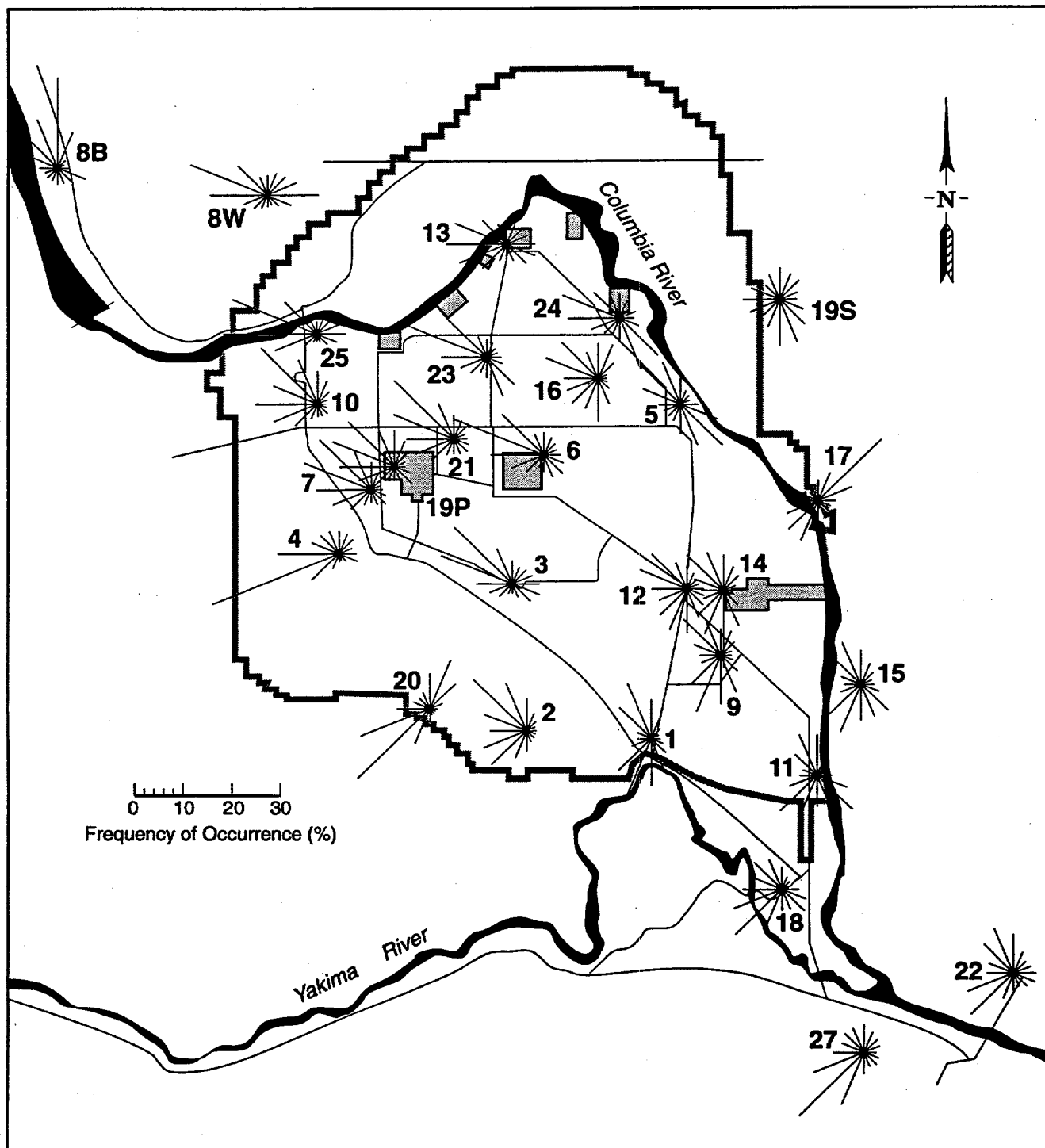
Figure 4.1-2. Wind roses (at 10 m) for the Hanford Meteorological Monitoring Network, 1979 to 1994. The point of each rose represents the direction from which the winds come.
