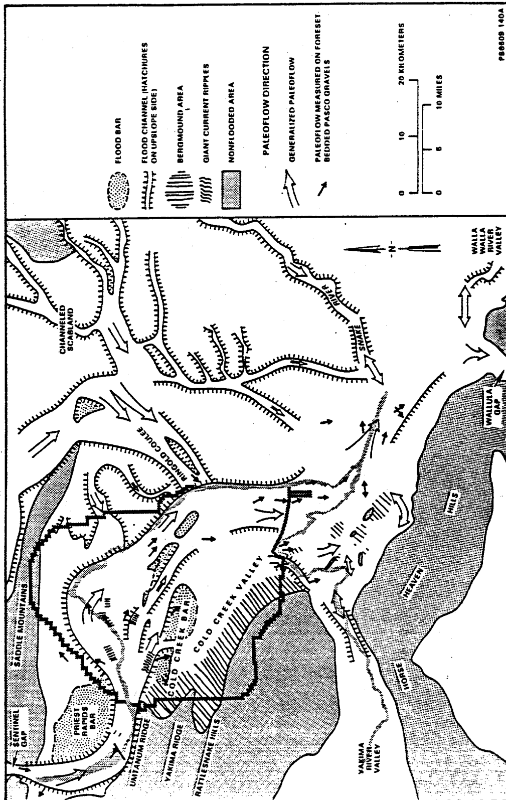
Figure 4.2-2. Paleoflow directions and landforms associated with cataclysmic flooding in the Central Columbia Plateau (after DOE 1988).
