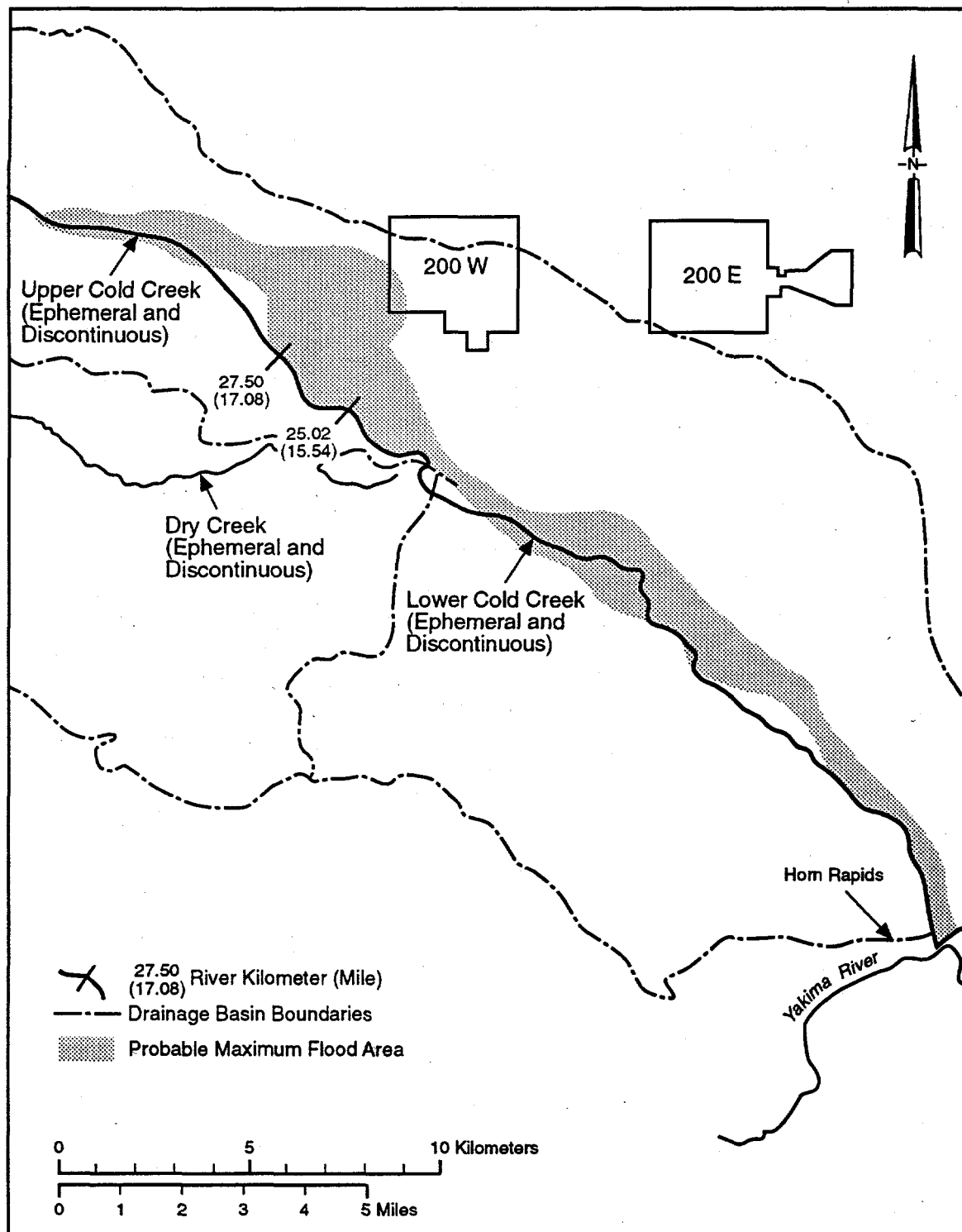
Figure 4.3-6. Extent of probable maximum flood in Cold Creek Area (after Skaggs and Walters 1981).
