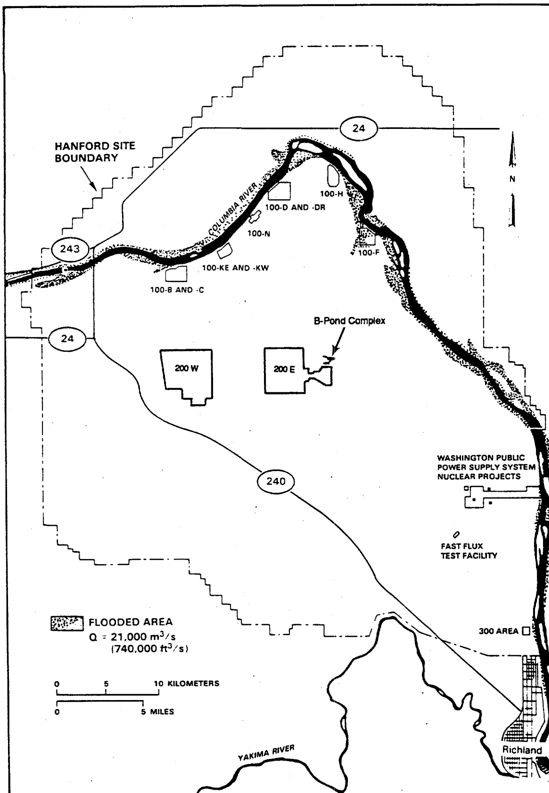
Figure 4.3-2. Flood area during the 1894 flood (DOE 1986).
