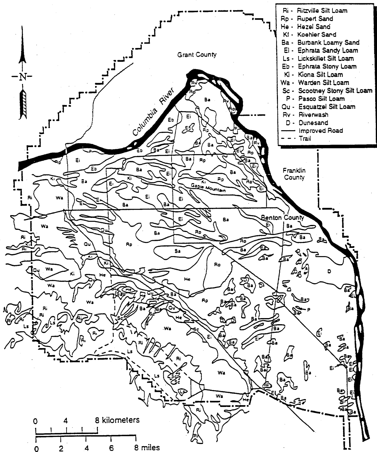
Figure 4.2-7. Soil map of the Hanford Site (from Hajek 1966).
