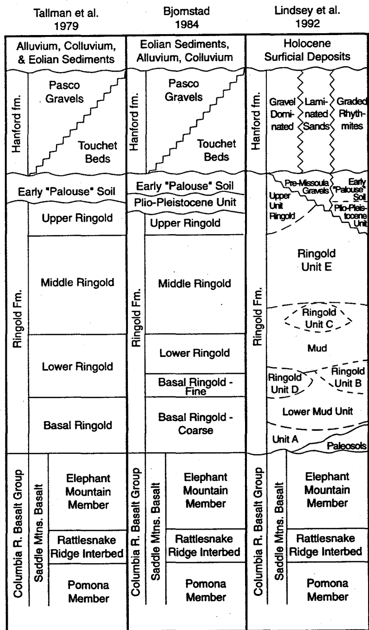
Figure 4.2-4. Stratigraphic column for the Hanford Site showing correlations among various authors.
