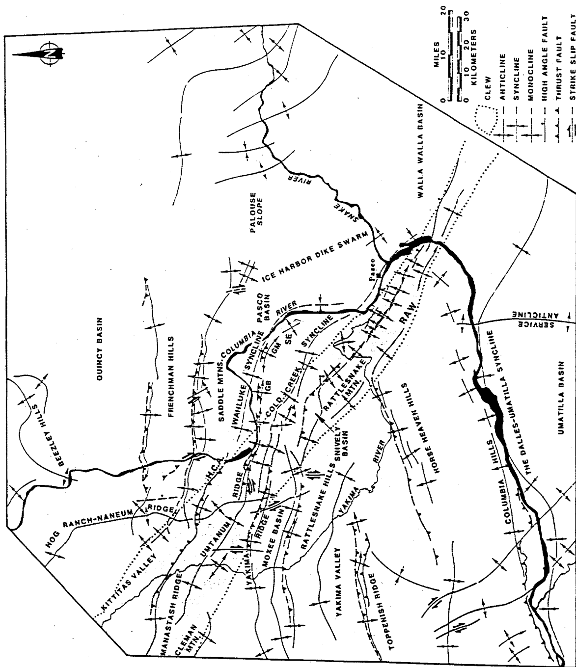
Figure 4.2-6. Location of structural features (Reidel et al. 1989)
