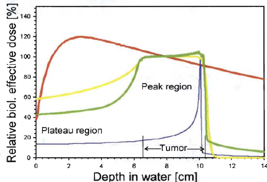
FIGURE 4. Biologically effective dose, as a function of the penetration depth in water, for MeV photon beams (15 MeV, red line), mono-energetic carbon ions (220 MeV/u, blue line) and spread-out Bragg peaks of protons (120 MeV; yellow line) and carbon ions (220 MeV/u; green line). The given numbers are relative units, normalized to dose at 8cm depth. For protons a constant RBE of 1.1 is assumed. The RBE for carbon was calculated using the track structure model (reproduced from [7]).
