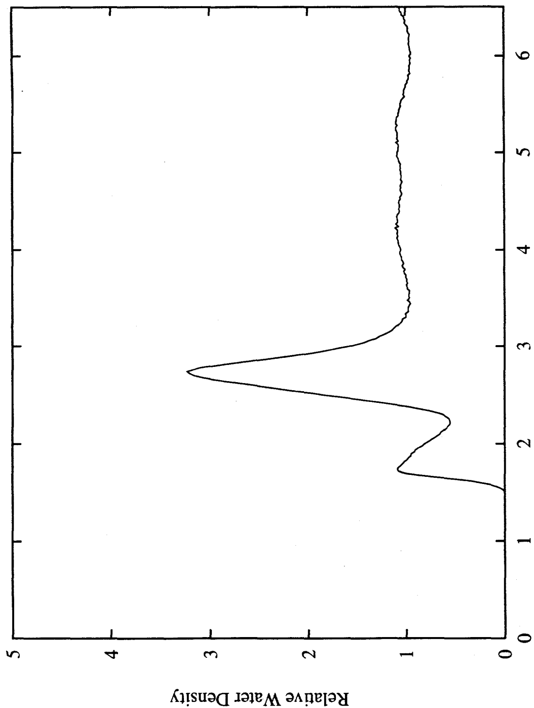
Distance Between Oxygen Atoms in Water and Nearest Protein Atoms (Å)
