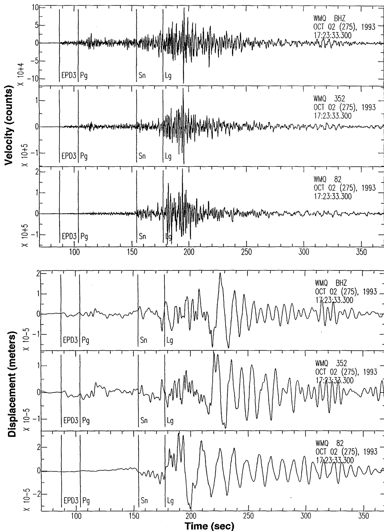
Figure 2. Seismograms for and earthquake 633 km from WMQ. The top traces are raw broadband velocity and the bottom traces are instrument corrected displacement low pass filtered at 0.2 Hz. In both plots the horizontal components are rotated to radial and tangential directions. The displacement shows the dispersed surface wave energy, not visible in the velocity version.
