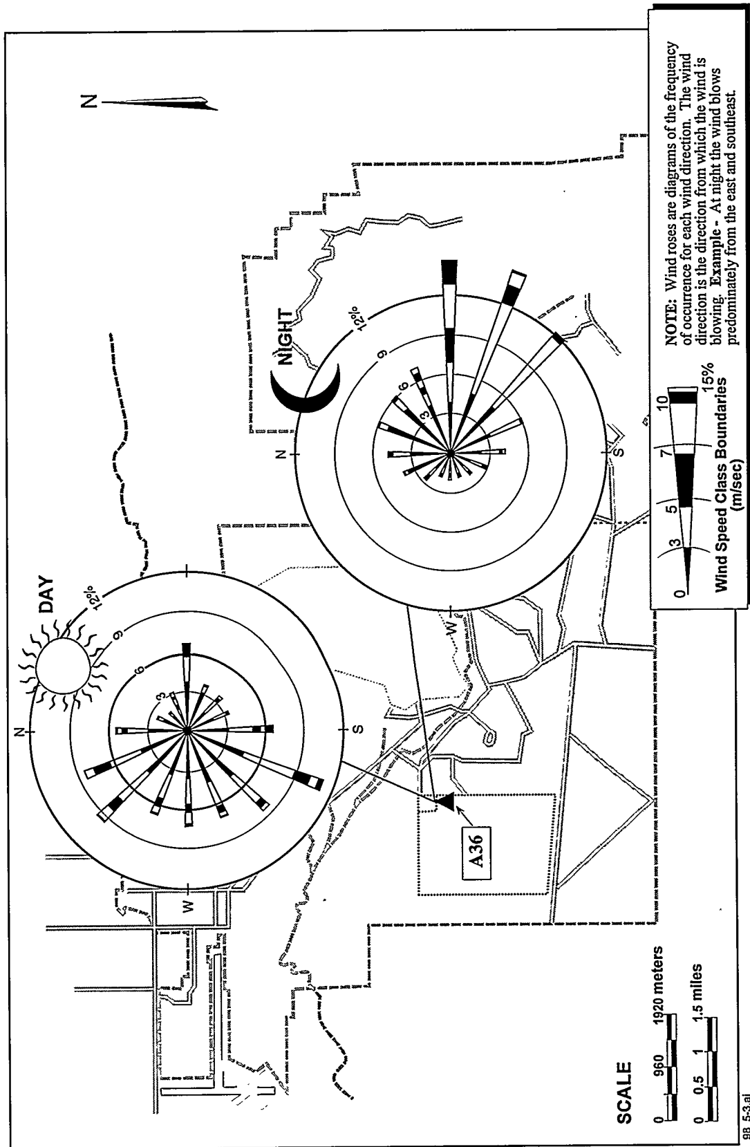
FIGURE 5-3. 1997 Annual Wind Roses for Daytime and Nighttime Wind Frequency at the A36 Tower
