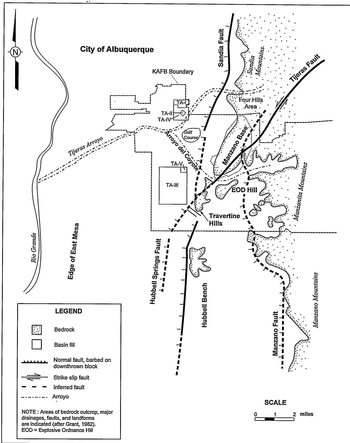
FIGURE 1-7. Generalized Geology in the Vicinity of SNL/NM and KAFB
