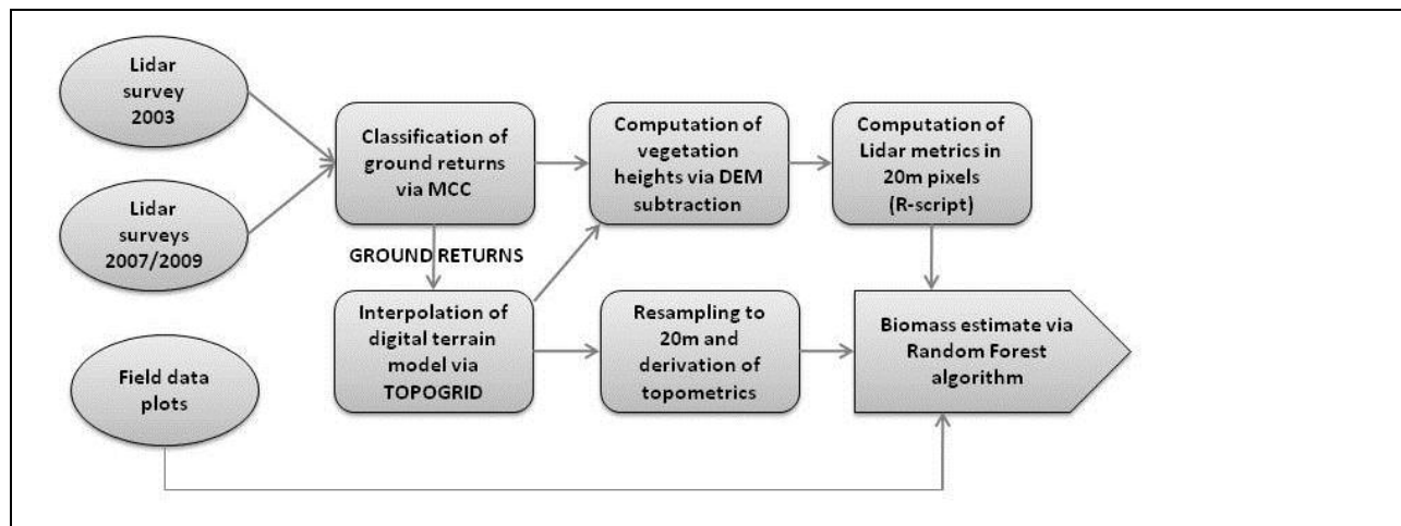
Figure 3: Procedure for deriving biomass estimates from remote sensing LiDAR data and field information. The LiDAR surveys from 2003 and 2007/2009 were processed separately to estimate above ground woody biomass followed by grid subtraction to obtain the change in biomass.
