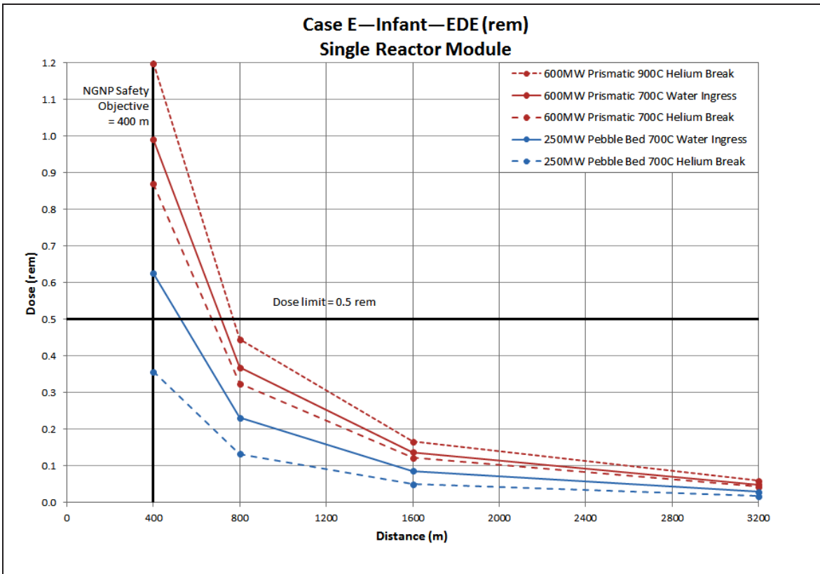
Figure 1. Case E, infant, EDE (rem), single reactor module.
