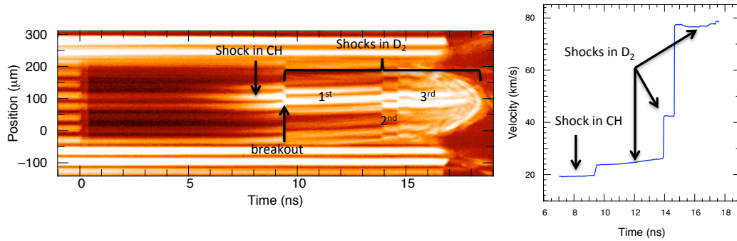
Fig. 3. Sample streak record and corresponding velocity profile. Breakout and merger events are identified.
