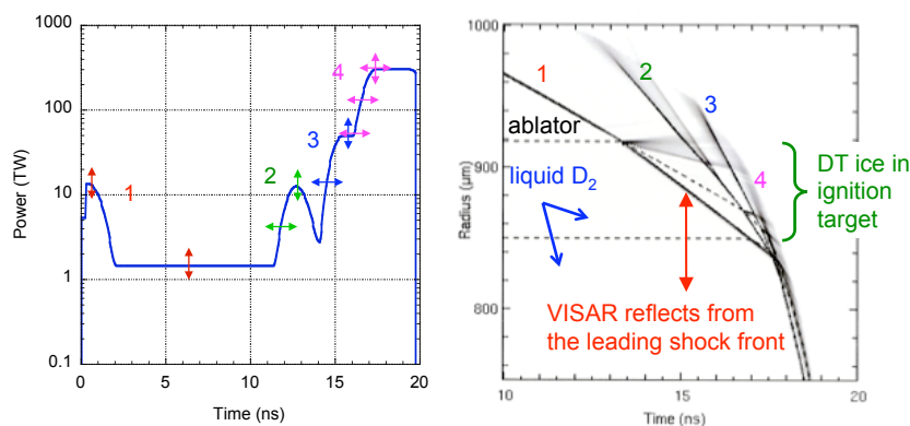
Fig. 1. Laser power history on the left; each segment of the pulse identified by the annotations launches a shock which propagates into the target as shown on the lagrangian radius versus time plot on the right.
