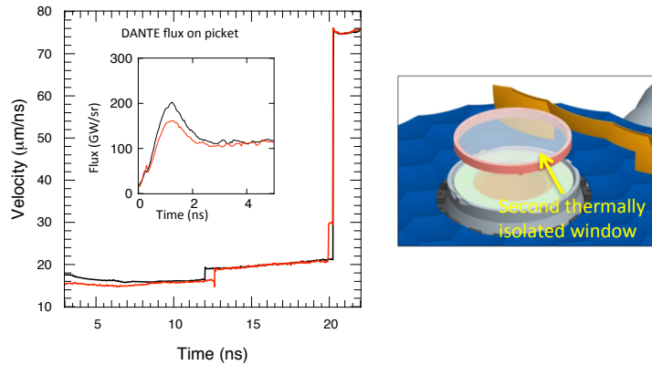
Fig. 4. Velocity profiles for targets incorporating LEH “storm windows” showing a high degree of reproducibility for two successive shots. A small reduction in the picket power of the second pulse produced a slightly later CH-D 2 breakout and a slightly earlier second shock merge time, in agreement with post-shot analysis.
