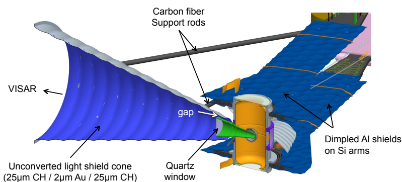
Fig. 2. Cut-away drawing of the target. The capsule and interior cone is filled with liquid deuterium.
