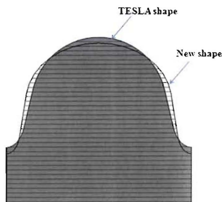
Figure 1: A comparison between TESLA shape and new "standard" design. The shapes have been scaled to the same cell length for comparison.
