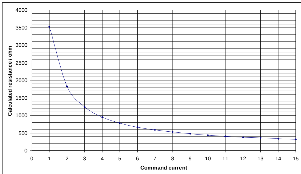
Figure 23 – COM port impedance.
