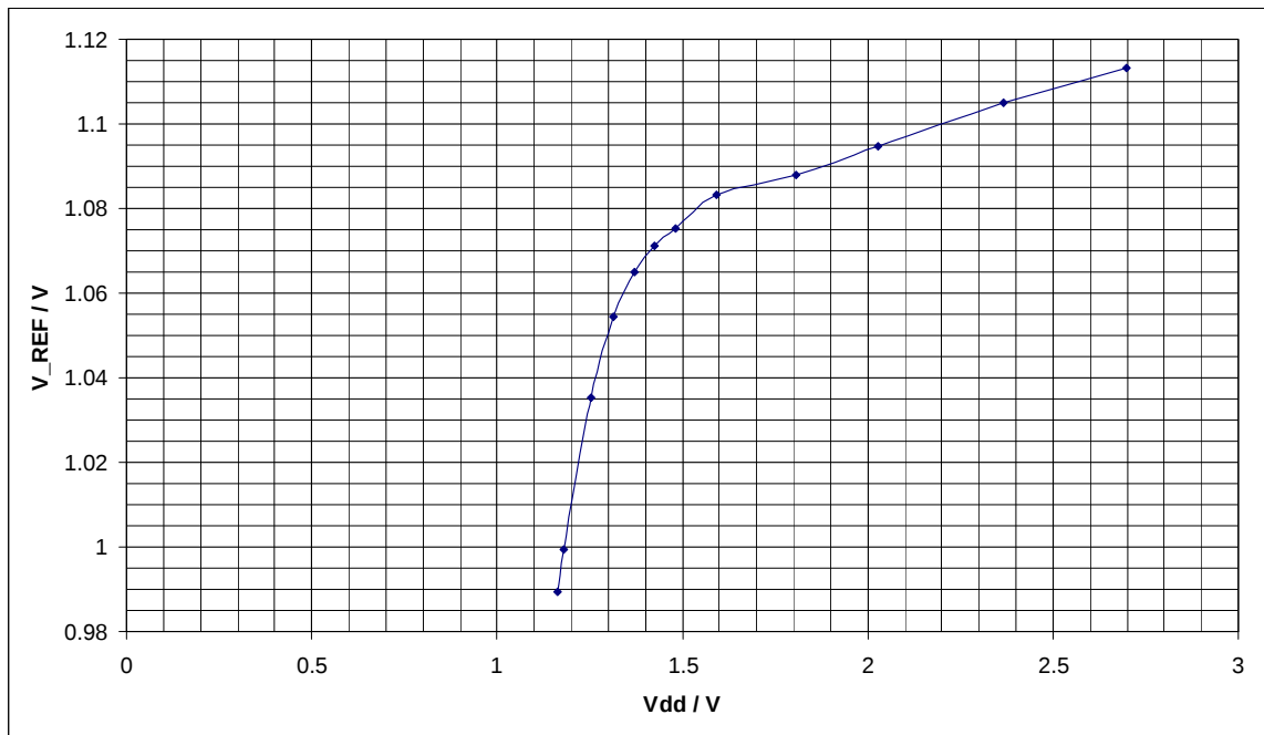
Figure 18 – V_REF open circuit – variation with VDD.
