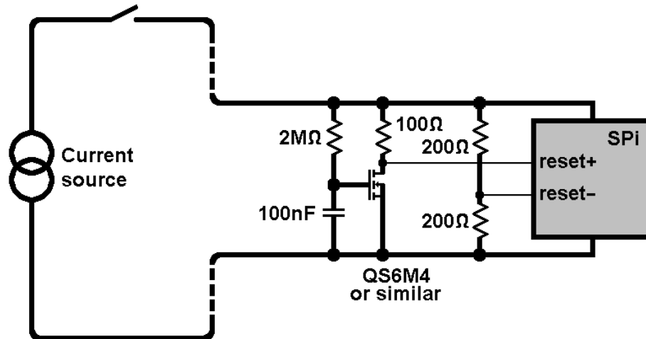
Figure 13 – Reset circuit
