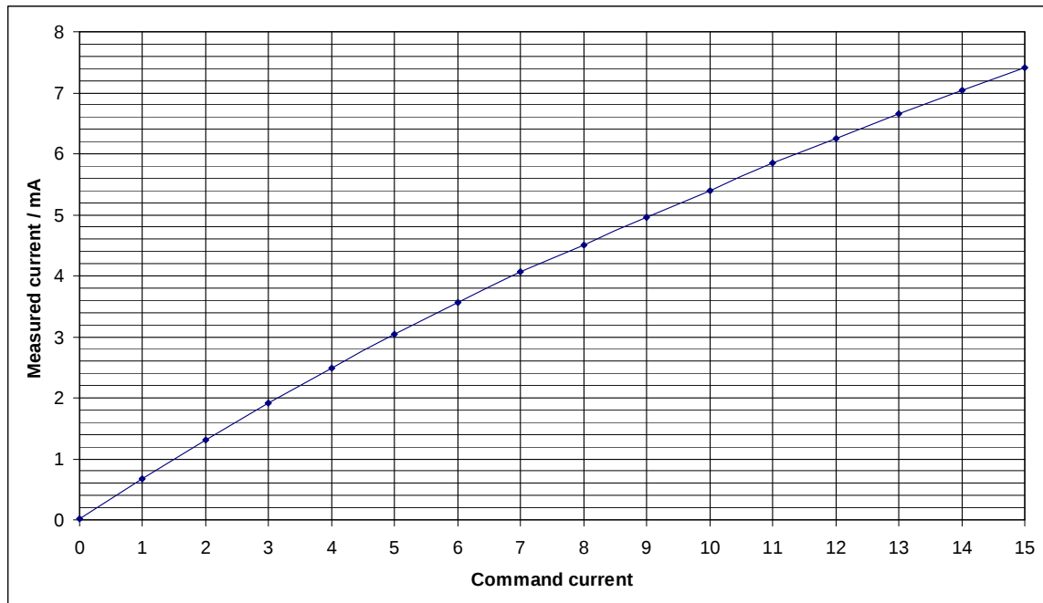
Figure 22 – COM port drive current.
