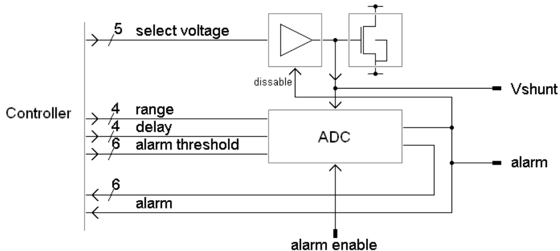
Figure 7 – Shunt regulator.
