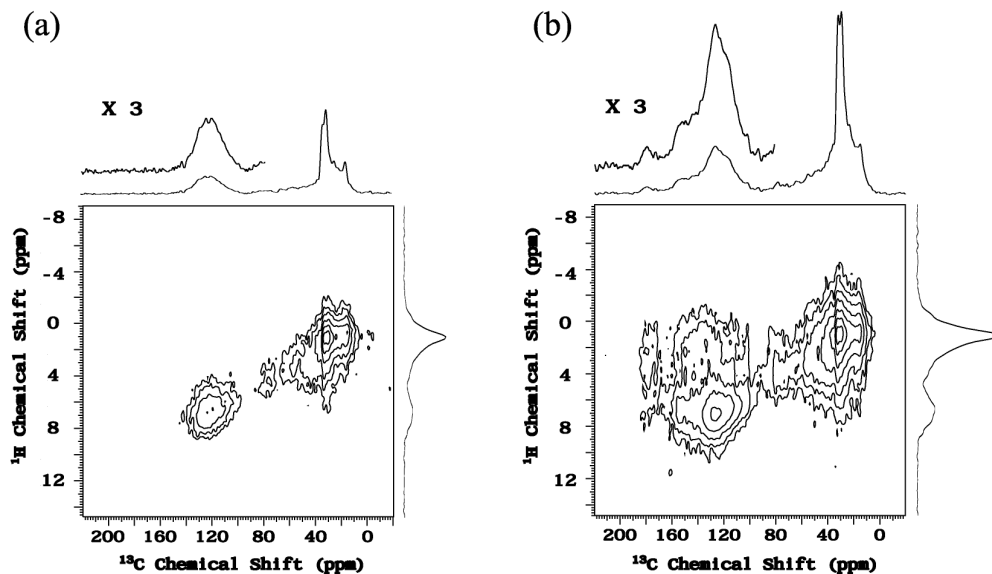
Fig. 3.6. 2D ^1\text{H}\{^{13}\text{C}\} HETCOR spectra of brown coal acquired using INEPT (a) and CP (b) transfers during mixing. The following RF magnetic fields were used: \nu_{RF}^H = 150 kHz during \pi/2 and PMLG5 _{\bar{m}} pulses, \nu_{RF}^H = 62 kHz during CP (tangent), \nu_{RF}^H = 11 kHz during SPINAL-64 decoupling in t_1 , \nu_{RF}^C = 104 kHz during CP, \pi/2 and \pi pulses, and \nu_{RF}^C = 11 kHz during SPINAL-64 decoupling in t_2 . Other experimental conditions were as follows: \nu_R = 41.667 kHz, \tau_{CP} = 1.5 ms, \tau_{RR} = 24 ms, \tau_1 = 0.84 ms, \tau_2 = 1.2 ms, \tau_{PMLG} = 0.75 \mu\text{s} , \tau_c = 15 \mu\text{s} , \tau_{RD} = 0.8 s, NS = 176, \Delta t_1 = 24 \mu\text{s} (100 rows), and AT = 8.7 h.
