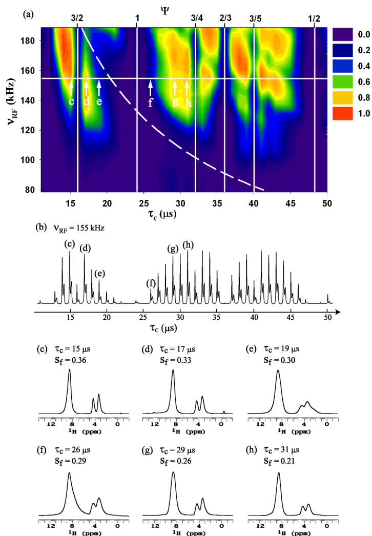
Fig. 4.3. (a) The integrated intensity of spin-echo in glycine as a function of \tau_c and \nu_{\text{RF}} , measured under \text{PMLG}5_{mm}^{\bar{x}} decoupling, with \tau \cong 2 \text{ ms} and \tau_R = 24 \mu\text{s} ( \nu_R = 41.67 \text{ kHz} ). The plot consists of 1920 points representing integrated intensity of the entire echo signal measured for 40 values of \tau_c and 48 values of \nu_{\text{RF}} . The dashed curve corresponds to the LG condition \nu_{\text{RF},\text{LG}} and the vertical lines to \psi = 3/2, 1, 3/4, 2/3, 3/5 and 1/2 . The measurement time was approximately 4 hours. (b) A series of 1D spectra measured for \nu_{\text{RF}} = 155 \text{ kHz} (horizontal line in (a)). (c-h) The projections of 2D ^1\text{H} - ^1\text{H} correlation spectra obtained under decoupling conditions marked in Figure 4.3a and b. Other experimental conditions were as given in the caption to Figure 4.2.
