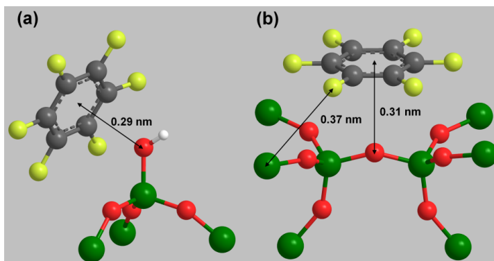
Fig. 5.6. The optimized geometries of (a) C 6 F 6 -silanol and (b) C 6 F 6 -siloxane models. Silicon atoms are green, oxygen atoms are red, carbon atoms are gray, fluorine atoms are yellow, and hydrogen atom is white. Silanol hydrogen is the only one shown.
