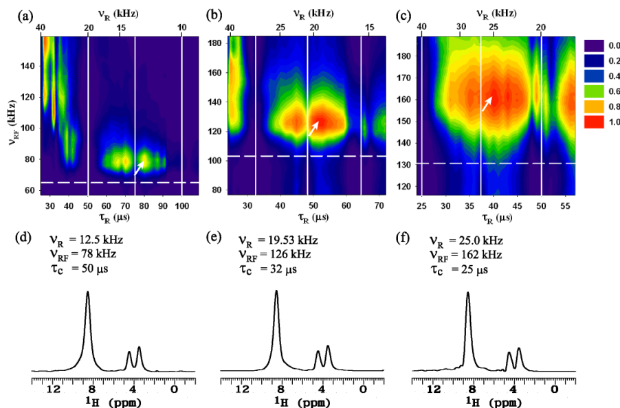
Fig. 4.2. The integrated intensity of spin-echo in glycine as a function of \tau_R and \nu_{RF} , measured under PMLG 5_{mm}^{xx} decoupling, with \tau \cong 2 ms, the carrier frequency set at 4 ppm from TMS, and \tau_c = 50 \mu s (a), 32 \mu s (b) and 25 \mu s (c). The experiments were performed at 14.1 T on a Varian NMR System 600 MHz spectrometer, equipped with 1.6 mm triple-resonance MAS probe. The plots comprise 2000 points representing integrated intensity of the entire echo signal measured for 40 values of \tau_R and 50 values of \nu_{RF} . Each signal consisted of 4 scans acquired using acquisition delay of 2s. Total measurement time was approximately 3 days per plot. The contours were normalized relative to the highest intensity observed in each plot. The vertical lines correspond from left to right to \psi = 1 , 3/2 and 2 . The dashed line represents the LG value \nu_{RF,LG} = 4\sqrt{2/3}\nu_c . (d-f) The projections of indirect dimensions of 2D ^1\text{H} - ^1\text{H} correlation spectra measured using the \nu_R and \nu_{RF} values indicated by arrows in (a-c). Each spectrum was acquired in 160 rows, 8 scan per row, with t_1 increment of \sim 100 \mu s, and the total experiment time was 1.5 hrs.
