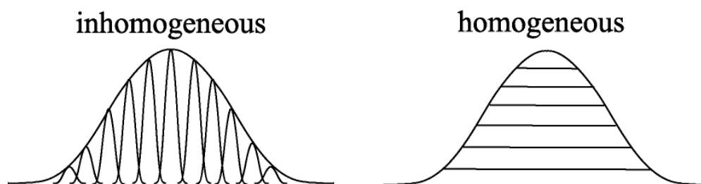
Figure 1.4. Visualization of inhomogeneous and homogeneous line broadening.
