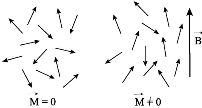
Figure 1.1. The semi-classical model of the net magnetization, \vec{M} . In the absence of the external magnetic field, \vec{M} = 0 , due to the orientations of individually magnetic moments (indicated by small vectors) being randomly distributed. With the field \vec{B} applied, the non-zero net magnetization appears along the \vec{B} direction.
