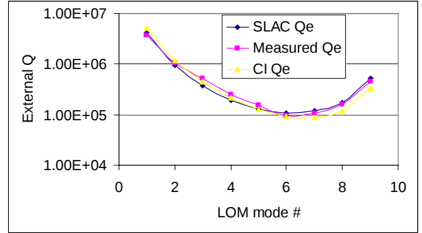
Figure 2. Comparison of the LOM coupler external Q factors for the lower order mode, between, measurements and simulations in Microwave Studio and Omega-3P.
