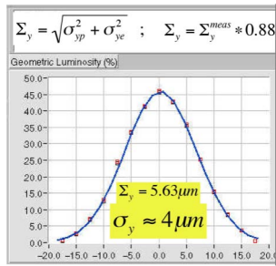
Figure 2: Vertical beam-beam luminosity scan.
