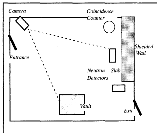
Figure 2: VTRAP Test-bed Configuration
