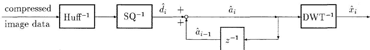
Figure 5: Predictive wavelet transform image decoder.
