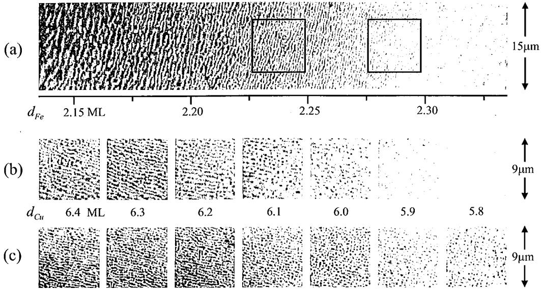
FIG. 1. (a) PEEM image of the Fe magnetic domains in Fe/Ni(5 ML)/Cu(6.40 ML)/Ni(20 ML)/Cu(001). d_{\text{Cu}}^0 = 6.40 ML corresponds to a zero interlayer coupling between the (Fe/Ni) film and the Ni(20 ML) film. The stripe domain width decreases with increasing the Fe film thickness toward the SRT point at d_{\text{Fe}}^0 = 2.32 ML, above which the Fe film has an in-plane magnetization. [(b) and (c)] PEEM images of the Fe domains at (b) d_{\text{Fe}} = 2.24 and (c) 2.29 ML as a function of the Cu film thickness. The position of the first images of (b) and (c) are marked by the two boxes in figure (a) except the 90^\circ rotation for a clearer view of the domain pattern evolution. Changing Cu thickness away from the zero coupling point of d_{\text{Cu}}^0 = 6.40 ML is equivalent to applying a virtual perpendicular magnetic field to the (Fe/Ni) film. The (Fe/Ni) magnetic stripe phase evolves into a bubble phase before being saturated.
