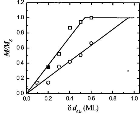
FIG. 2. (Color online) The normalized magnetization M/M_s determined from PEEM images as a function of \delta d_{\text{Cu}} = |d_{\text{Cu}} - d_{\text{Cu}}^0| which simulates the strength of the perpendicular virtual magnetic field applied to the (Fe/Ni) film. Data from d_{\text{Fe}} = 2.24 ML [Fig. 1(b)] are represented by square symbols; data from d_{\text{Fe}} = 2.29 ML [Fig. 1(c)] are represented by circular symbols. Solid symbols represent the stripe phase and open symbols represent the bubble phase. The solid lines are guides for the eyes.
