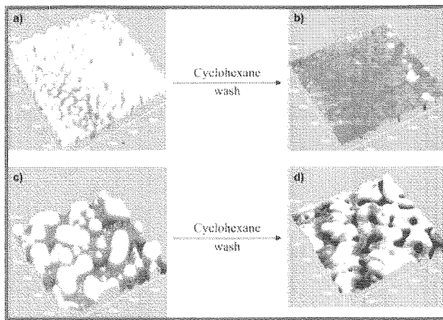
Figure 7. AFM height mode images of 40:60 PS:PLA thin films cast from a 0.7 wt % solution which were (a) as-cast, (b) as-cast, followed by wash with cyclohexane; (c) annealed 1 h at 70 °C, (d) annealed, followed by wash with cyclohexane. All images are 10 \mu\text{m} \times 10 \mu\text{m} .
