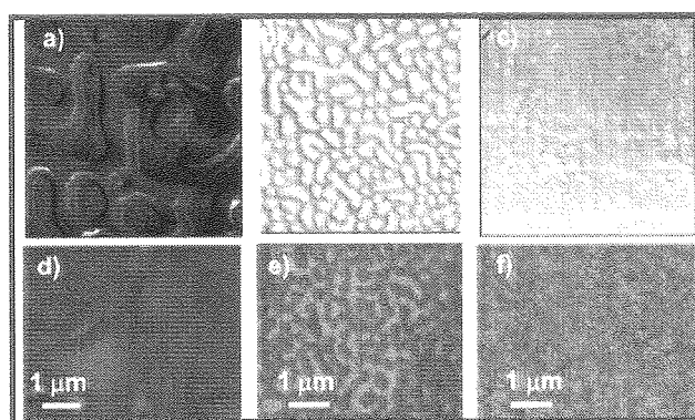
Figure 5. (upper row) AFM phase mode images of 40:60 PS:PLA films spun-cast from dichloromethane solutions with total polymer loading of (a) 1.0, (b) 0.7, and (c) 0.4 wt %. All AFM images are 10 \mu\text{m} \times 10 \mu\text{m} . (lower row) X-PEEM color-coded composite maps (nonrescaled) of 40:60 PS:PLA films (d) 1.0, (e) 0.7, and (f) 0.4 wt %. PS is coded red, and PLA is coded green.
