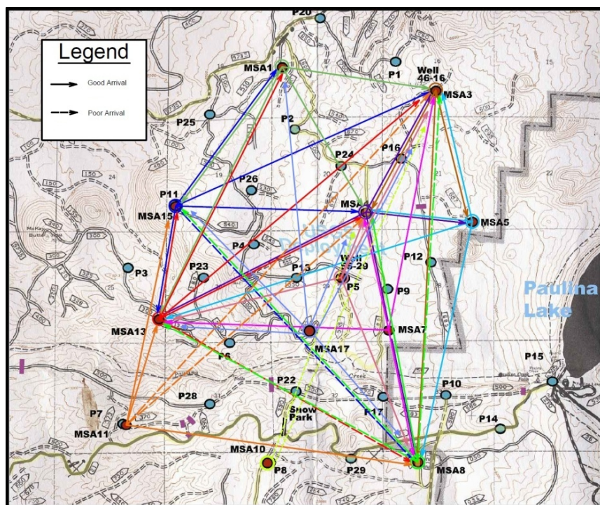
Figure 1. Calibration shot arrivals. Stations with colored circles represent shot points, and the associated colored arrows show which stations recorded the arrivals from that calibration shot.
