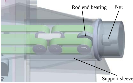
Fig. 3. Structure of the cold mass support warm end
