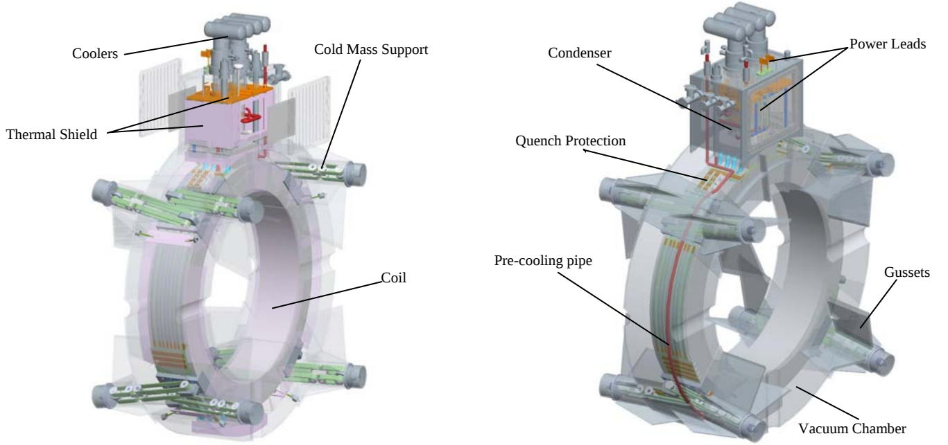
Fig. 1. 3D model of MICE coupling magnet
