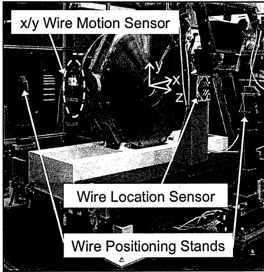
Figure 1: NDCX-II magnet measurement facility including wire stands on motion stages, a wire displacement sensor, and laser micrometers for determining the wire location.
