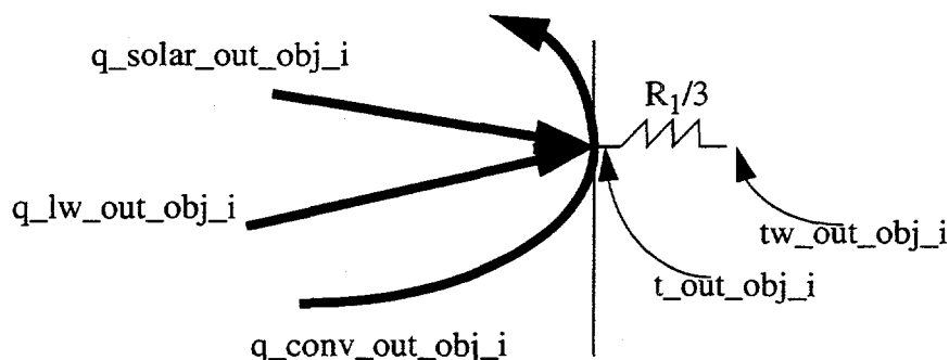
Figure 44. The heat flux balance at the exterior surface node
