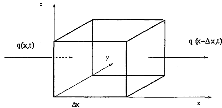
Figure 39. Volume element for conduction heat flow
