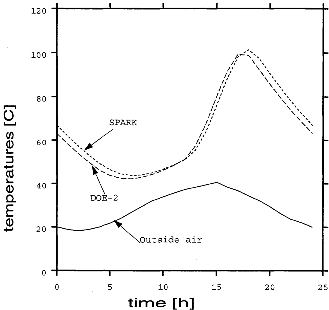
Figure 18. Indoor air temperature: structure 2 (wood - insulation - gypsumboard)
