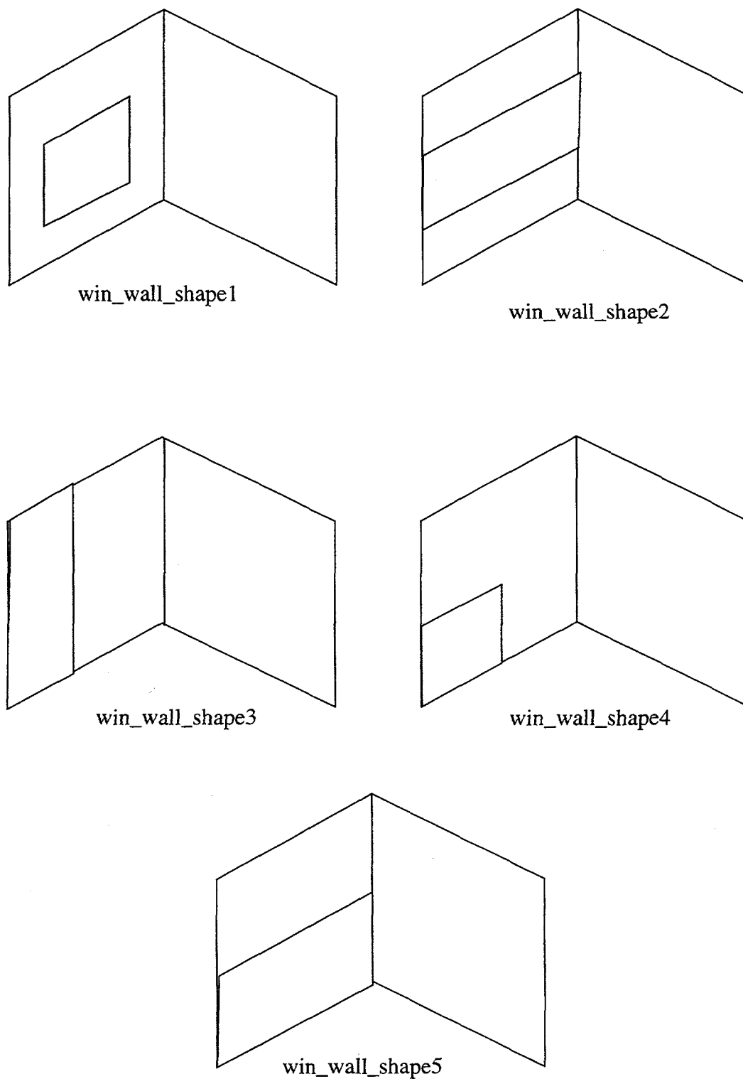
Figure 65. The relative positioning of adjacent window and wall surfaces at an angle of 90^\circ .
