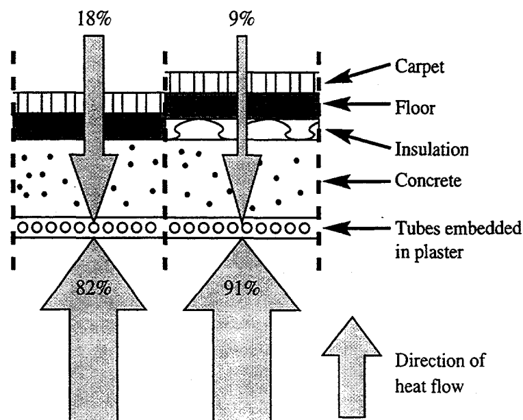
Figure 12. Heat transfer for ceiling with cooling grid
