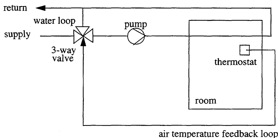
Figure 59. Hybrid control strategy
