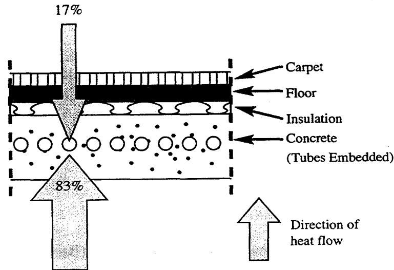
Figure 14. Heat transfer for slab cooling
