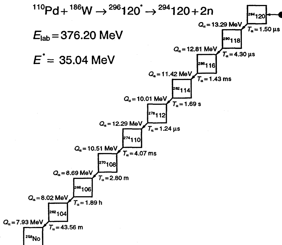
Figure 7. Calculated Q -values for \alpha decay and corresponding calculated half-lives for the decay chain starting at ^{294}120 .
