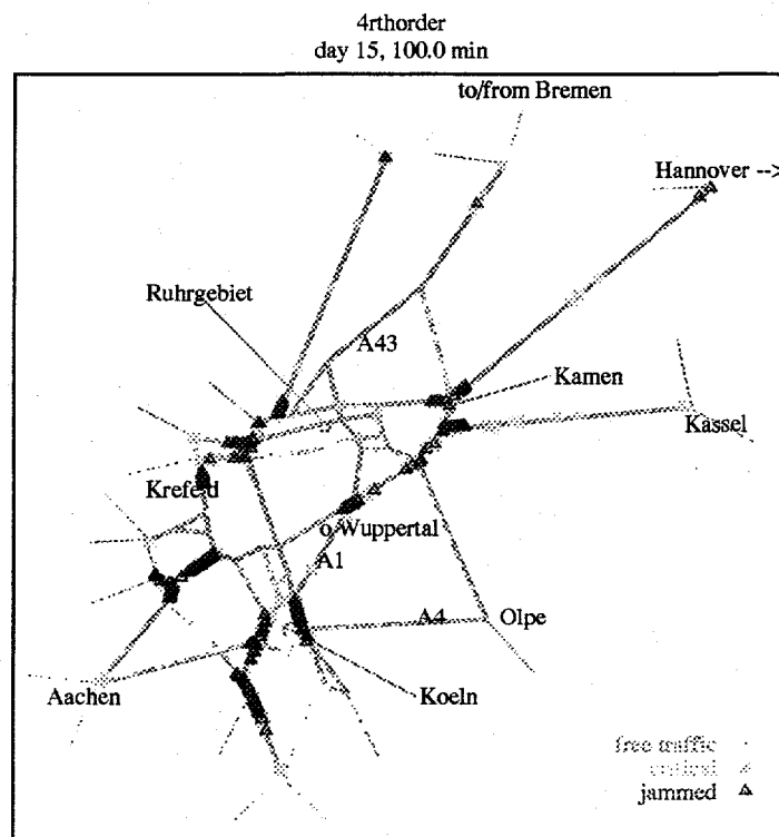
Figure 4: Top : Situation at the "first day" after 6000 iterations (100 minutes), when trips through the network are chosen with a fourth order preference for long trips, and when all drivers follow the geometrically shortest path. — Bottom : Situation at "day 15" after 6000 iterations (100 minutes), for the same initial conditions as for the top figure, but where drivers have "learned".
