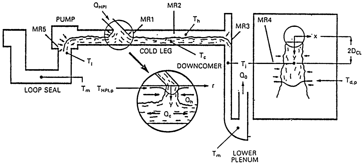
Figure 2. Conceptual Definition of Flow Regime and Regional Mixing Model
