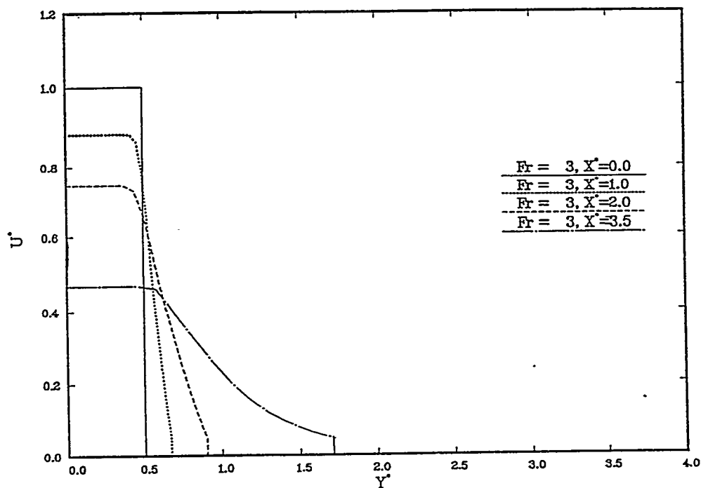
Figure 8. Calculated Results of Velocity Profiles for a Negatively Buoyant Planar Jet ( Fr = 3 )
