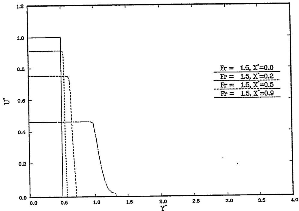
Figure 6. Calculated Results of Velocity Profiles for a Negatively Buoyant Planar Jet ( Fr = 1.5 )
