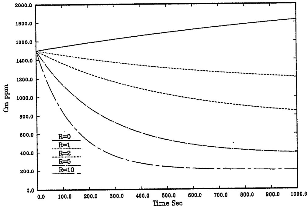
Figure 3. Dilution Transient Under Stratified and Recirculating Flow Regime
