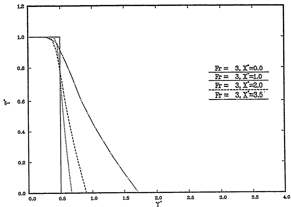
Figure 7. Calculated Results of Temperature (or Concentration) Profiles for a Negatively Buoyant Planar Jet ( Fr = 3 )
