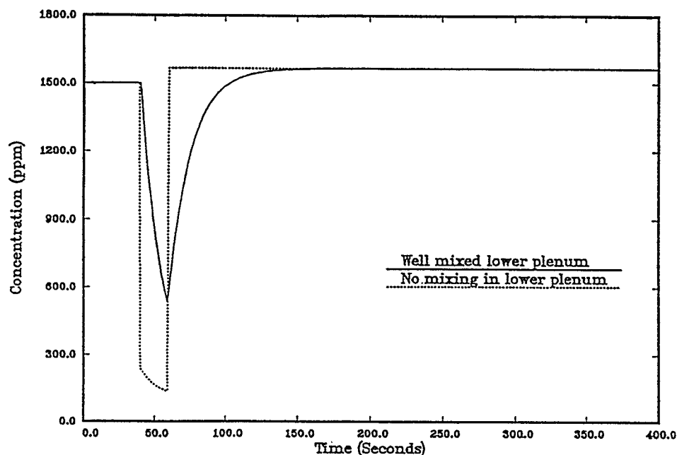
Figure 10. Transient Boron Concentration Entering the Core
