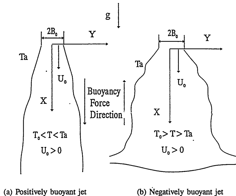
Figure 4. Schematic of a Positively and a Negatively Buoyant Jet
