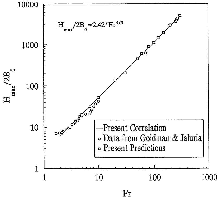
Figure 9. Comparison of Predicted Maximum Penetration Distance of Negatively Buoyant Vertical Planar Jets with Experimental Data
