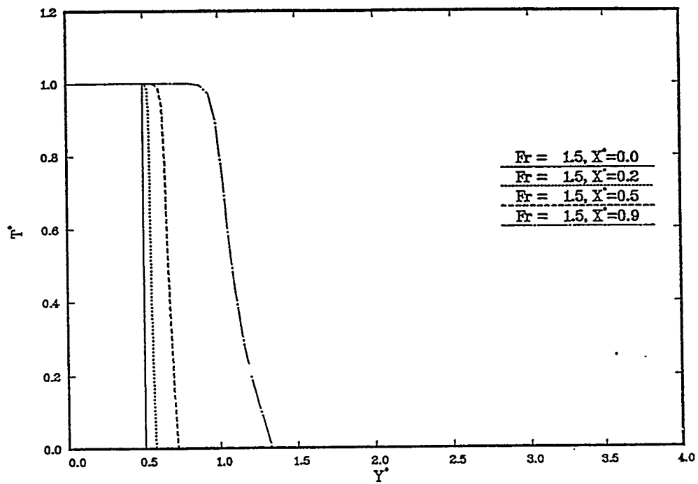
Figure 5. Calculated Results of Temperature (or Concentration) Profiles for a Negatively Buoyant Planar Jet ( Fr = 1.5 )
