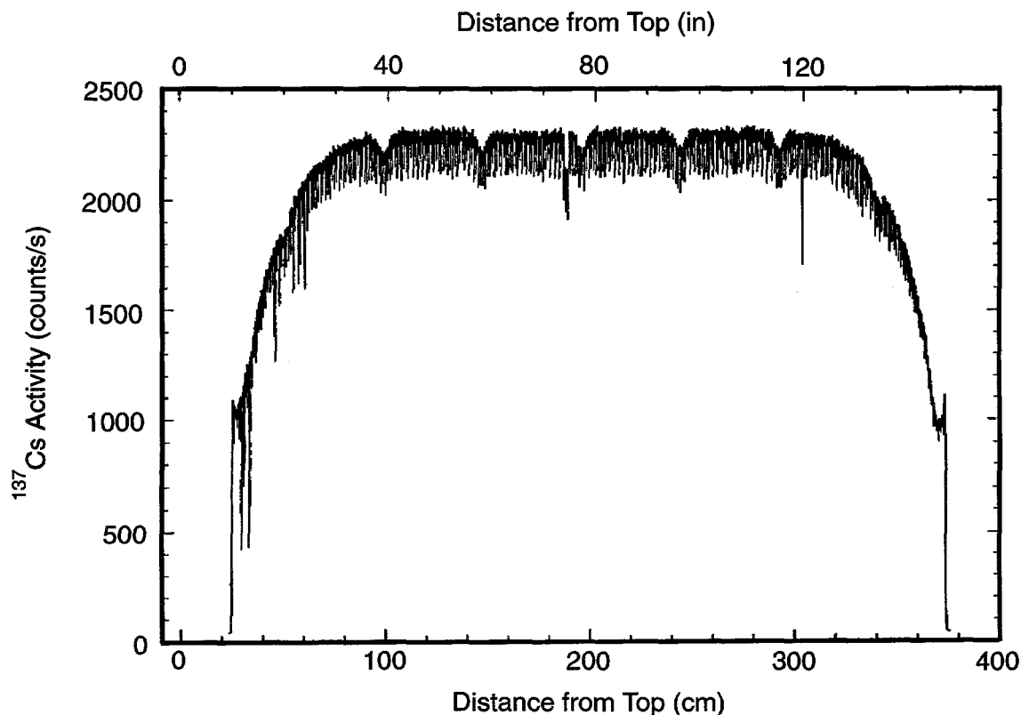
Figure 1. Axial gamma-ray scan for ^{137}\text{Cs} activity in a fuel rod from ATM-104 (Figure B.7. from [1]).
