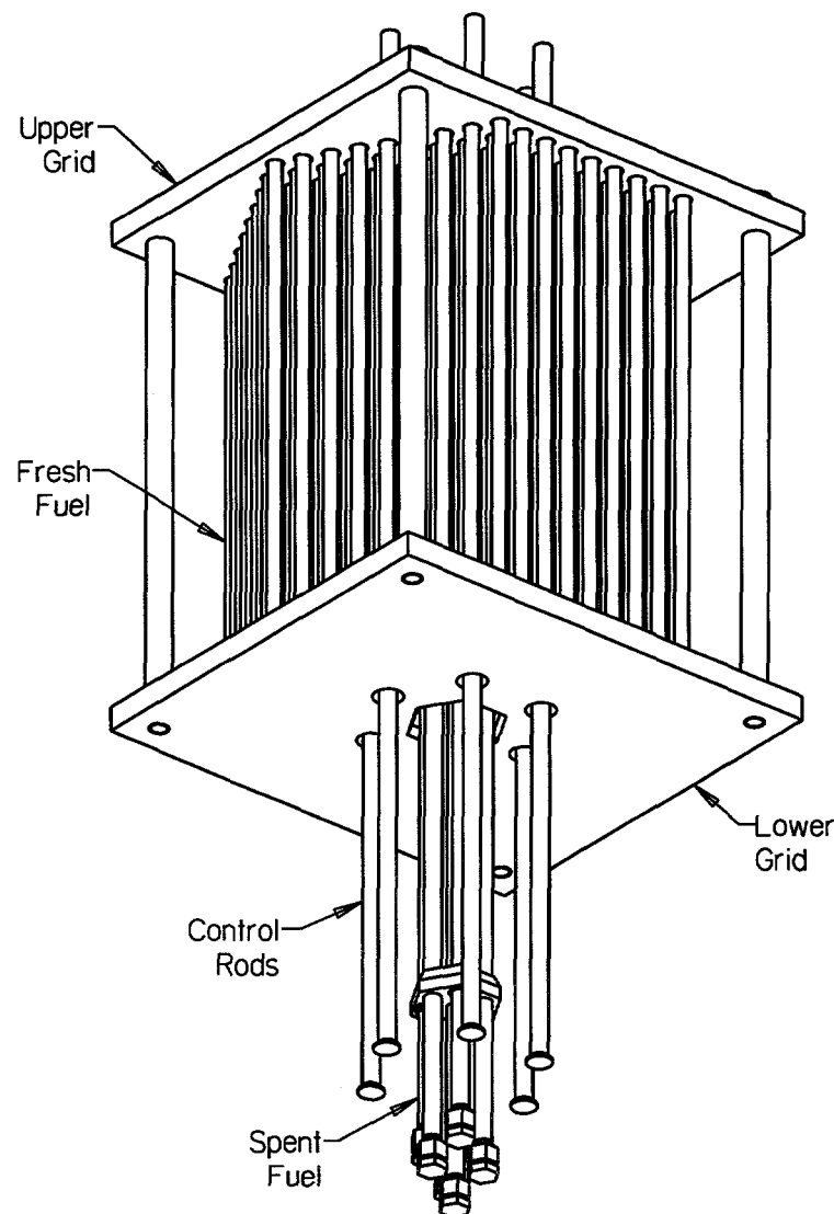
Figure 3. View of the SFSX critical assembly from below showing the spent fuel bundle.
