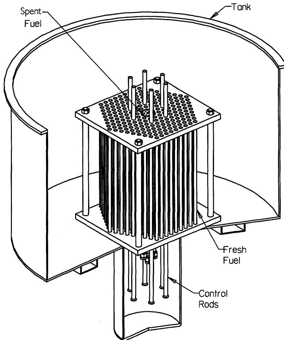
Figure 2. Overall view of the SFSX critical assembly.
