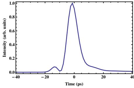
Figure 4: ILS pulse trace reconstructed from frequency resolved optical gating (FROG) pulse measurement showing 8.3 ps FWHM pulse length.
