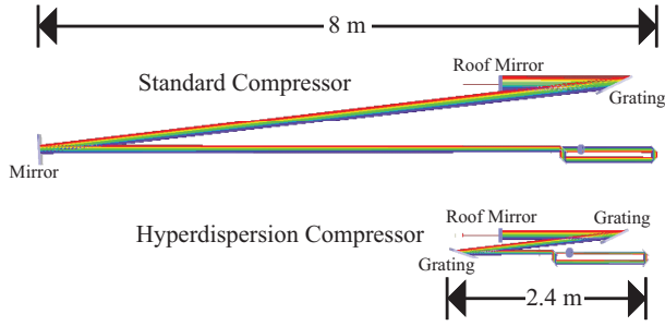
Figure 3: Comparison of the size of a standard (top) and hyperdispersion (bottom) compressor with a dispersion of 6650 ps/nm.
