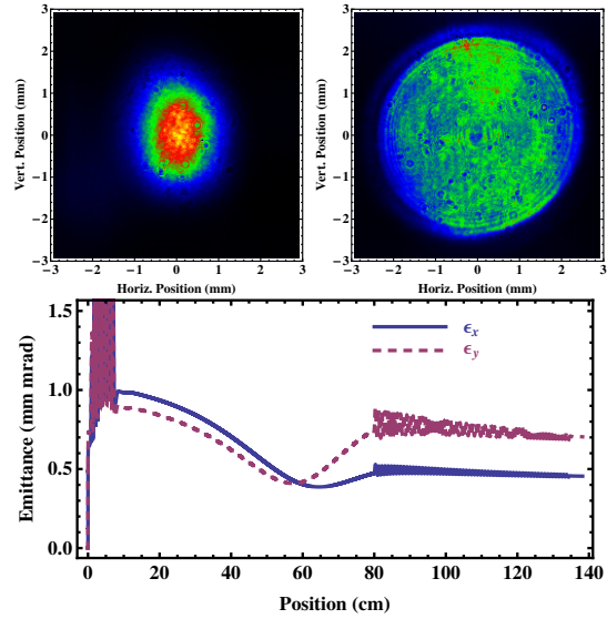
Figure 2: Top: Profiles before and after refractive beam shaper. Left: before, Right: after. Bottom: Simulated emittance growth of electron beam through X-band gun and first accelerating section with starting distribution shown above
