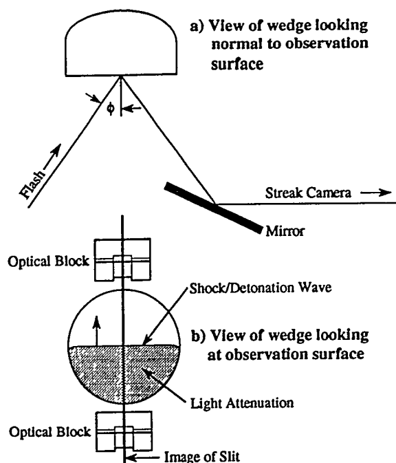
FIGURE 3. Optical configuration.
