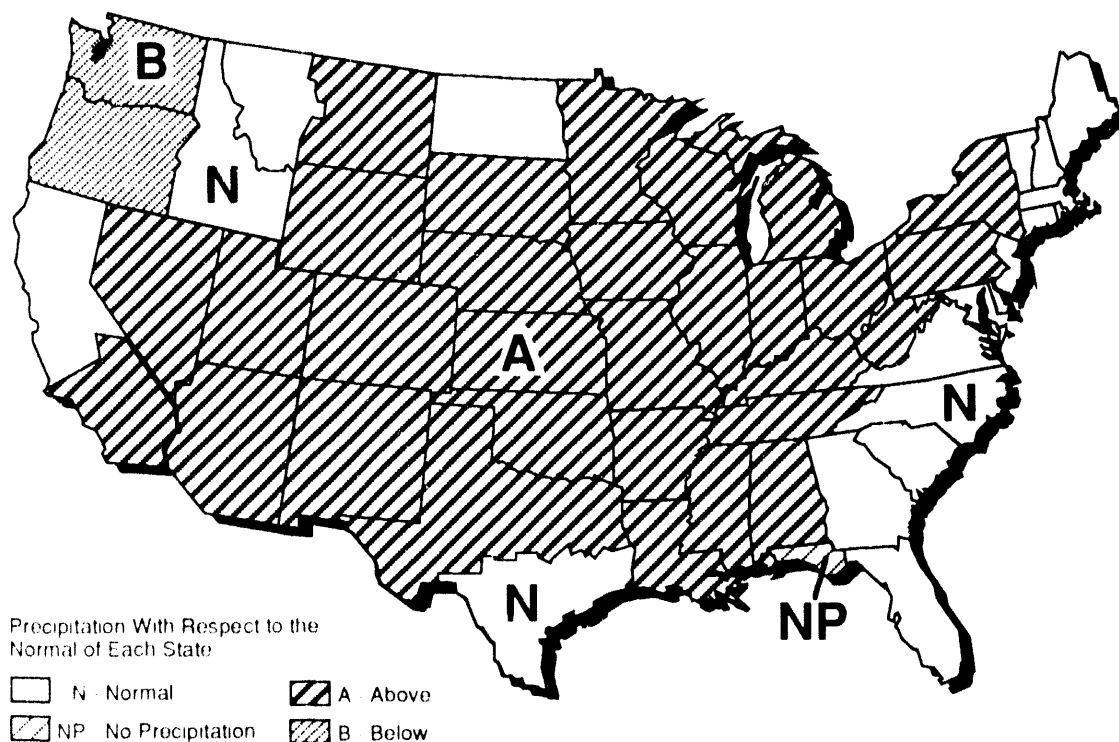
Figure 35. 6 - 10 Day Precipitation Outlook for November 23 Through November 27, 1993
