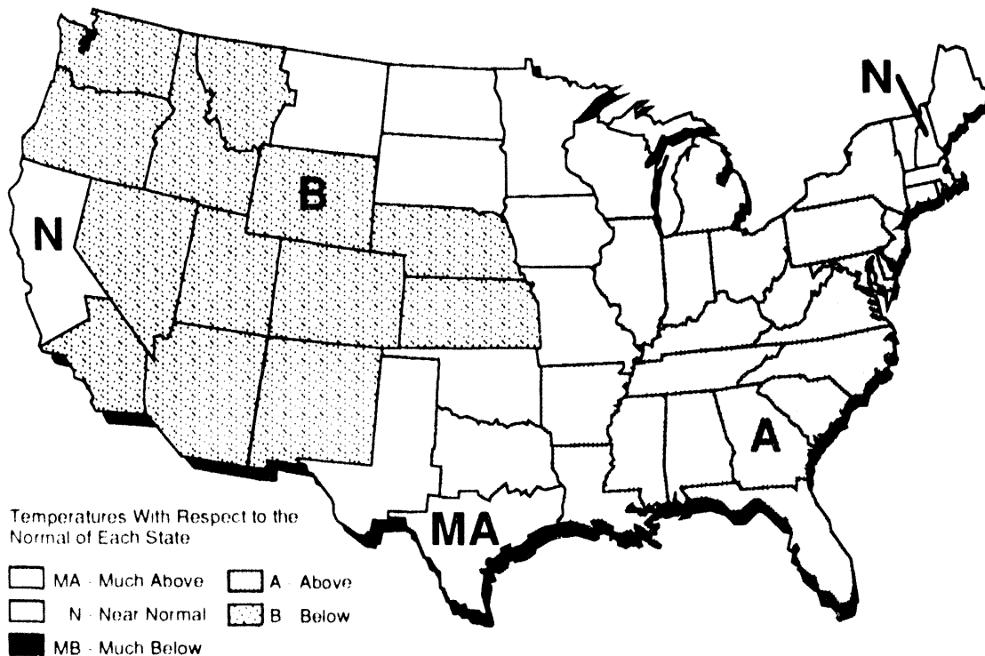
Figure 34. 6 - 10 Day Temperature Outlook for November 23 Through November 27, 1993
